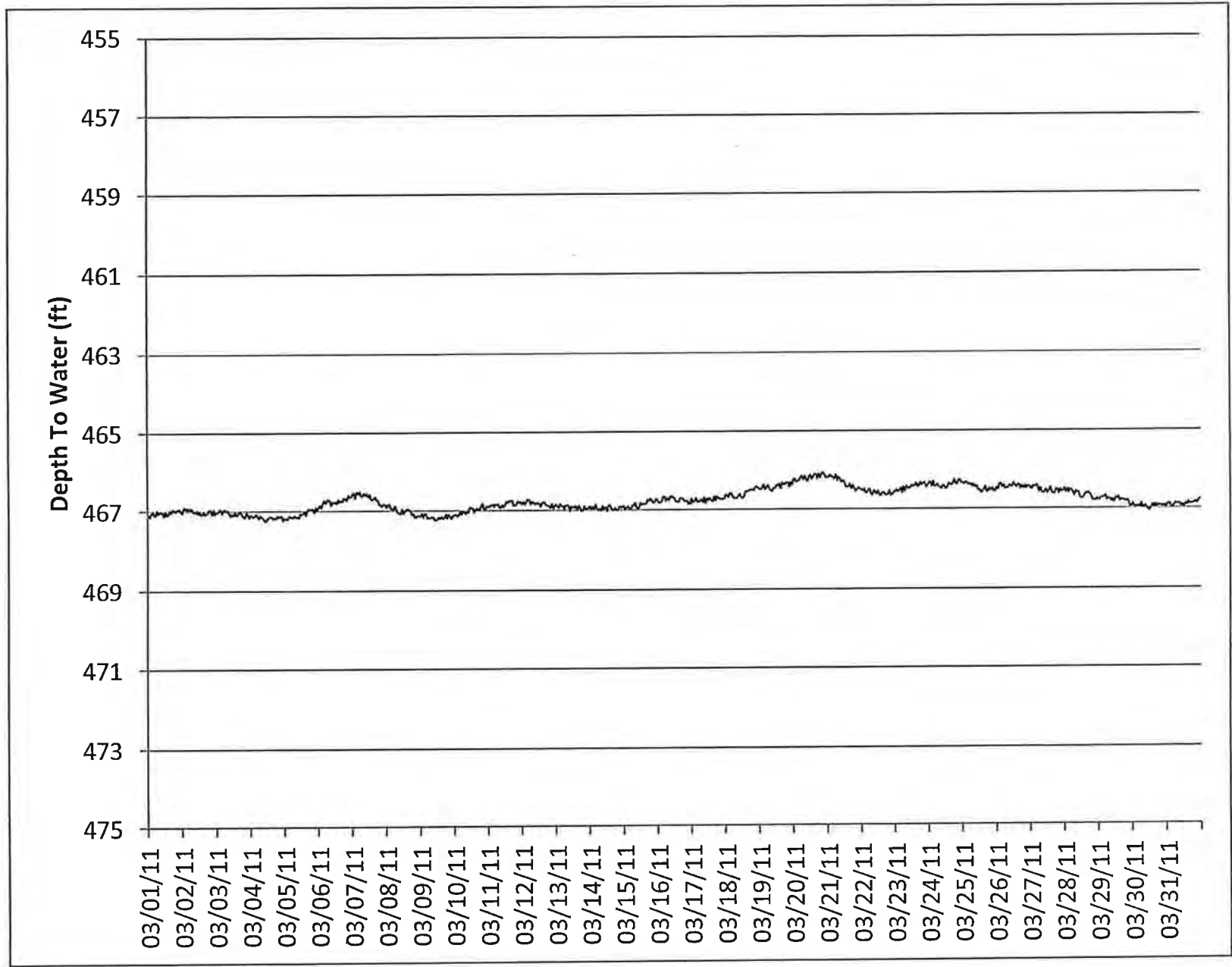
WATER LEVEL HYDROGRAPH FOR MW-30M
