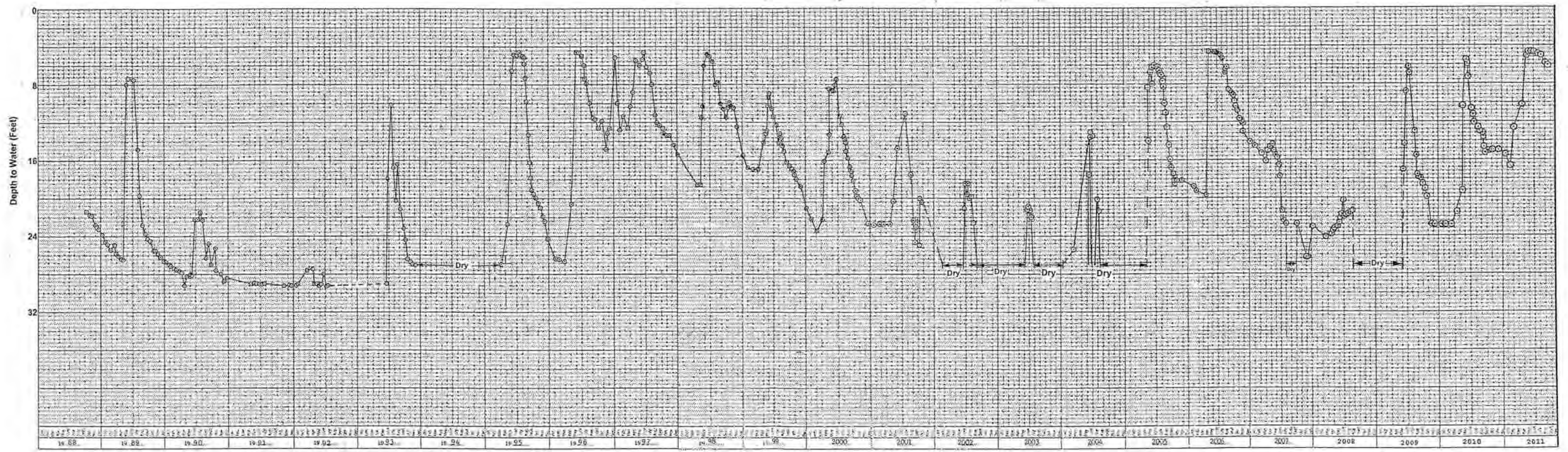
WATER-LEVEL HYDROGRAPH FOR WELL NO. 12M
