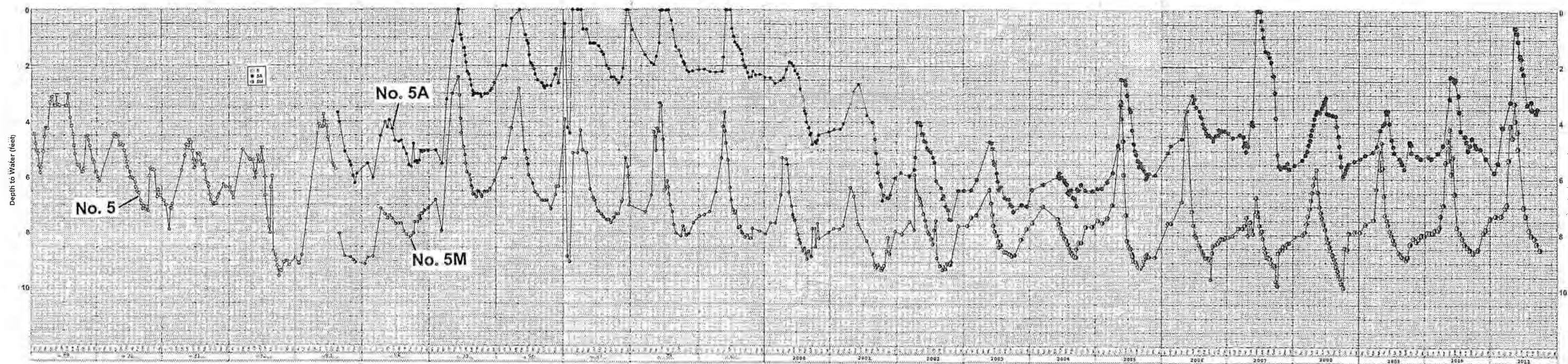
WATER-LEVEL HYDROGRAPH FOR WELL NO. 5, NO. 5A, AND NO. 5M
