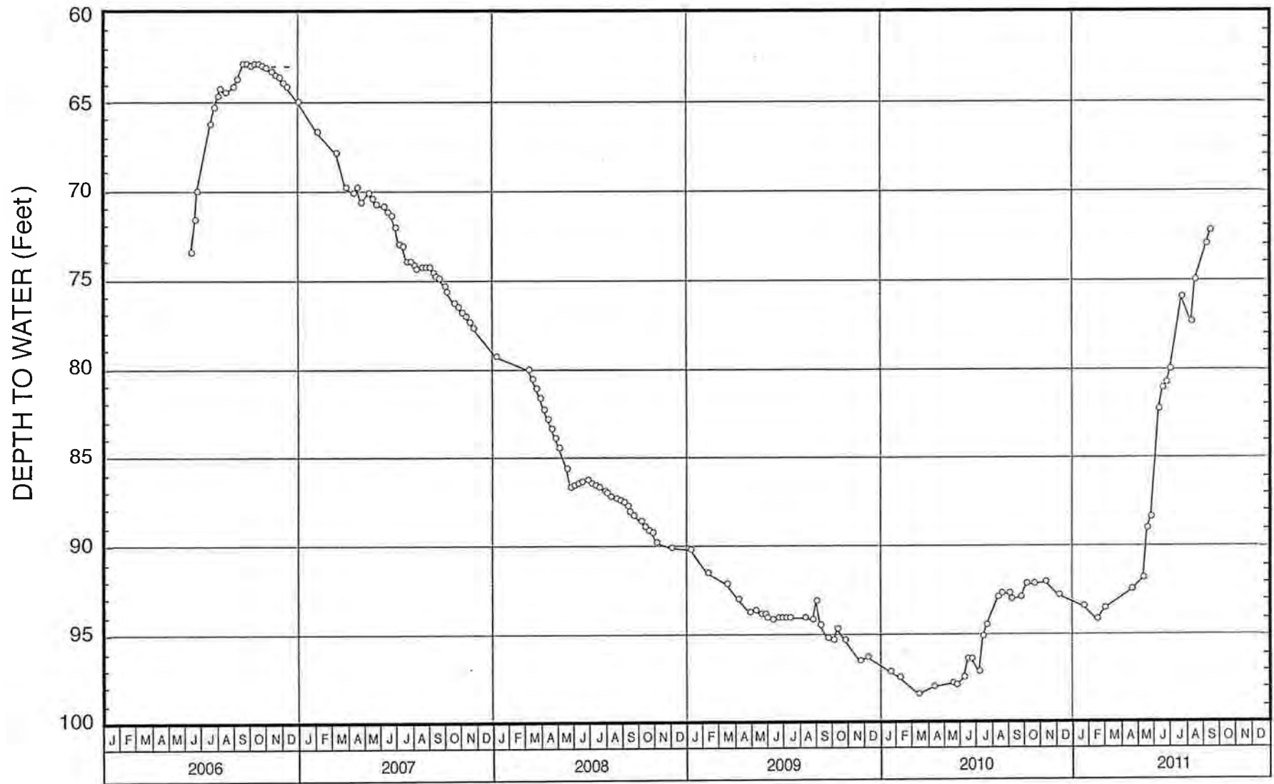
WATER-LEVEL HYDROGRAPH FOR WELL NO. 29
