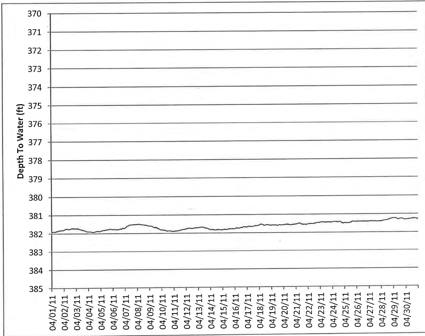
WATER LEVEL HYDROGRAPH FOR MW-24M
