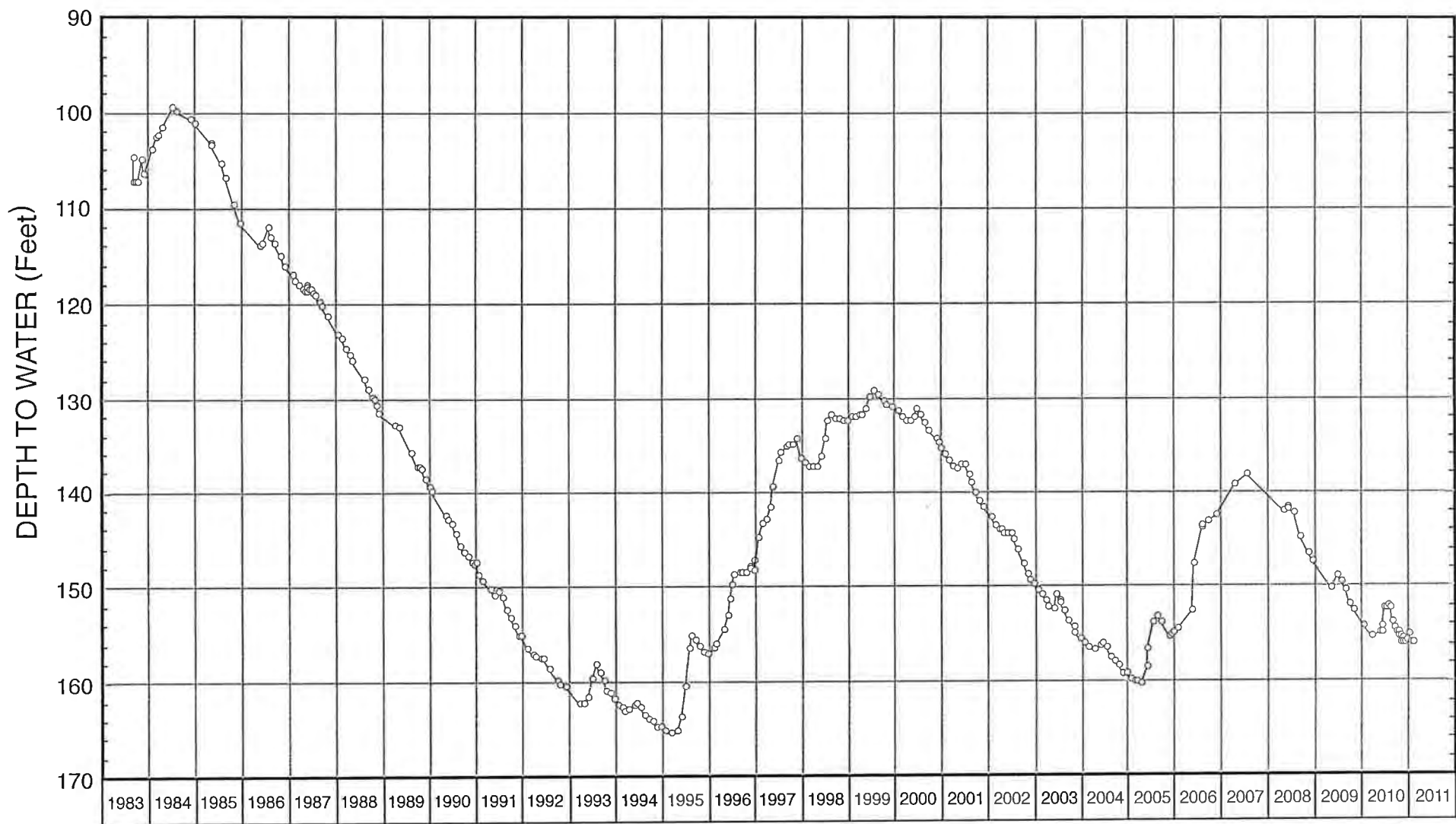
FIGURE 13 - WATER-LEVEL HYDROGRAPH FOR SC-2
