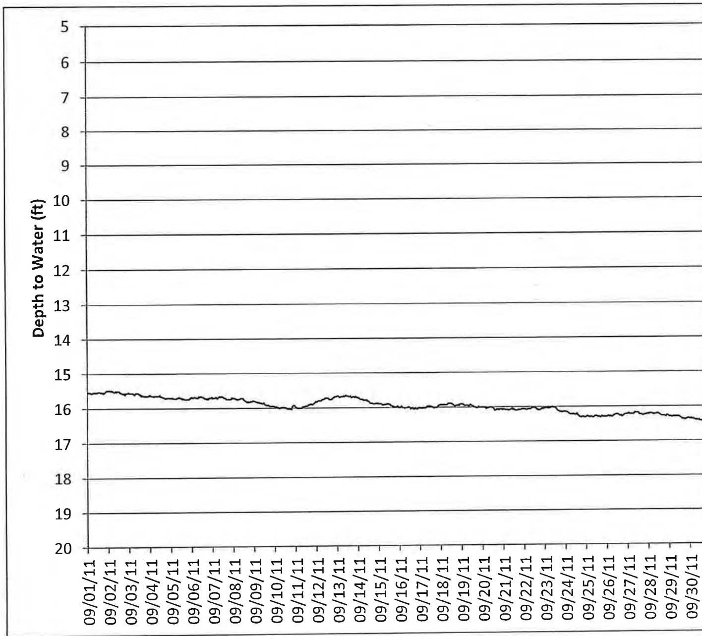
WATER LEVEL HYDROGRAPH FOR MW-23M
