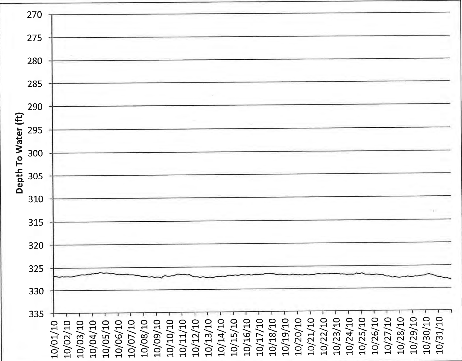
WATER LEVEL HYDROGRAPH FOR MW-14M
