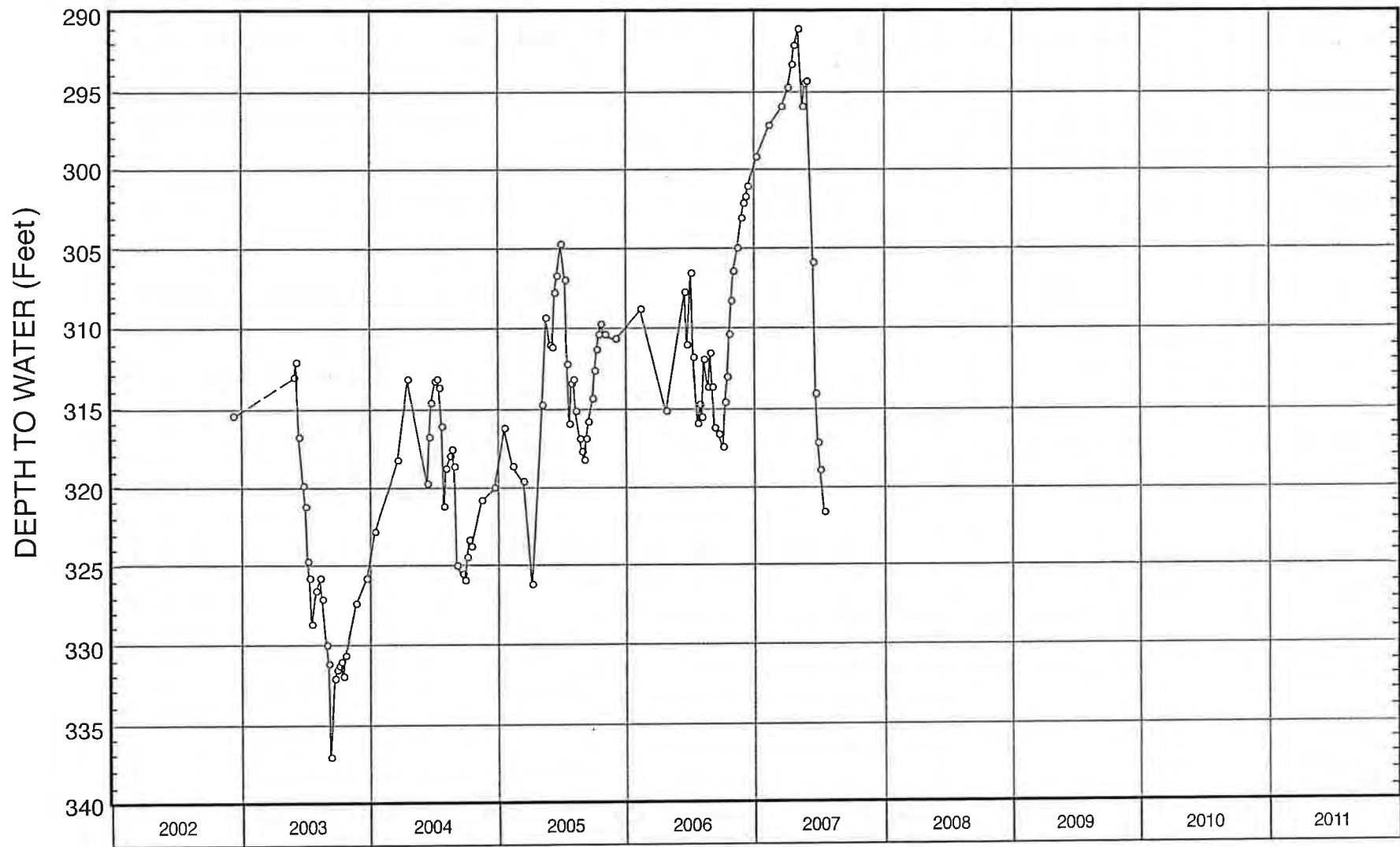
WATER-LEVEL HYDROGRAPH FOR WELL NO. 25
