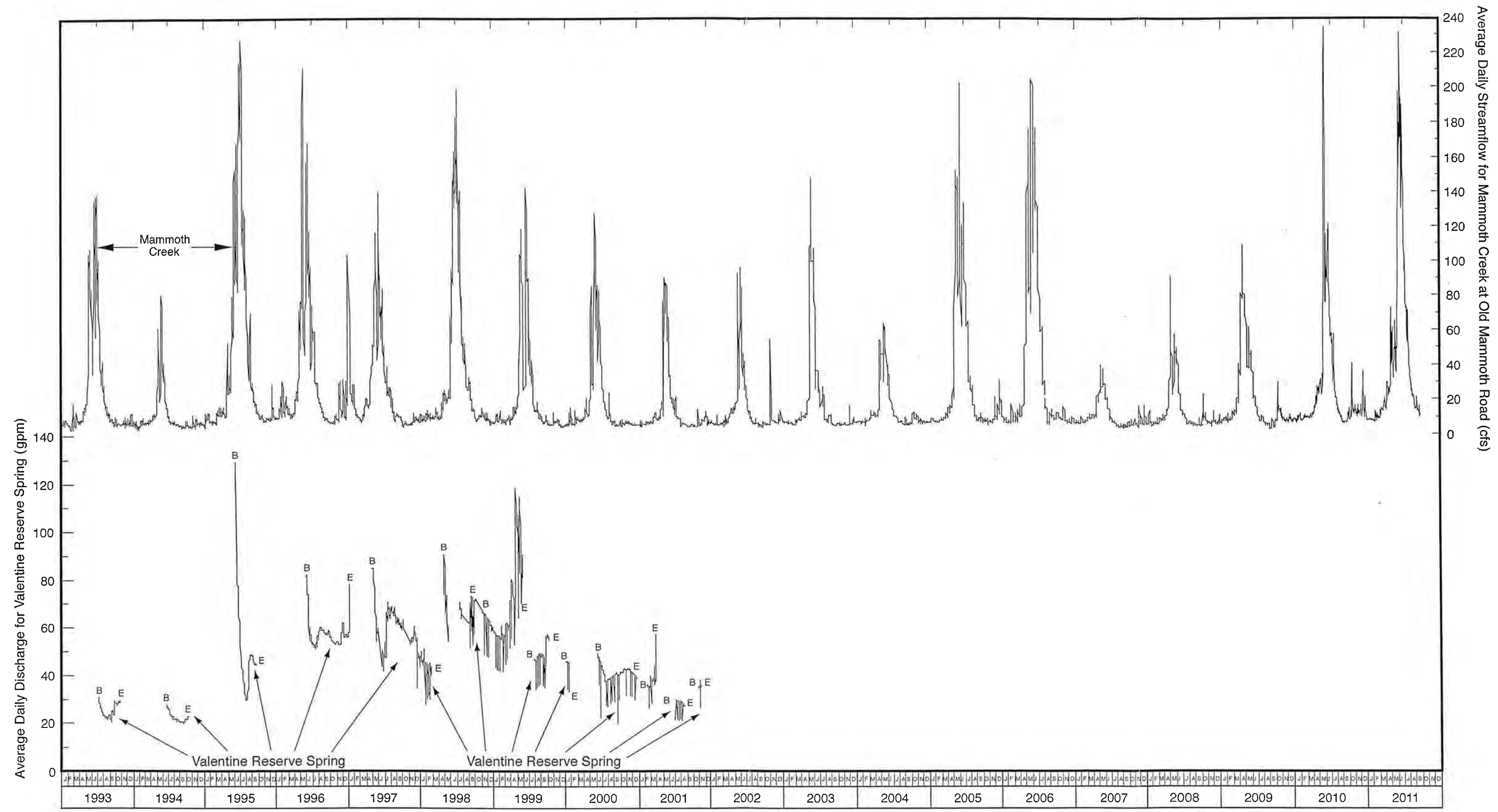
FIGURE 19 - FLOW FOR VALENTINE SPRING (1993-2001) AND MAMMOTH CREEK STREAMFLOW (1993-2011)
