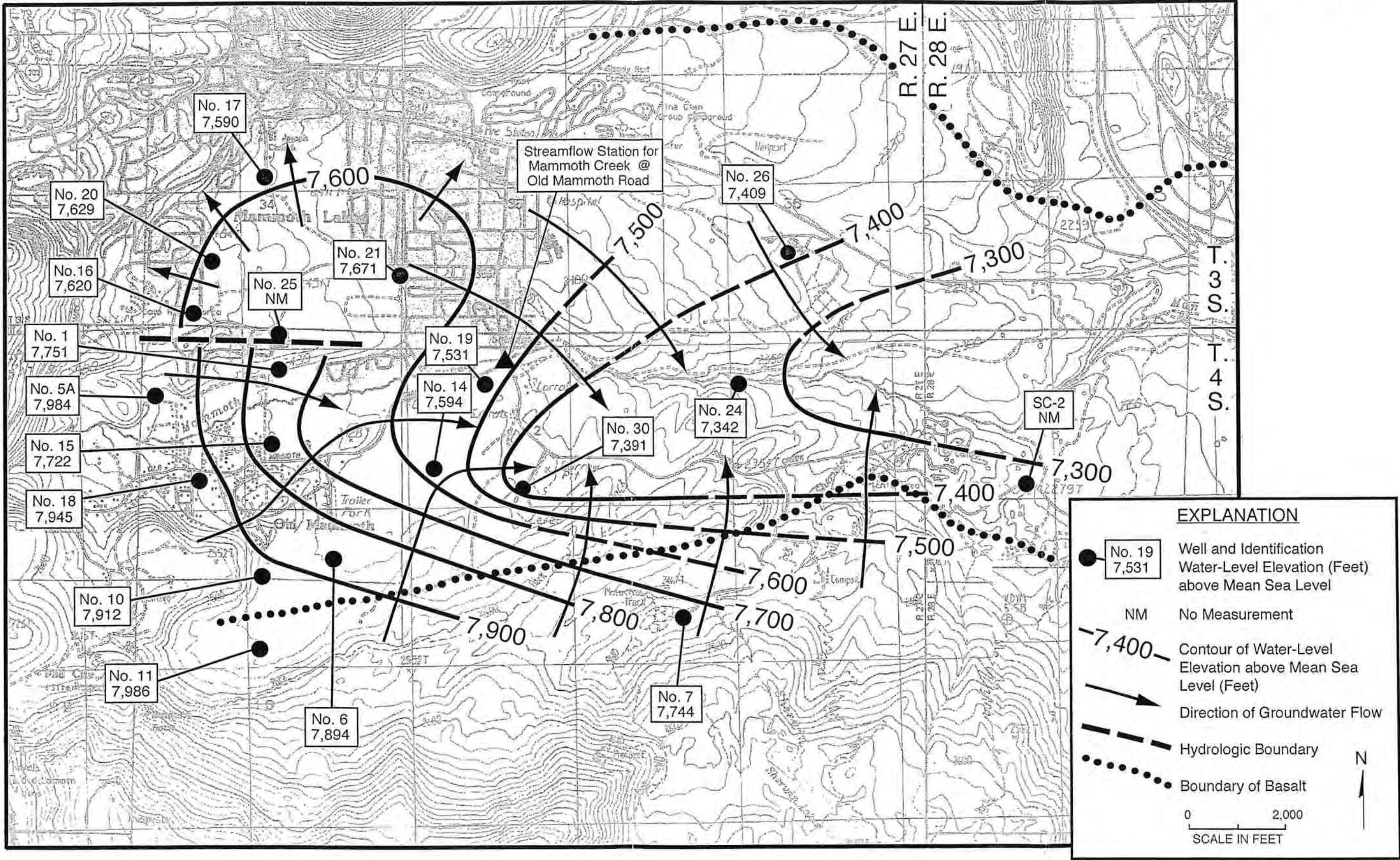
FIGURE 18 - WATER-LEVEL ELEVATIONS IN SEPTEMBER 2011
