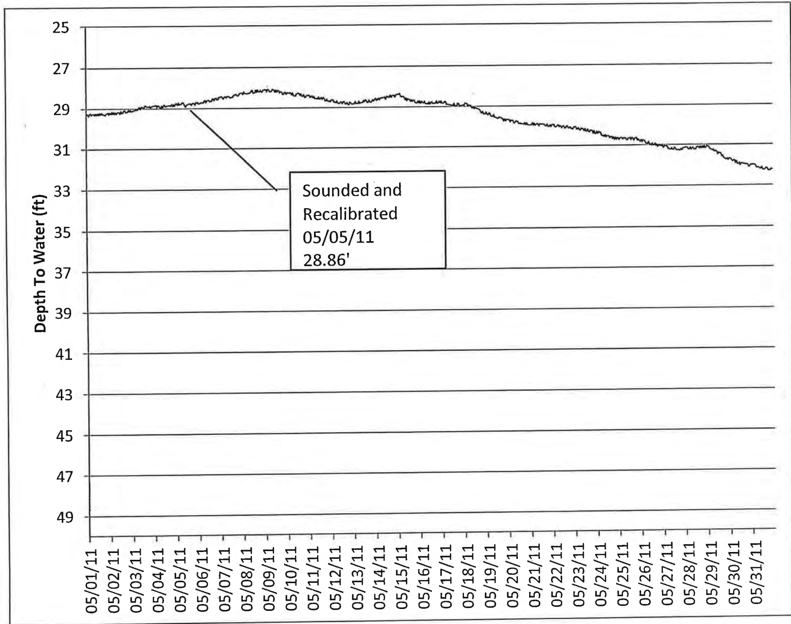
WATER LEVEL HYDROGRAPH FOR MW-27M
