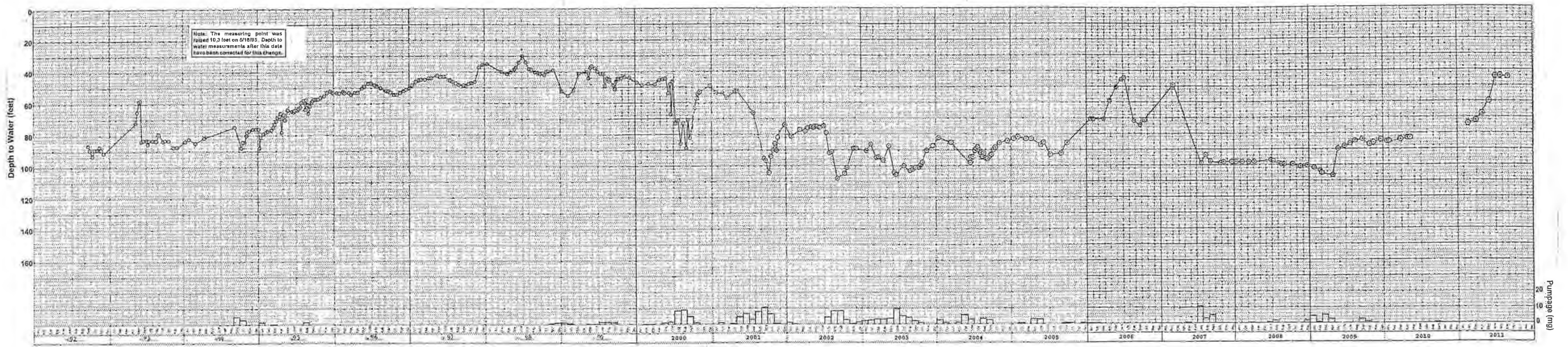
FIGURE 6-WATER-LEVEL AND PUMPAGE HYDROGRAPH FOR WELL NO. 18
