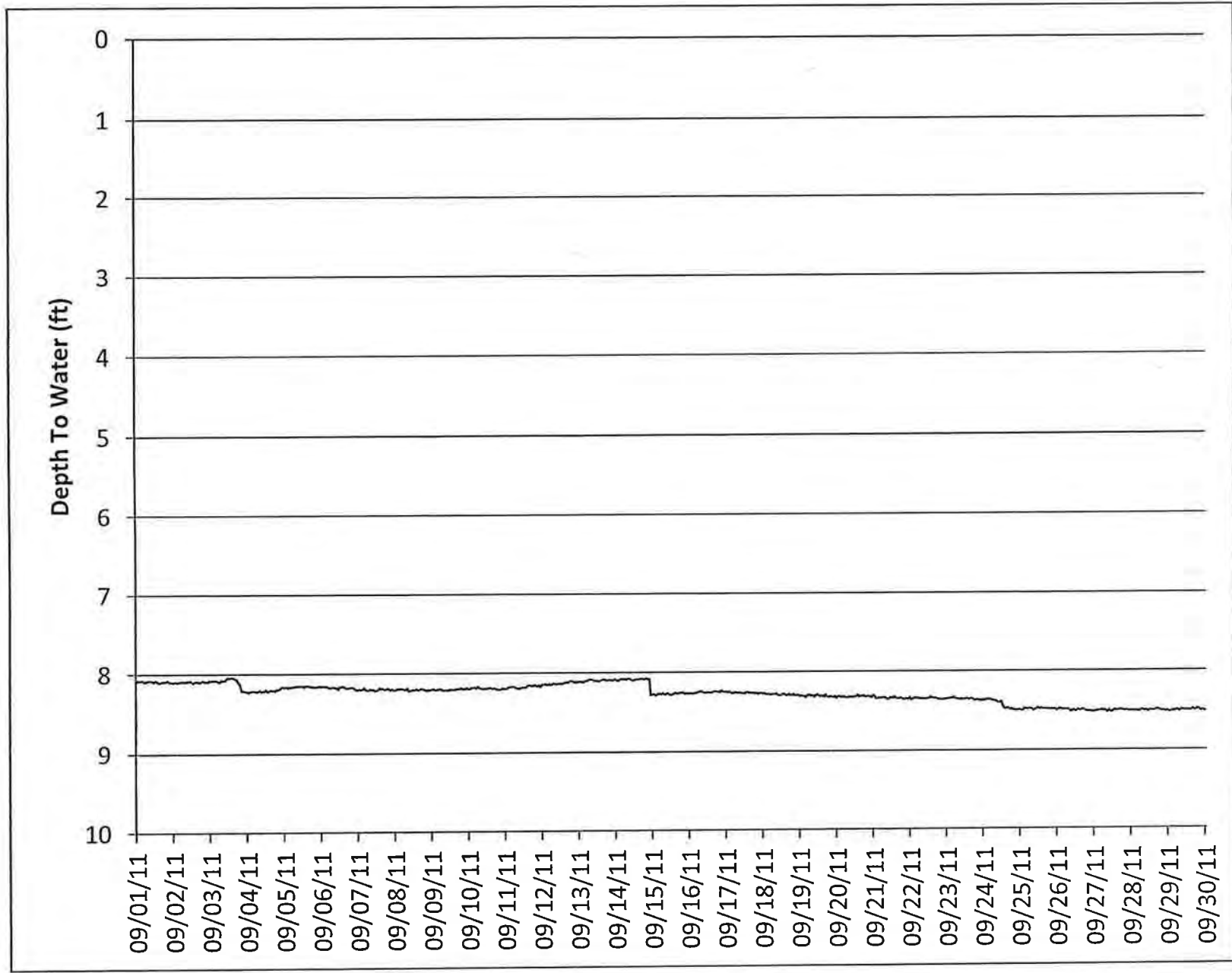
WATER LEVEL HYDROGRAPH FOR MW-5M
