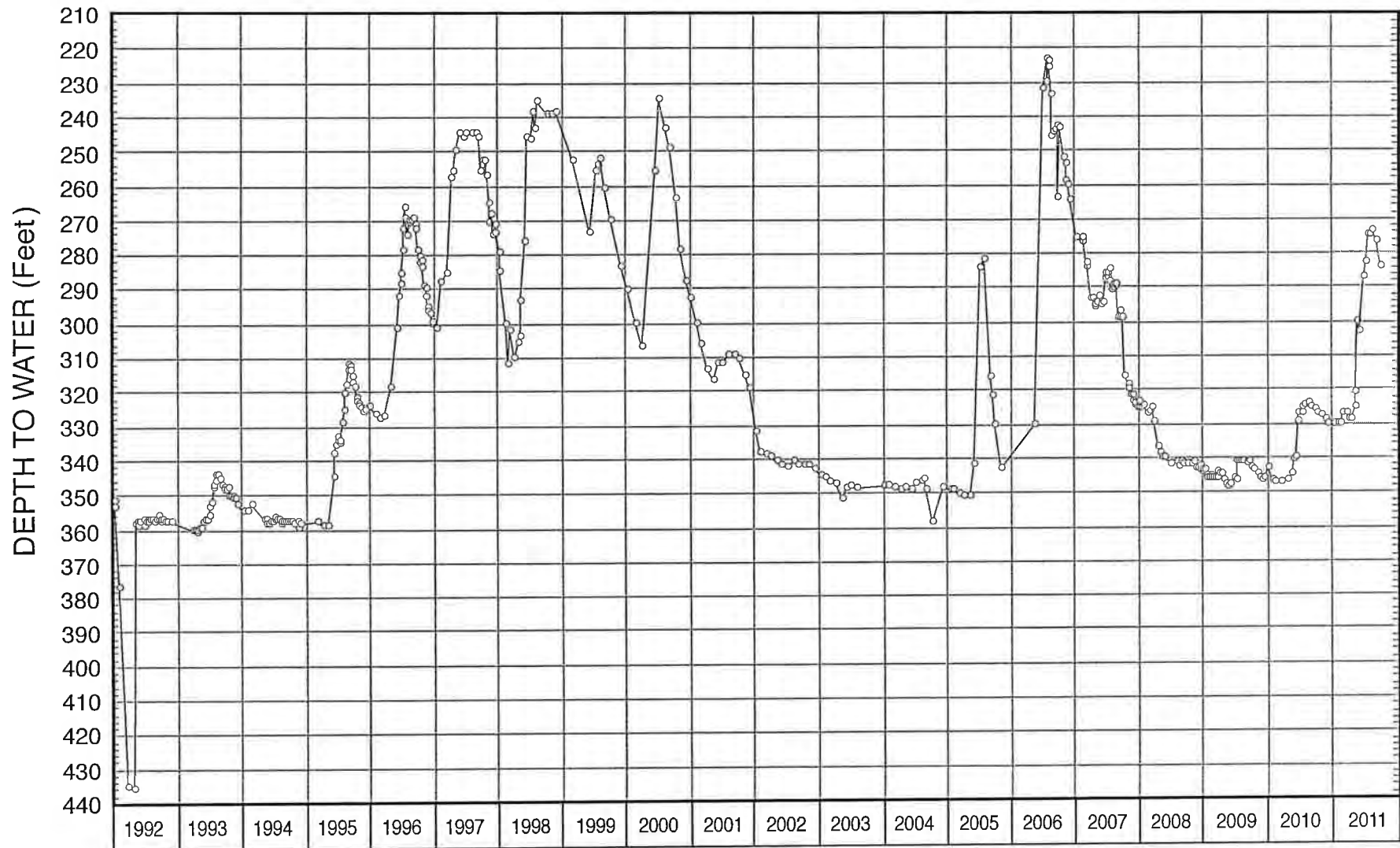
FIGURE 8 - WATER-LEVEL HYDROGRAPH FOR WELL NO. 14M
