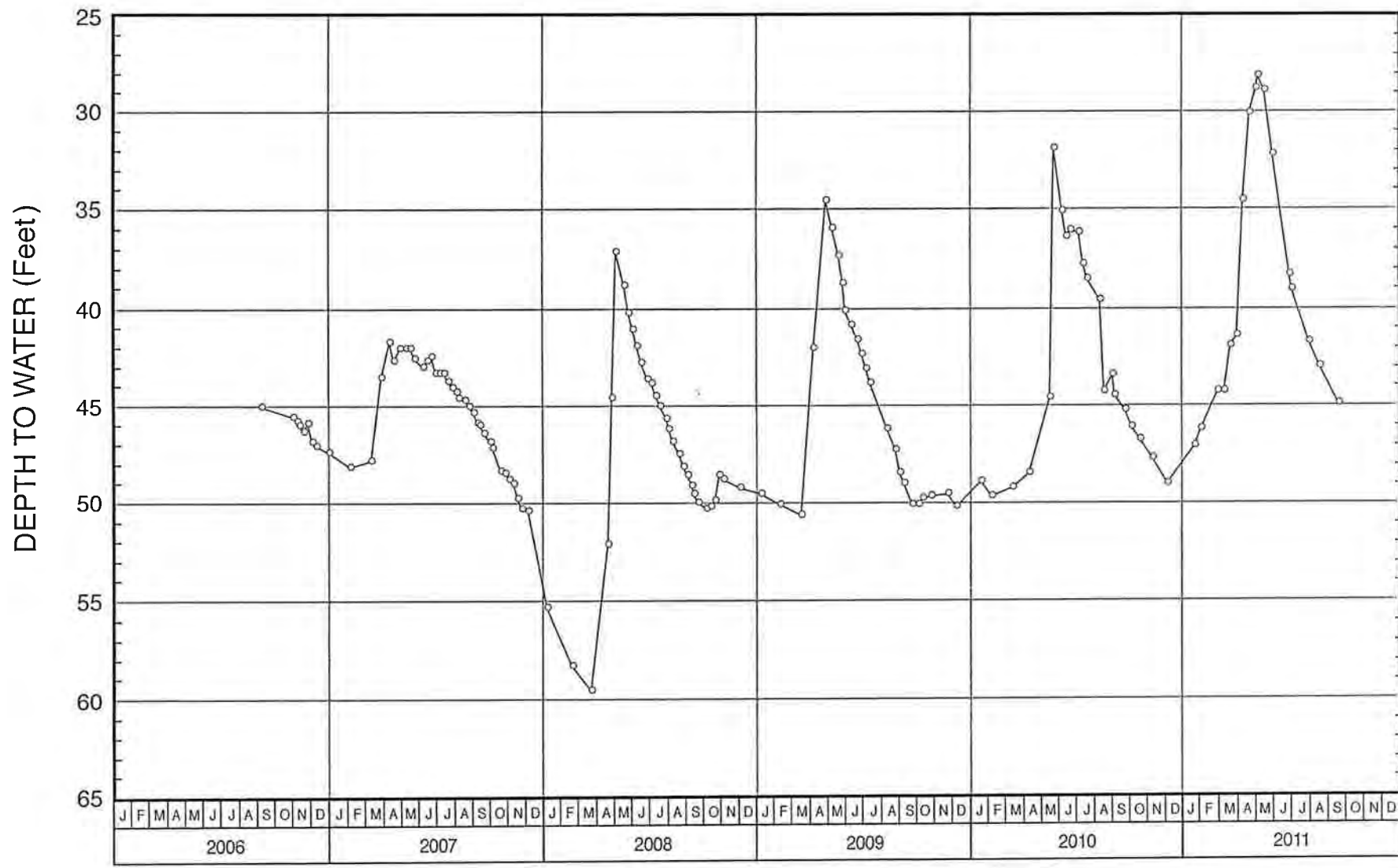
WATER-LEVEL HYDROGRAPH FOR WELL NO. 27
