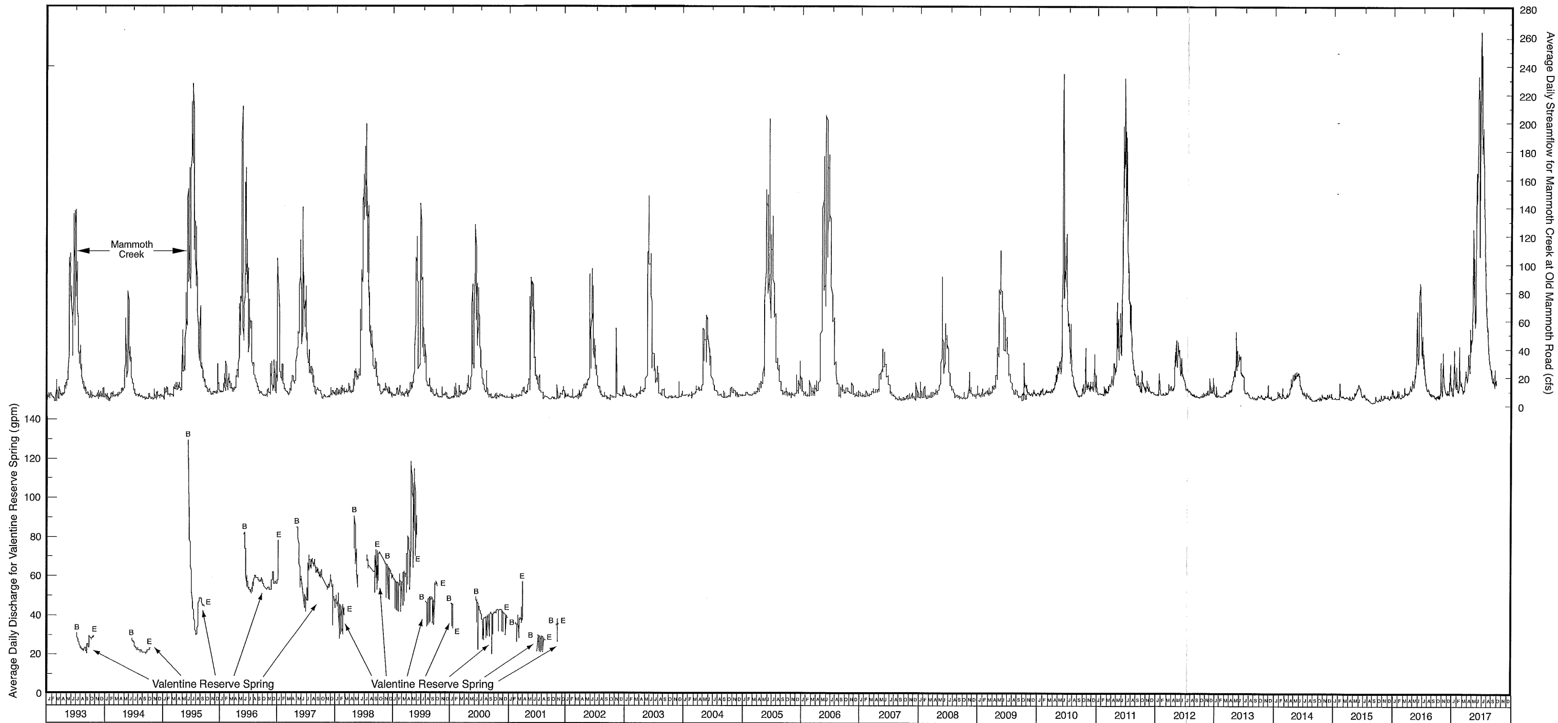
FIGURE 24 - FLOW FOR VALENTINE SPRING (1993-2001) AND MAMMOTH CREEK STREAMFLOW (1993-2017)
