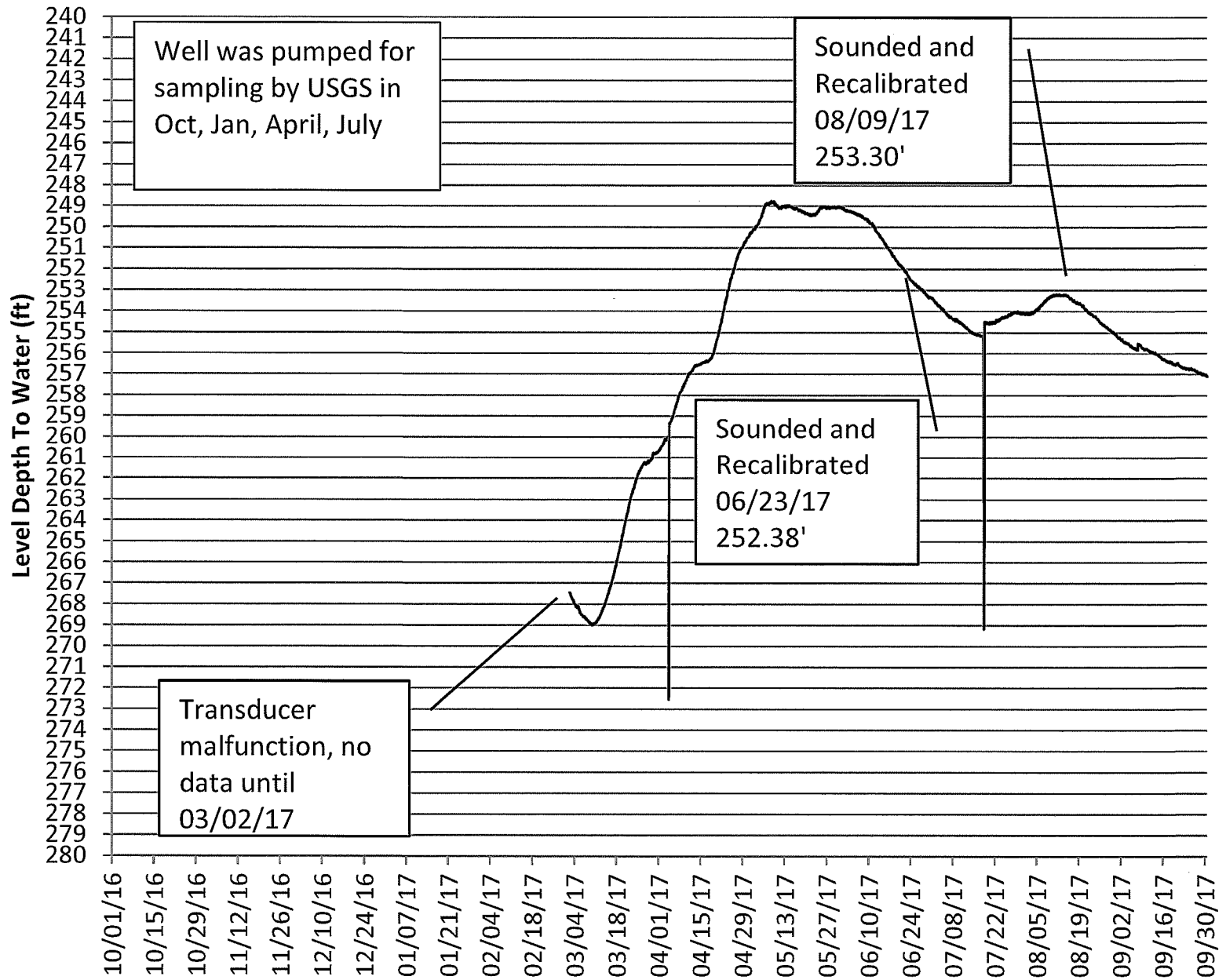
WATER LEVEL HYDROGRAPH FOR MW-26M
