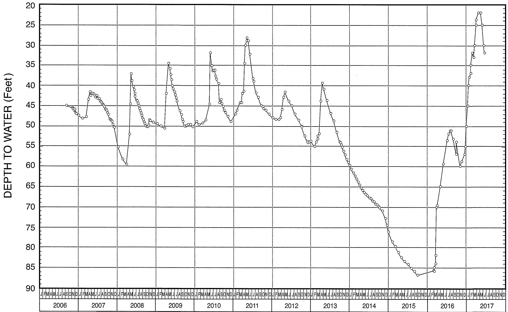
WATER-LEVEL HYDROGRAPH FOR WELL NO. 27
