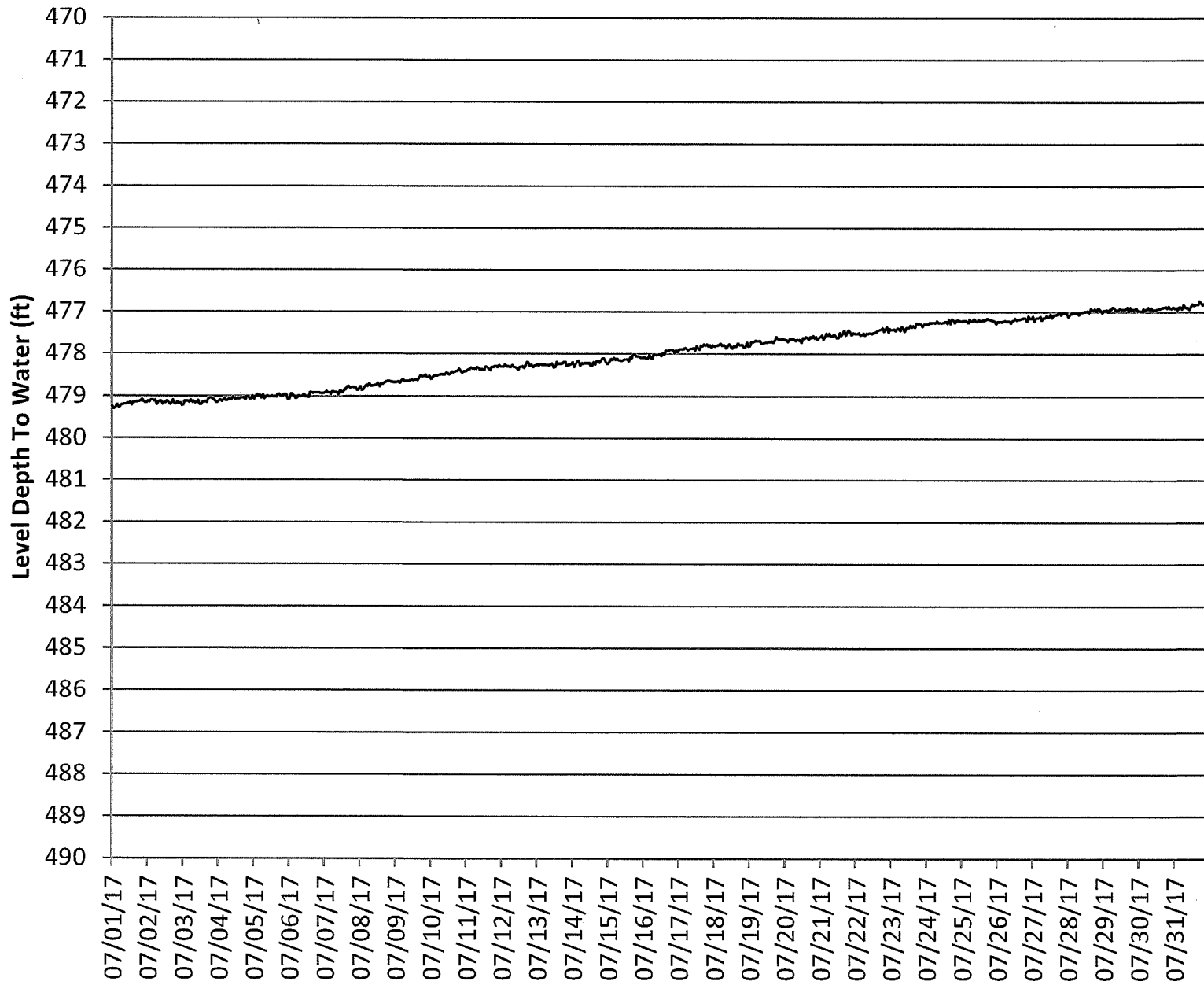
WATER LEVEL HYDROGRAPH FOR MW-30M
