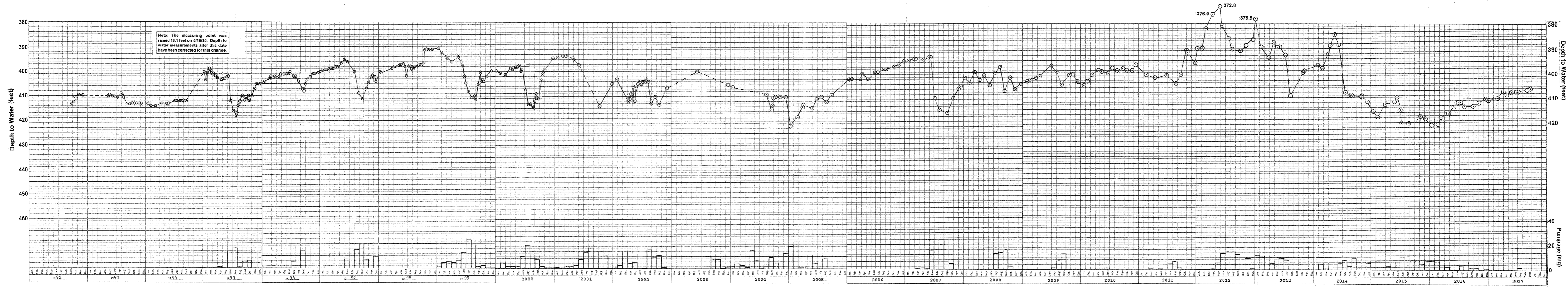
FIGURE 7-WATER-LEVEL AND PUMPAGE HYDROGRAPH FOR WELL NO. 20
