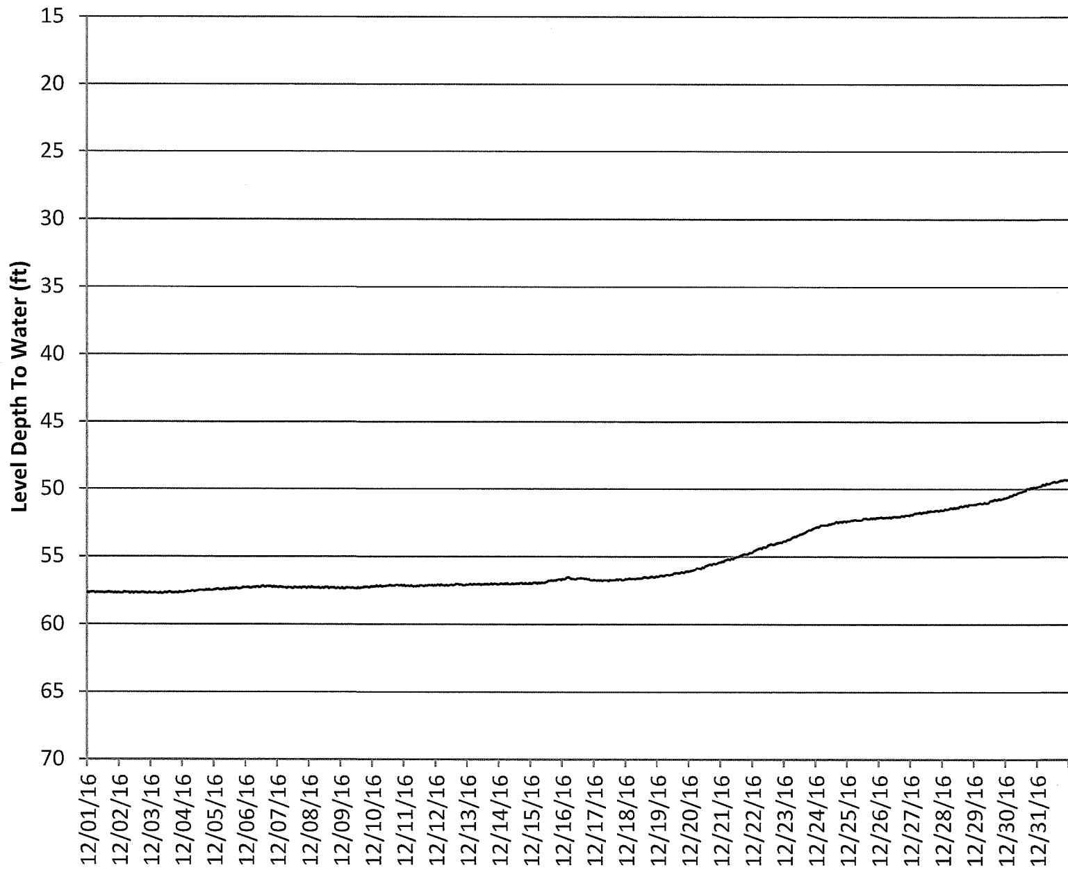
WATER LEVEL HYDROGRAPH FOR MW-27M
