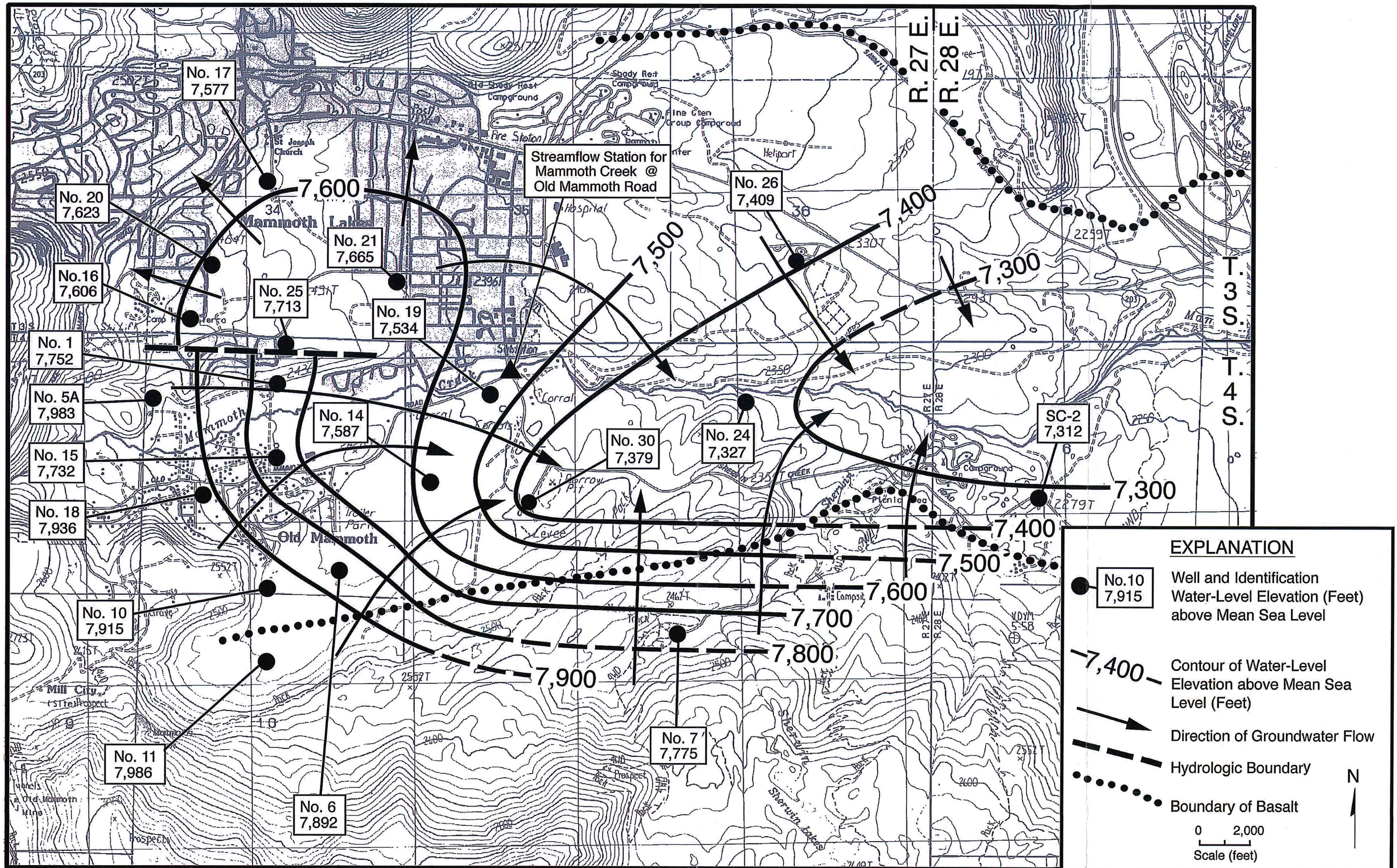
FIGURE 19 - WATER-LEVEL ELEVATIONS IN LATE SEPTEMBER 2017
