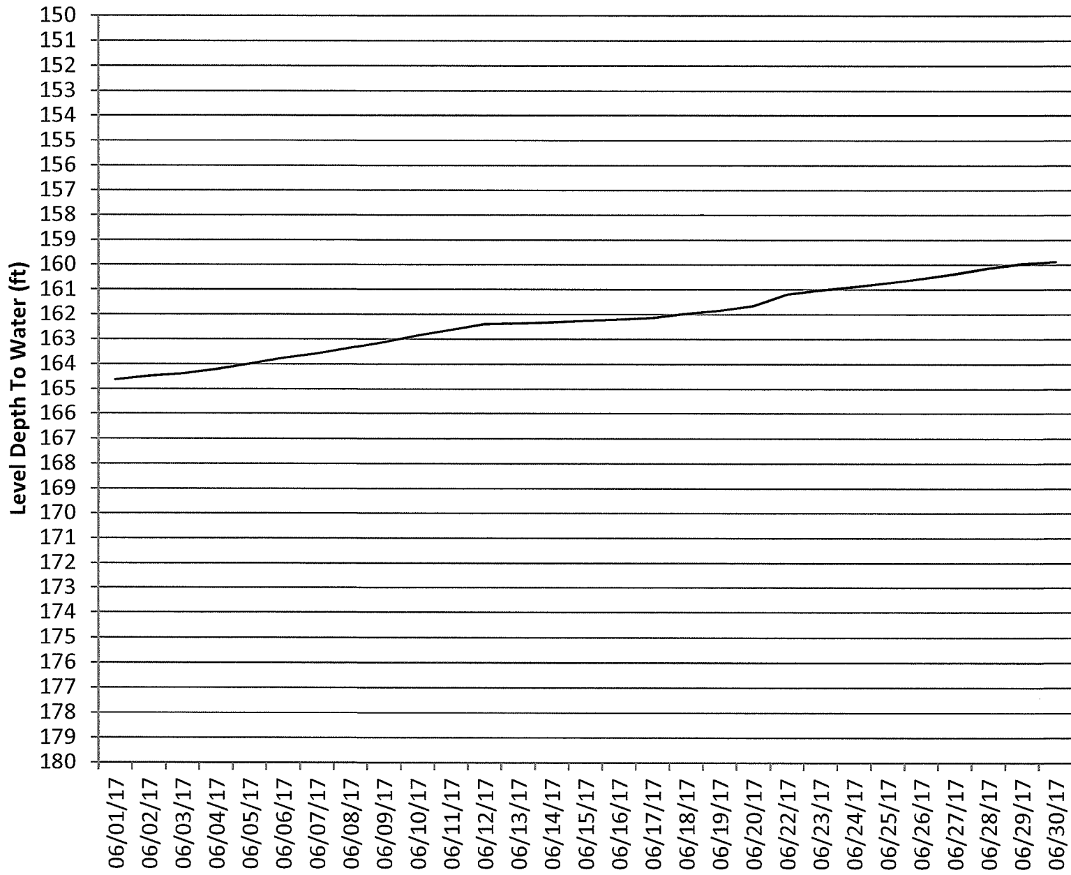
WATER LEVEL HYDROGRAPH FOR MW-SC-2
