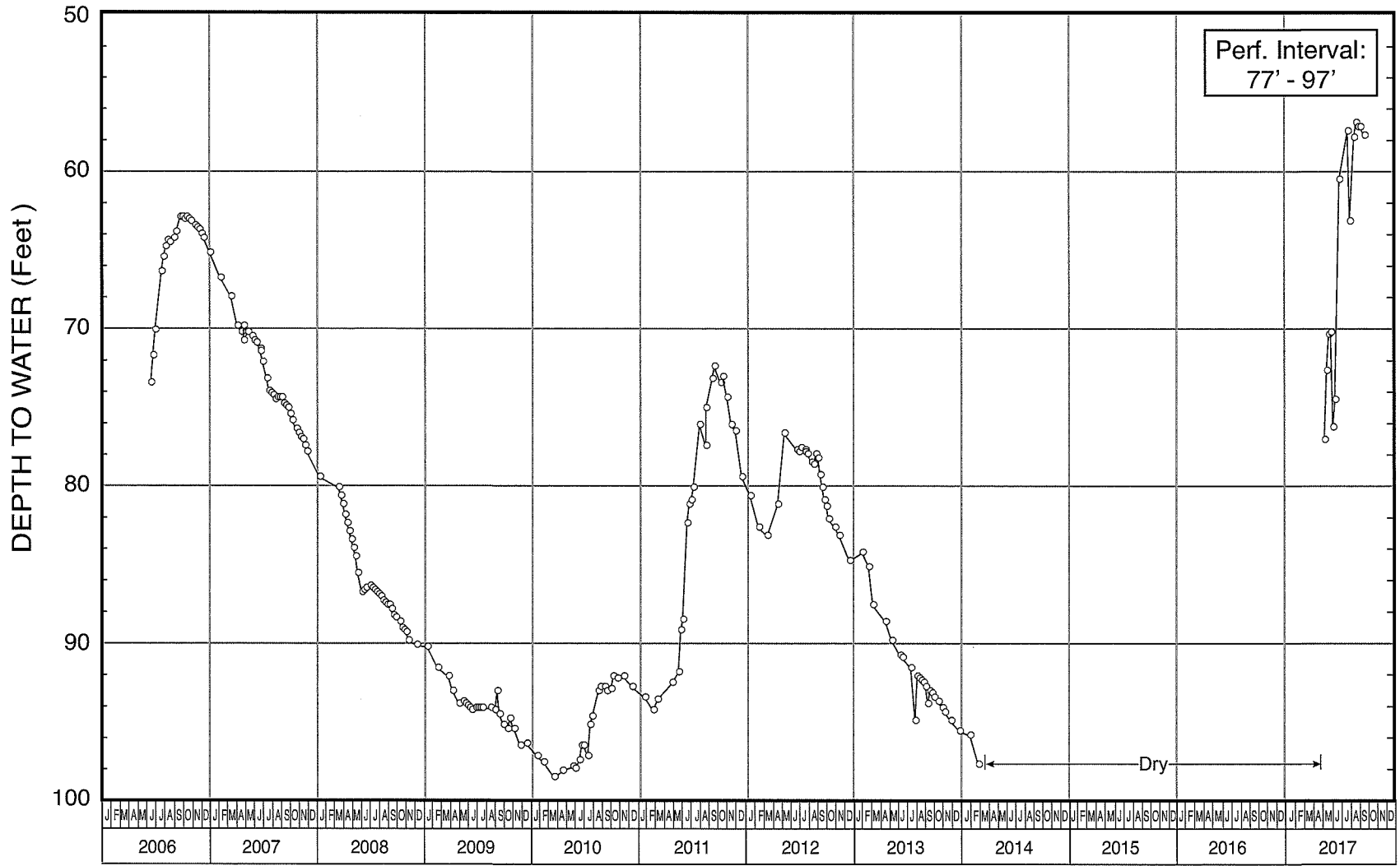
WATER-LEVEL HYDROGRAPH FOR WELL NO. 29
