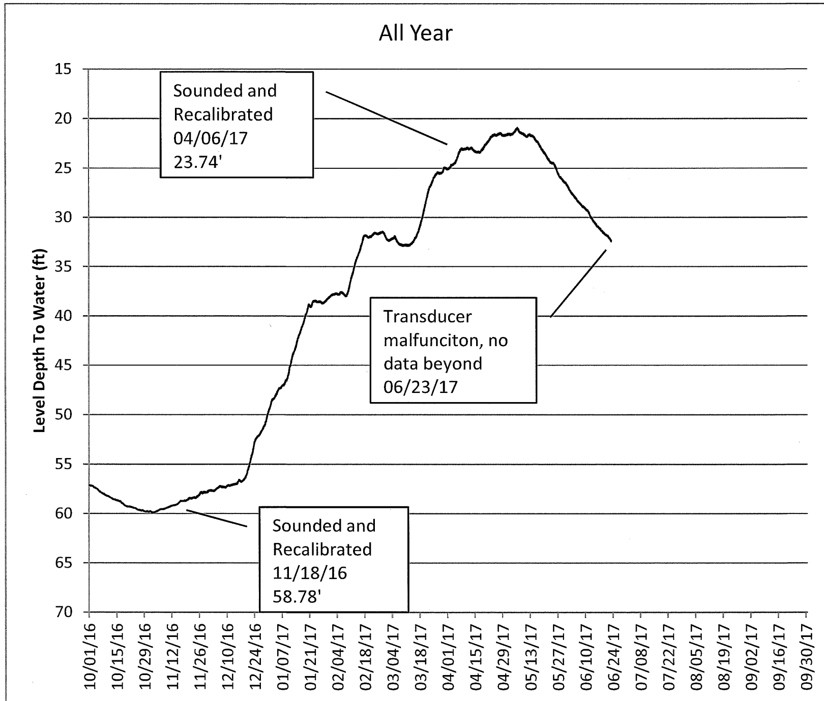
WATER LEVEL HYDROGRAPH FOR MW-27M
