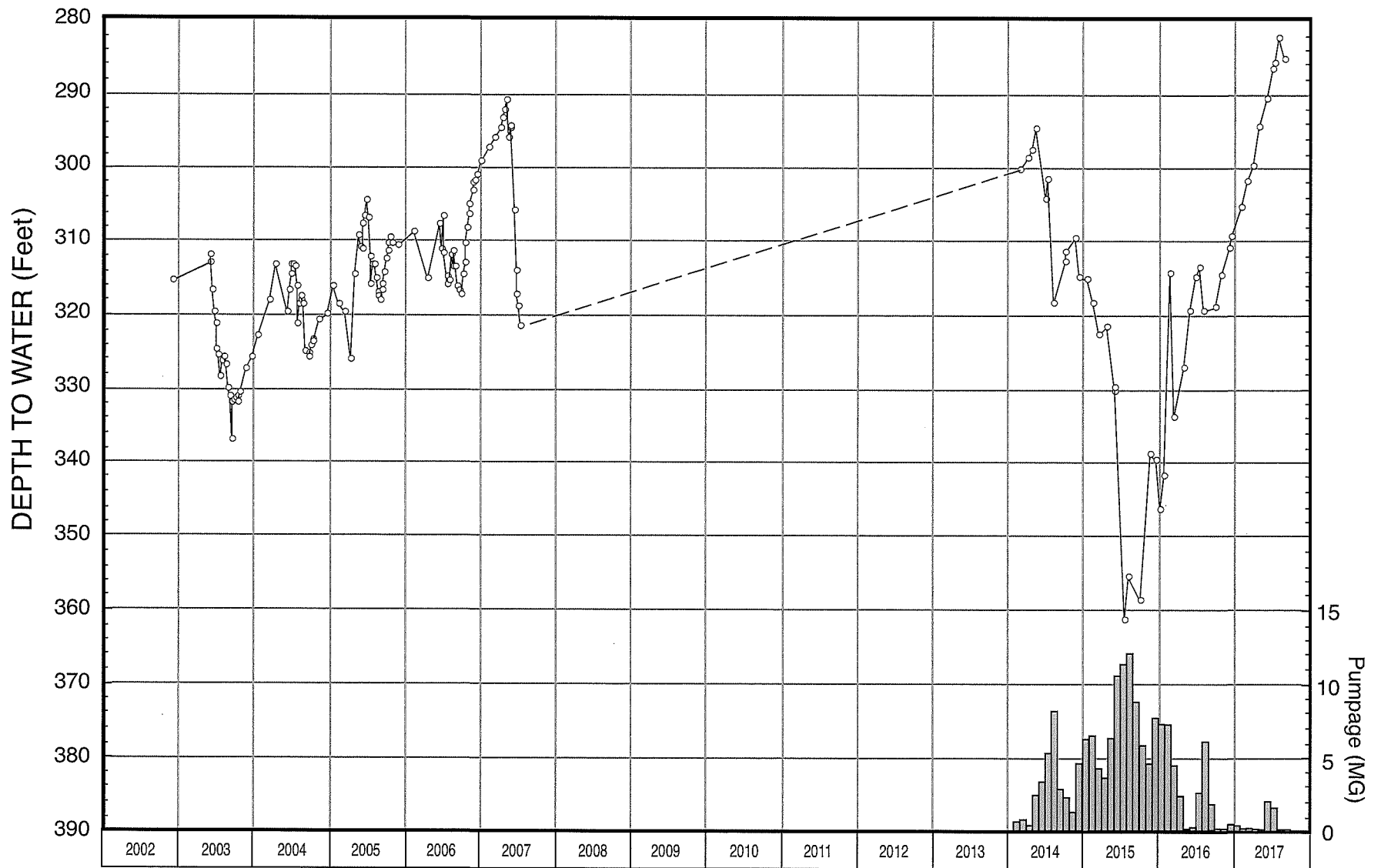
FIGURE 8 - WATER-LEVEL HYDROGRAPH FOR WELL NO. 25
