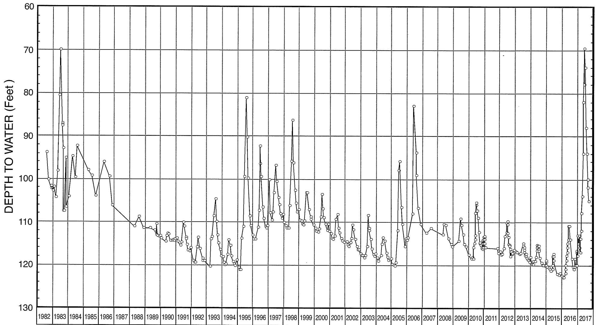
FIGURE 13 - WATER-LEVEL HYDROGRAPH FOR SC-1
