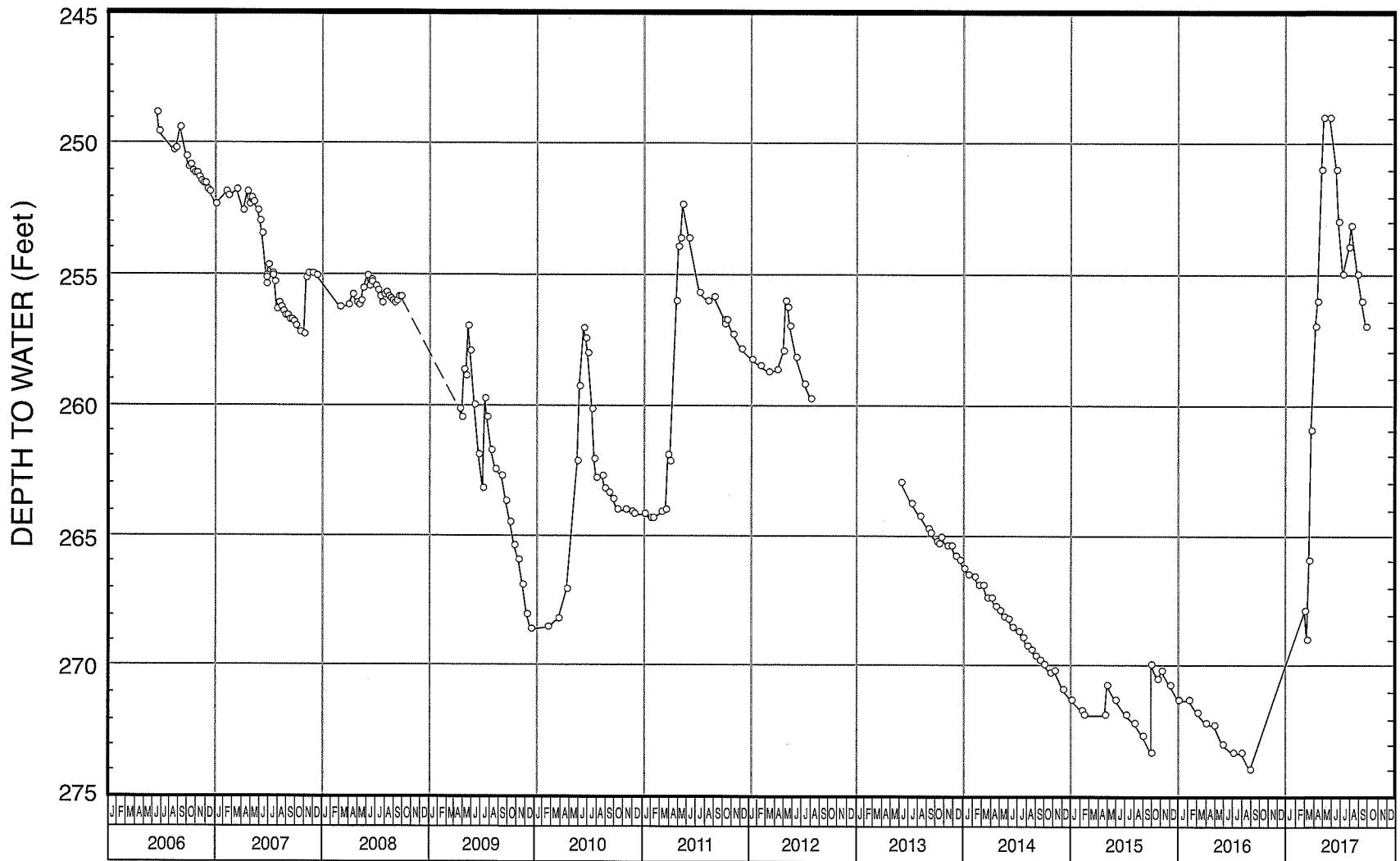
WATER-LEVEL HYDROGRAPH FOR WELL NO. 26
