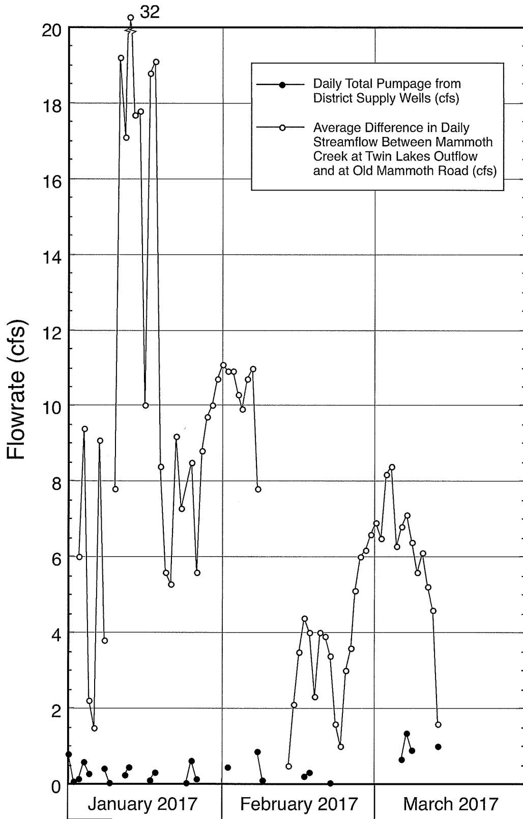
FIGURE 20 - RELATIONSHIP BETWEEN DIFFERENCE IN MAMMOTH CREEK STREAMFLOW AT TWIN LAKES OUTFLOW AND OLD MAMMOTH ROAD AND DISTRICT SUPPLY WELL PUMPAGE (JANUARY - MARCH 2017)
