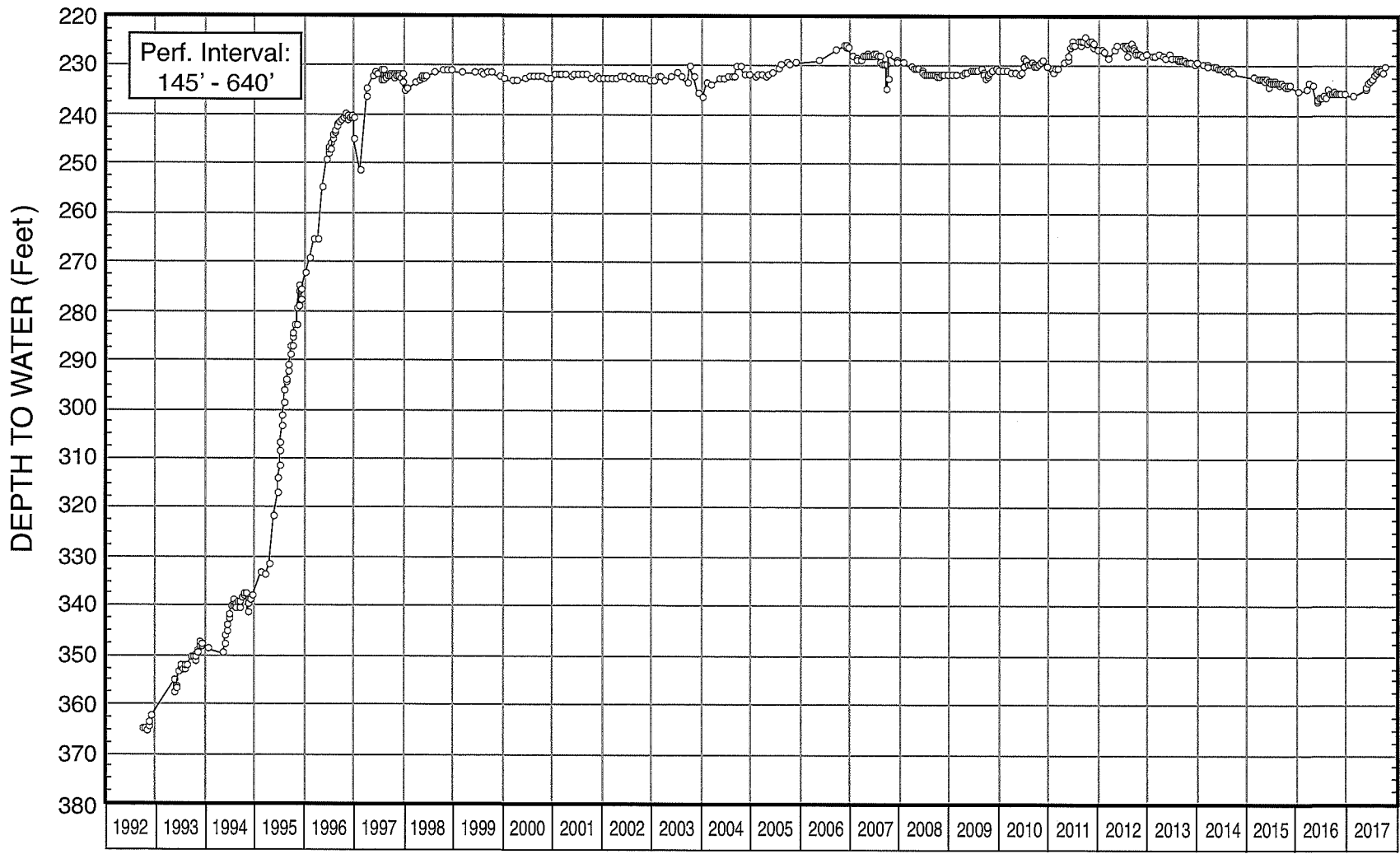
FIGURE 11 - WATER-LEVEL HYDROGRAPH FOR WELL NO. 21
