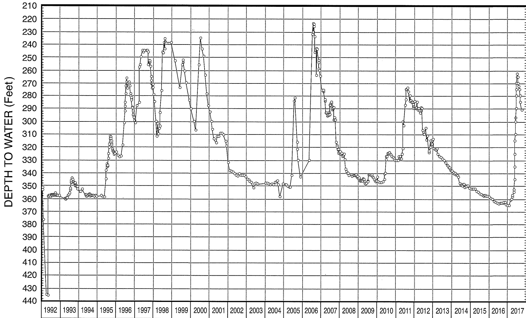
FIGURE 9 - WATER-LEVEL HYDROGRAPH FOR WELL NO. 14M
