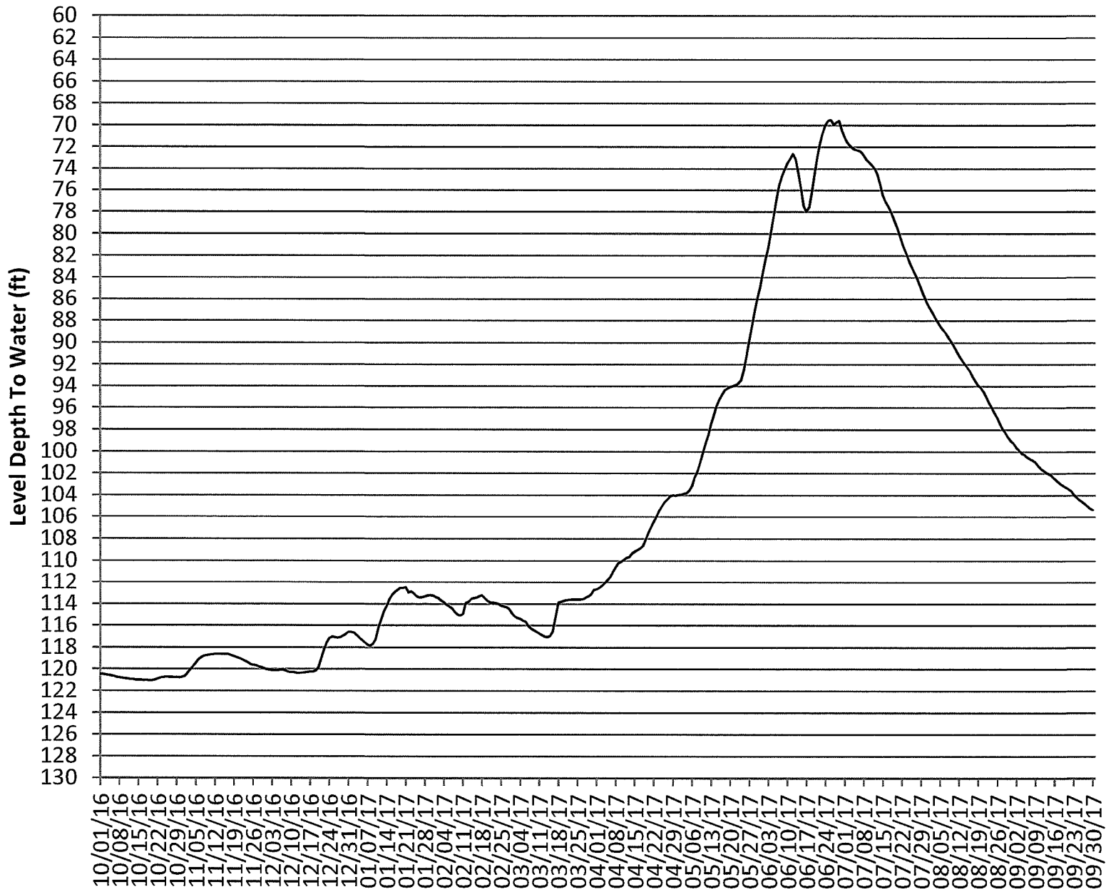
WATER LEVEL HYDROGRAPH FOR MW-SC-1
