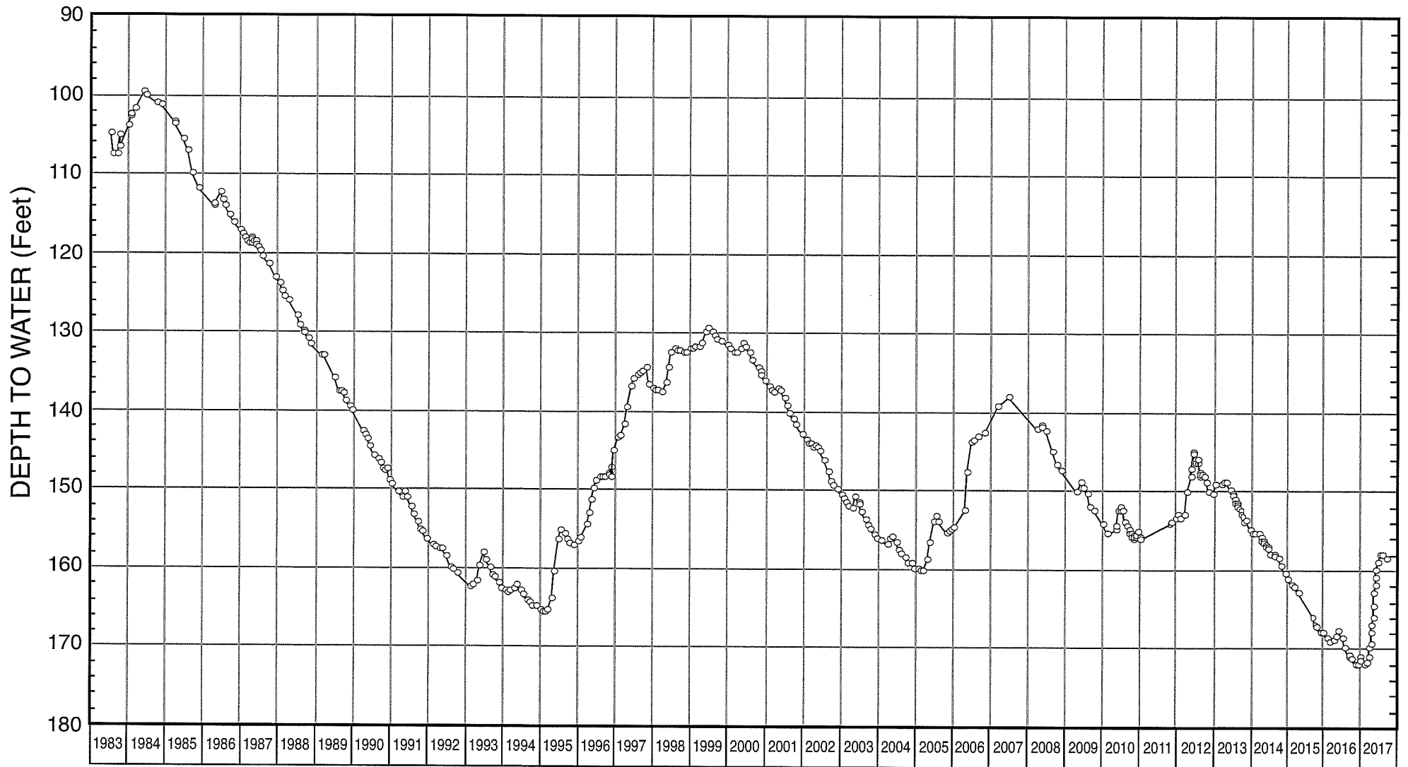
FIGURE 14 - WATER-LEVEL HYDROGRAPH FOR SC-2
