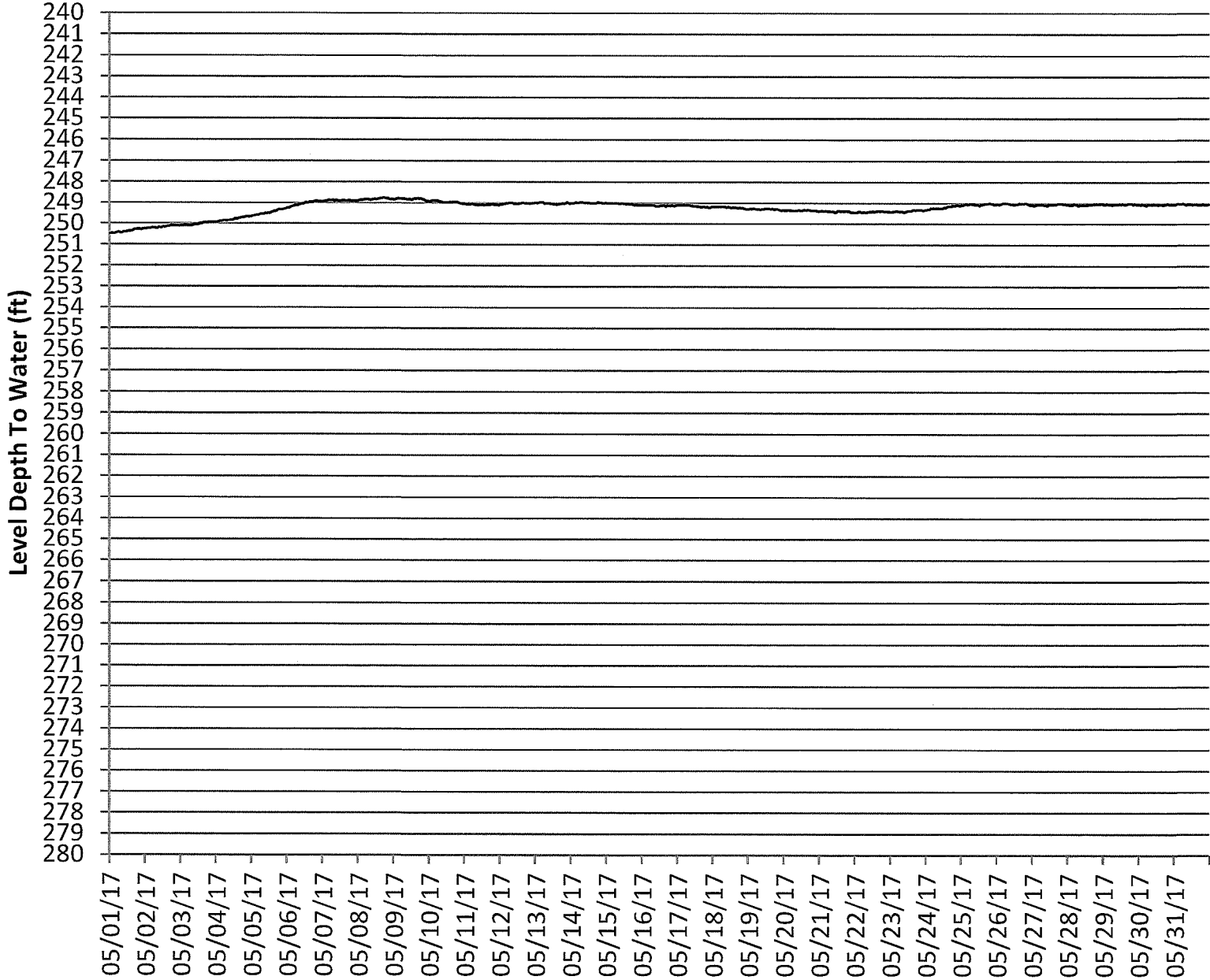
WATER LEVEL HYDROGRAPH FOR MW-26M
