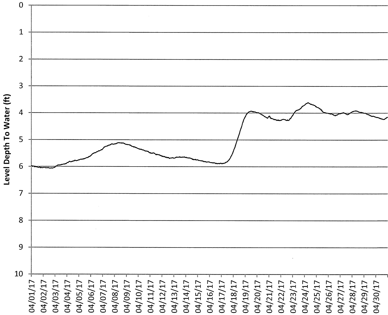
WATER LEVEL HYDROGRAPH FOR MW-5M
