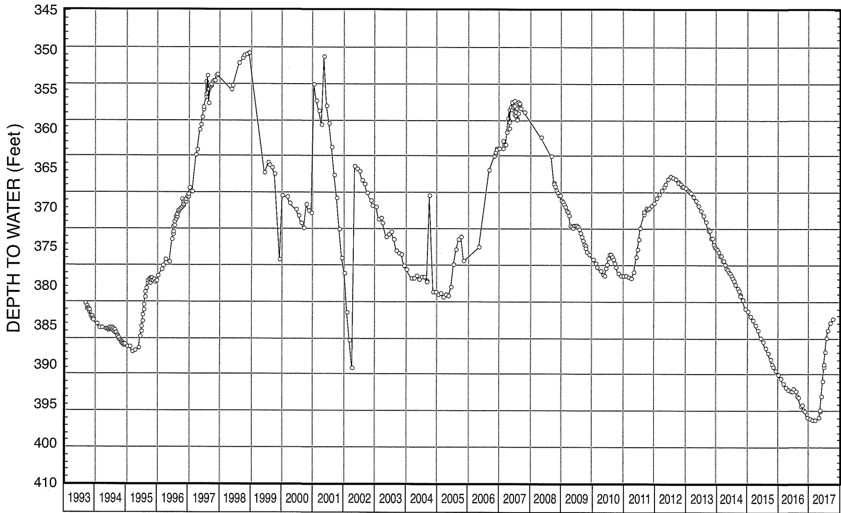
FIGURE 12 - WATER-LEVEL HYDROGRAPH FOR WELL NO. 24
