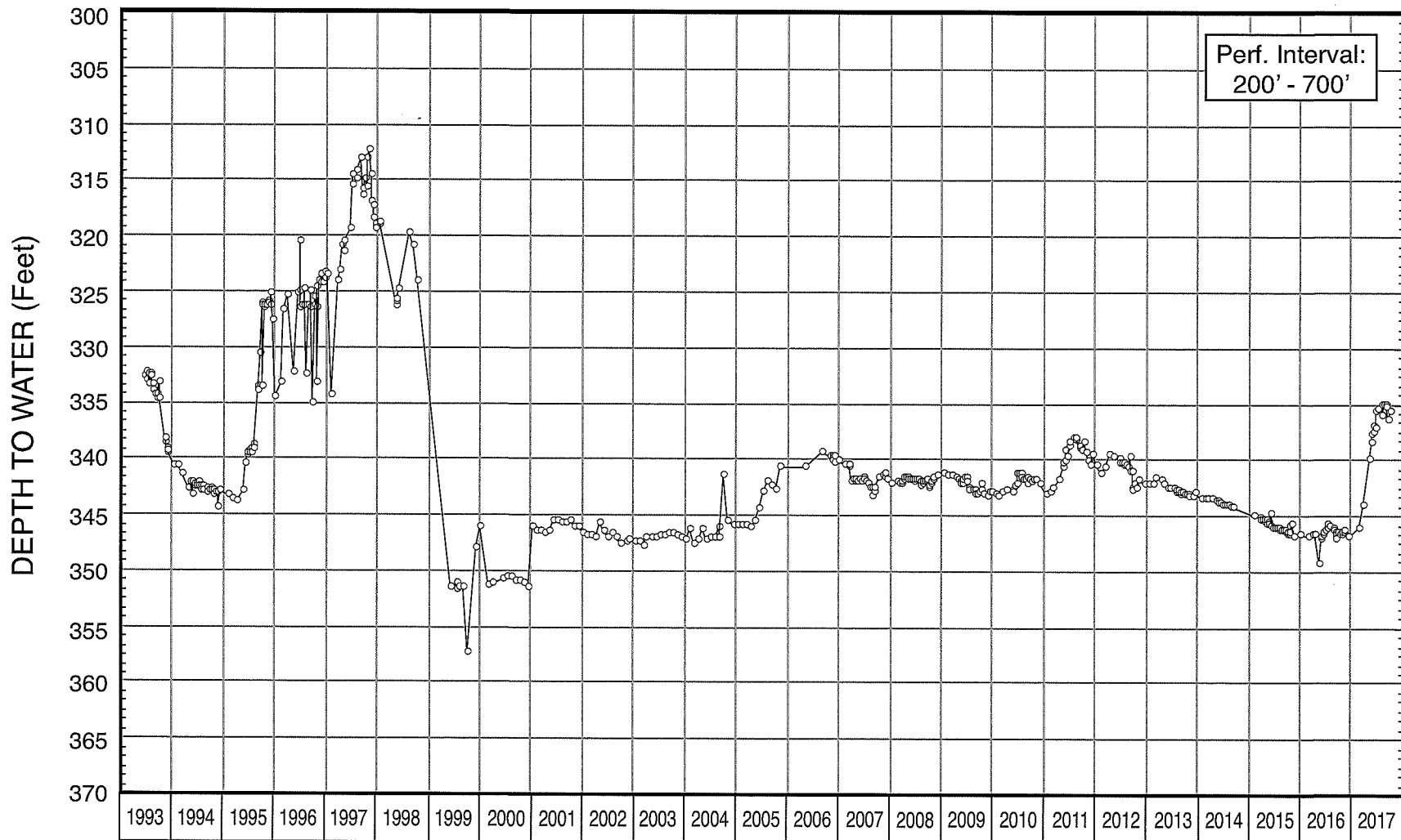
FIGURE 10 - WATER-LEVEL HYDROGRAPH FOR WELL NO. 19
