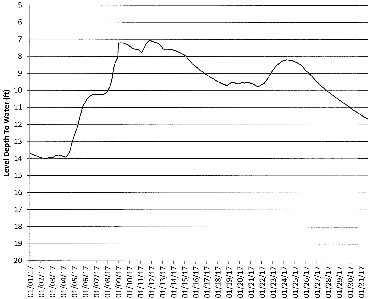
WATER LEVEL HYDROGRAPH FOR MW-23M
