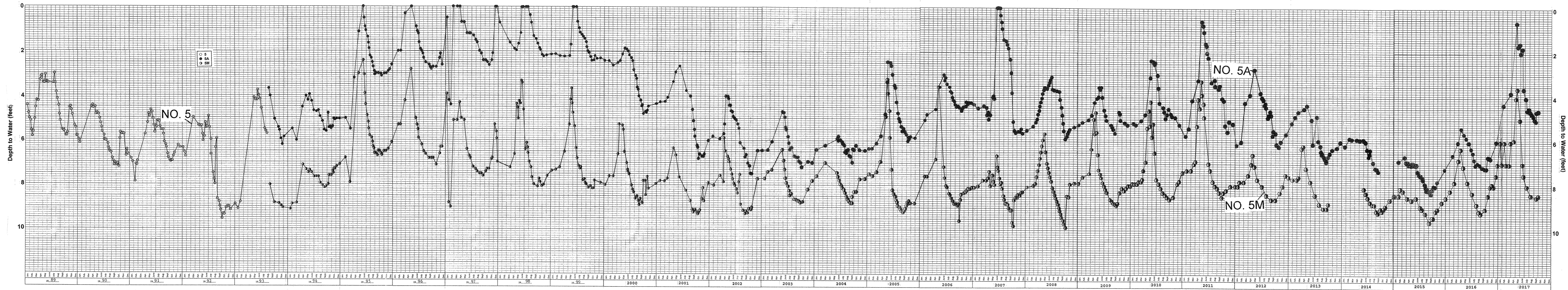
WATER-LEVEL HYDROGRAPH FOR WELL NO. 5, NO. 5A, AND NO. 5M
