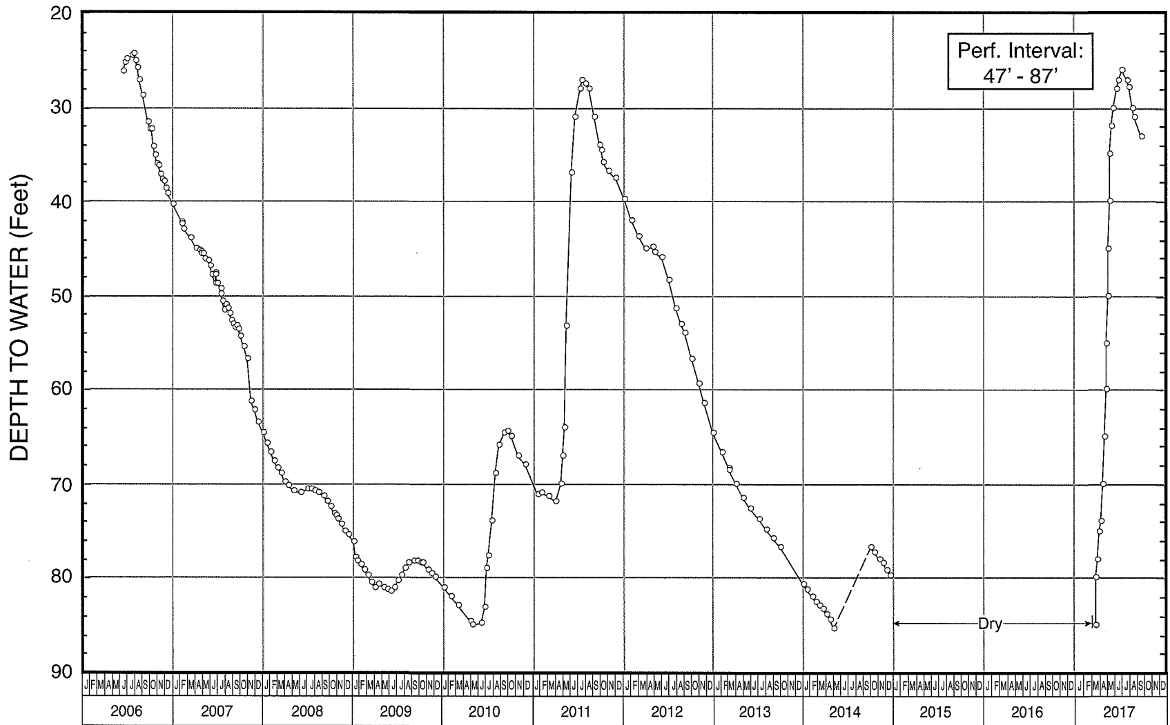
WATER-LEVEL HYDROGRAPH FOR WELL NO. 28
