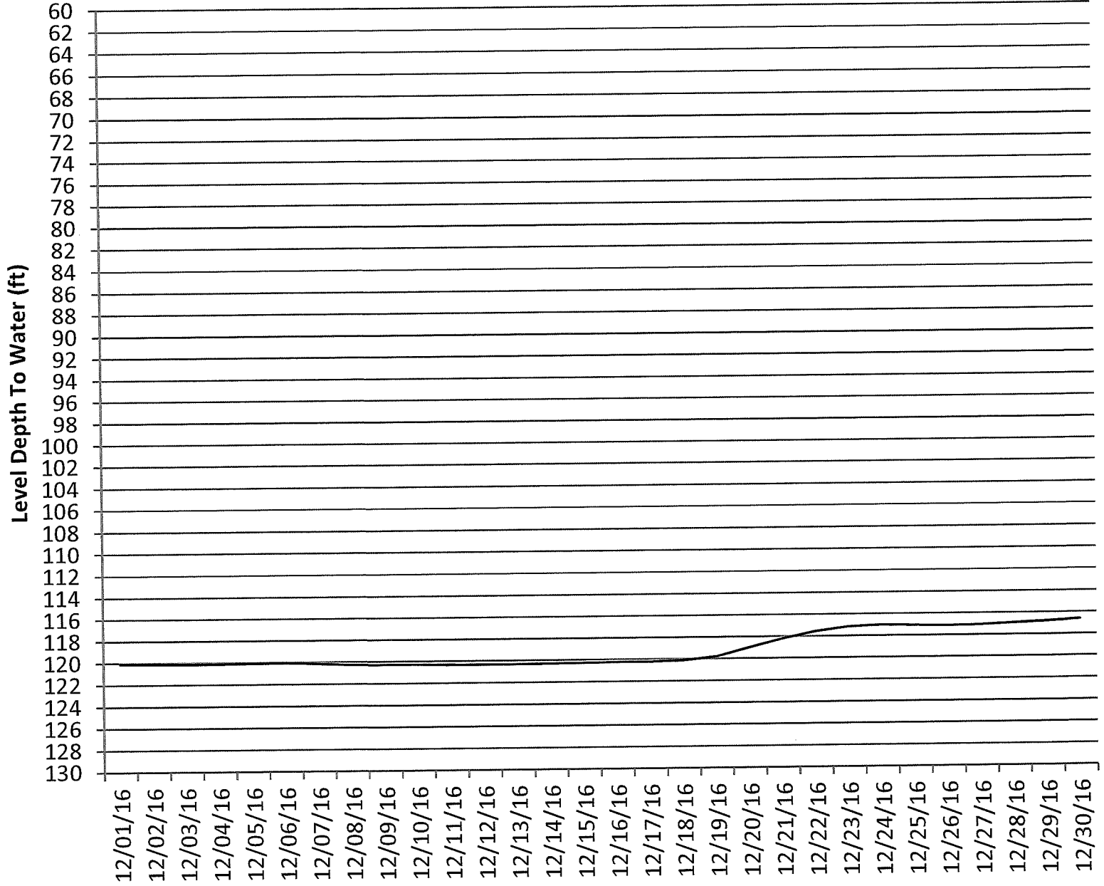
WATER LEVEL HYDROGRAPH FOR MW-SC-1
