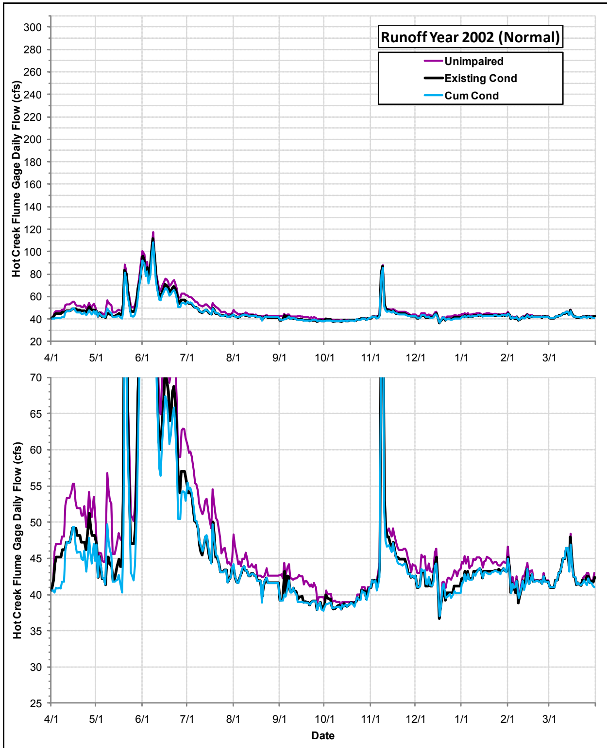
Daily Flows (cfs) at the USGS Hot Creek Flume Gage under the Cumulative Condition, the Existing Condition and the Index of Unimpaired Conditions during Runoff Year 2002
