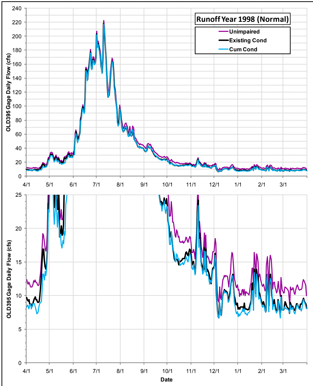
Daily Flows (cfs) at the OLD395 Gage under the Cumulative Condition, the Existing Condition and the Index of Unimpaired Conditions during Runoff Year 1998
