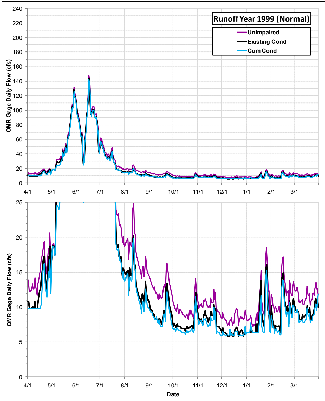
Daily Flows (cfs) at the OMR Gage under the Cumulative Condition, the Existing Condition and the Index of Unimpaired Conditions during Runoff Year 1999
