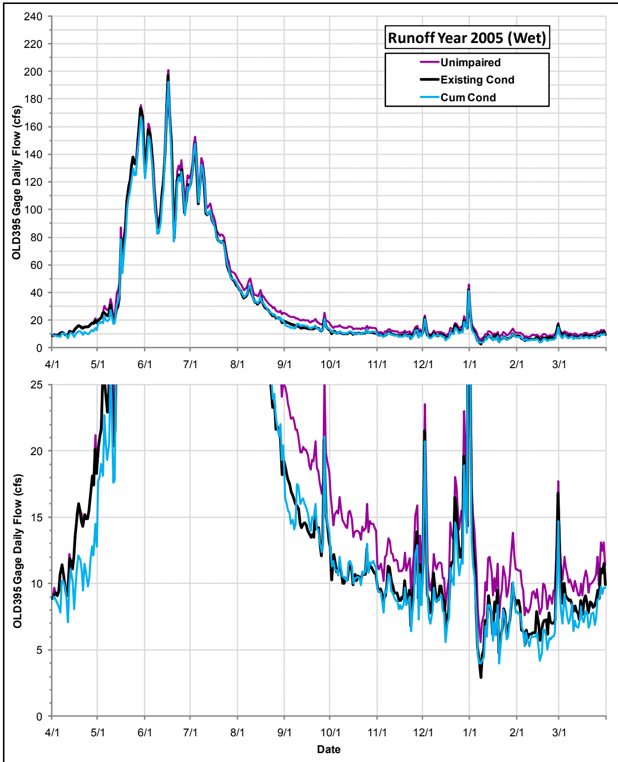
Daily Flows (cfs) at the OLD395 Gage under the Cumulative Condition, the Existing Condition and the Index of Unimpaired Conditions during Runoff Year 2005
