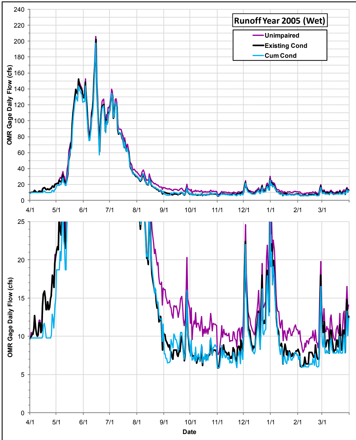
Daily Flows (cfs) at the OMR Gage under the Cumulative Condition, the Existing Condition and the Index of Unimpaired Conditions during Runoff Year 2005
