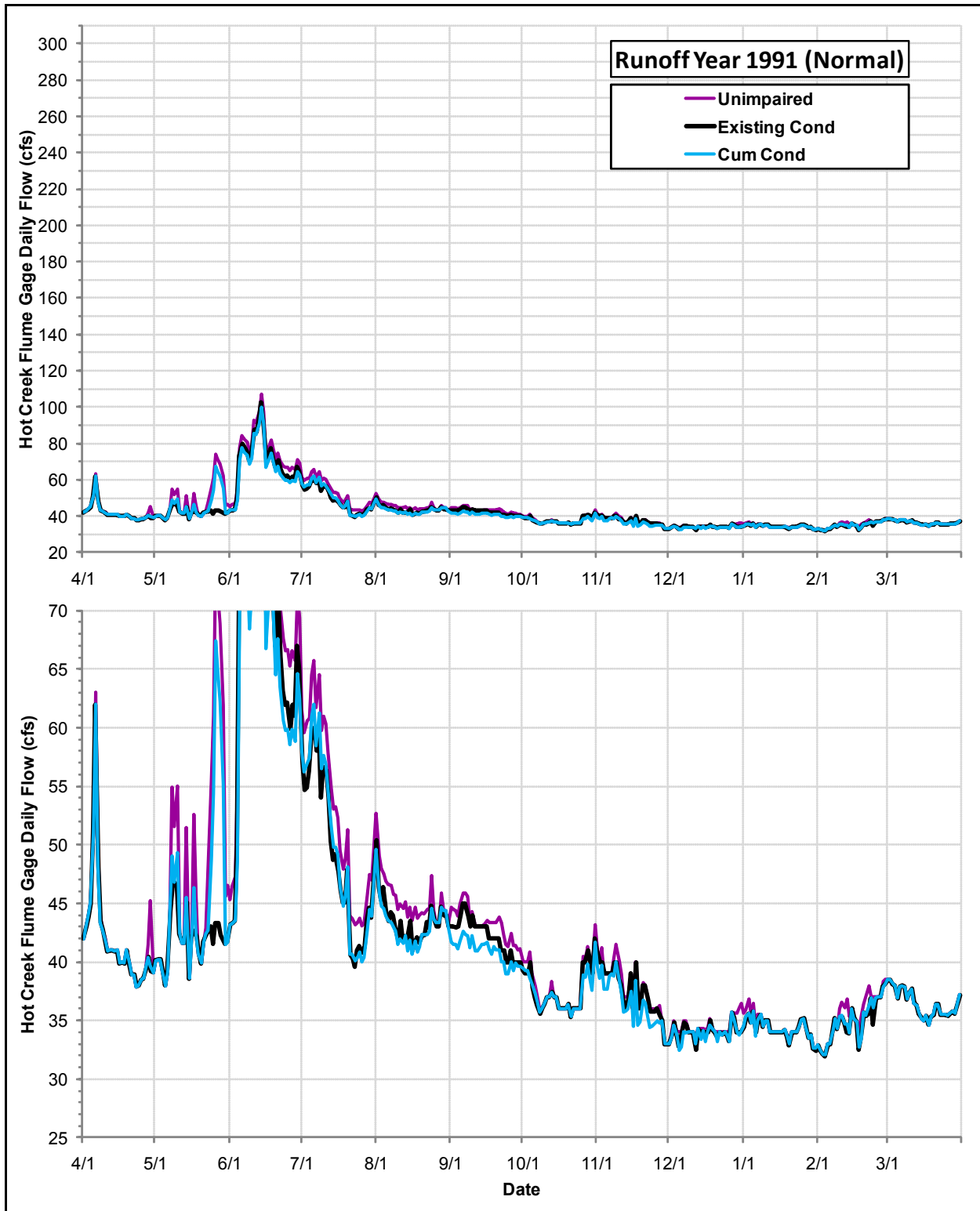
Daily Flows (cfs) at the USGS Hot Creek Flume Gage under the Cumulative Condition, the Existing Condition and the Index of Unimpaired Conditions during Runoff Year 1991
