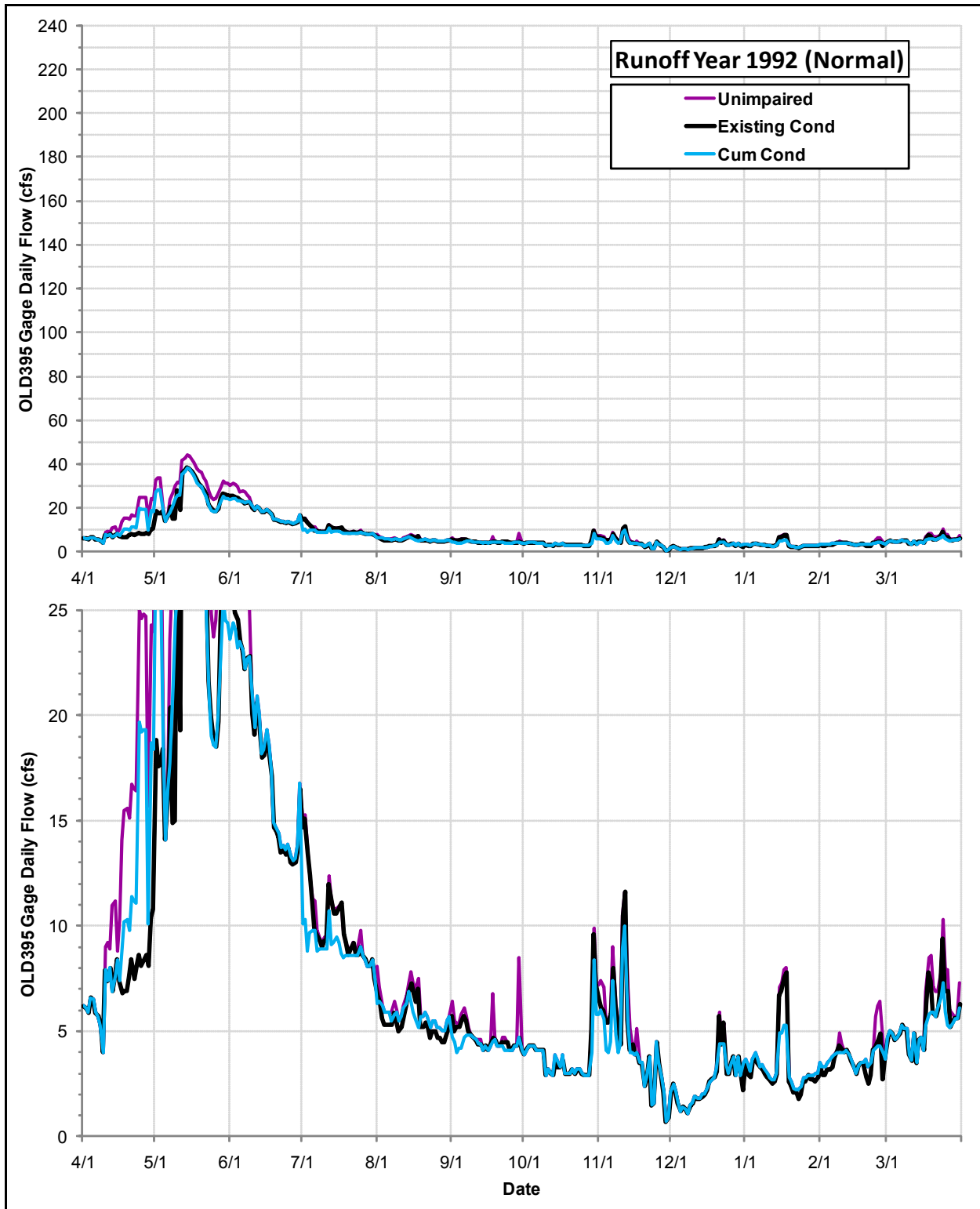
Daily Flows (cfs) at the OLD395 Gage under the Cumulative Condition, the Existing Condition and the Index Unimpaired Conditions during Runoff Year 1992
