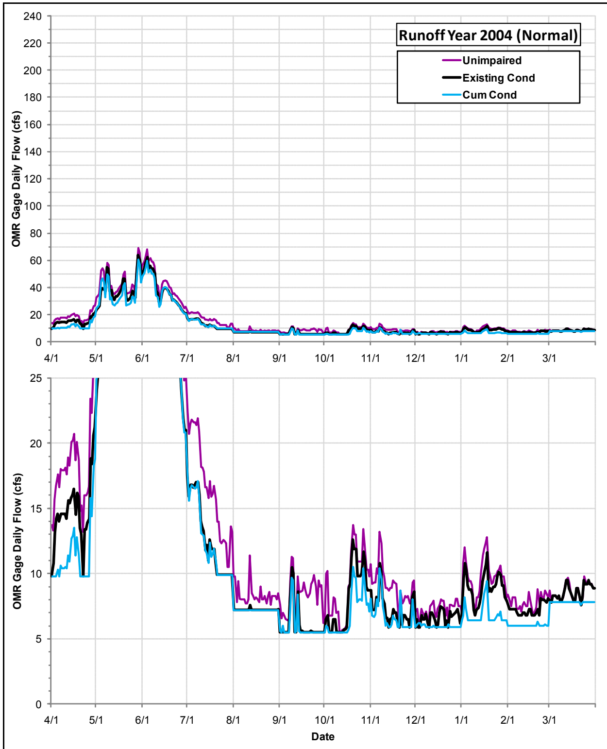
Daily Flows (cfs) at the OMR Gage under the Cumulative Condition, the Existing Condition and the Index of Unimpaired Conditions during Runoff Year 2004
