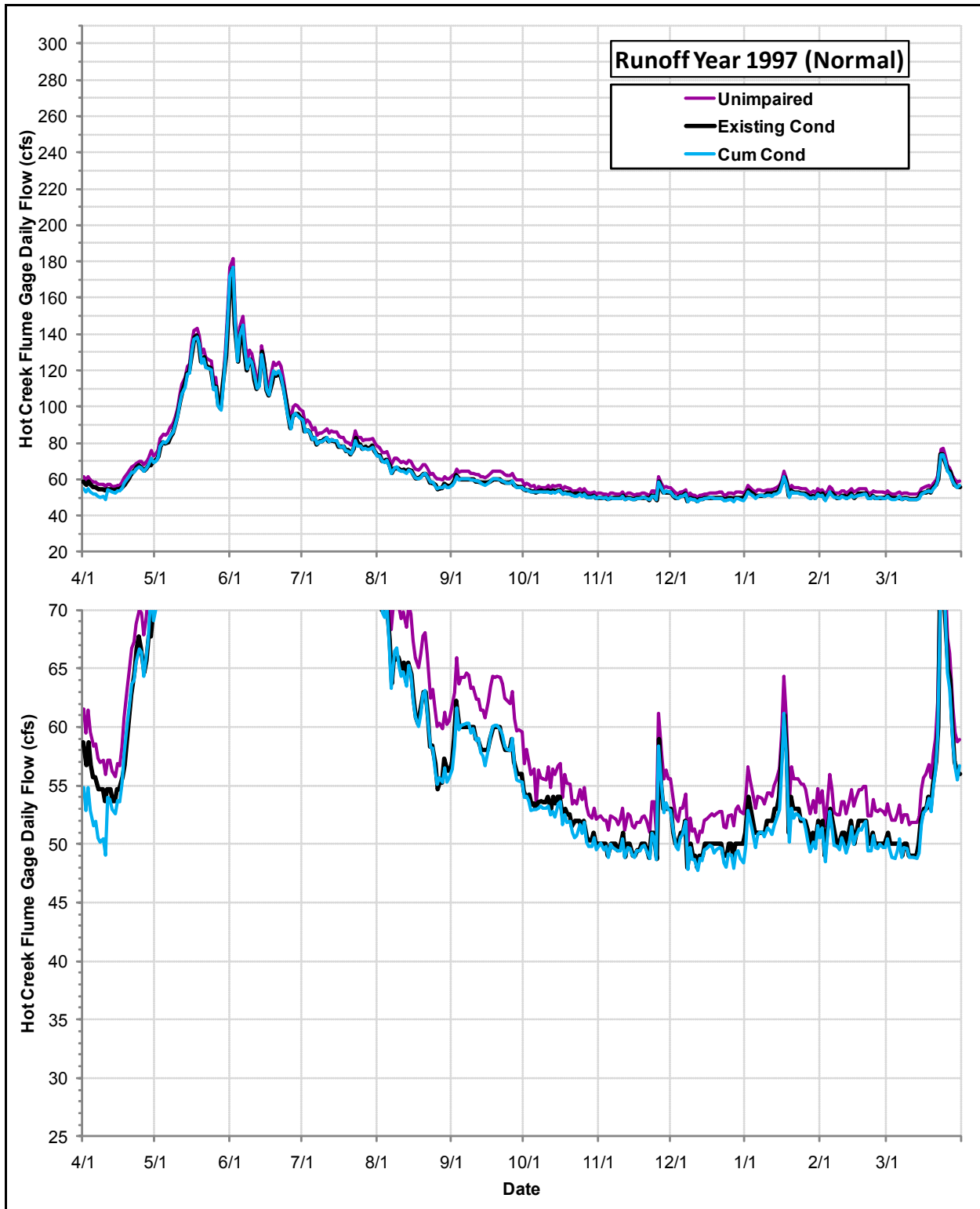
Daily Flows (cfs) at the USGS Hot Creek Flume Gage under the Cumulative Condition, the Existing Condition and the Index of Unimpaired Conditions during Runoff Year 1997
