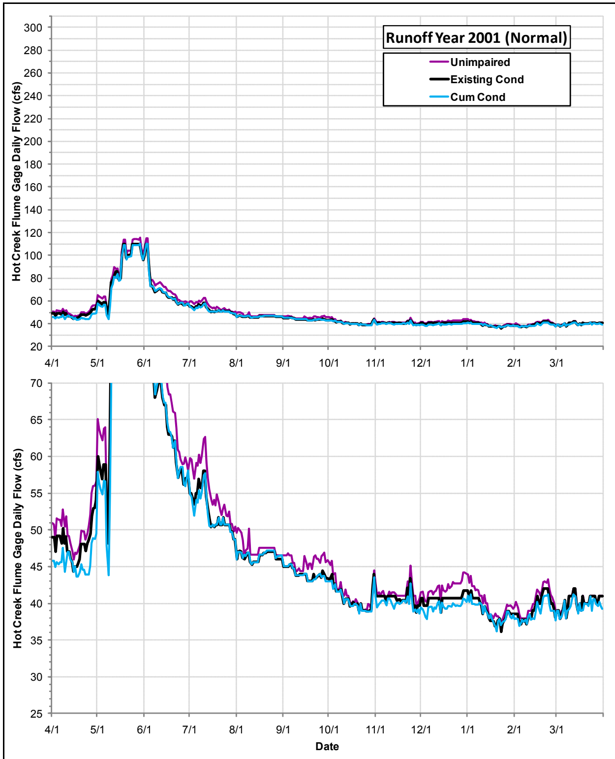
Daily Flows (cfs) at the USGS Hot Creek Flume Gage under the Cumulative Condition, the Existing Condition and the Index of Unimpaired Conditions during Runoff Year 2001
