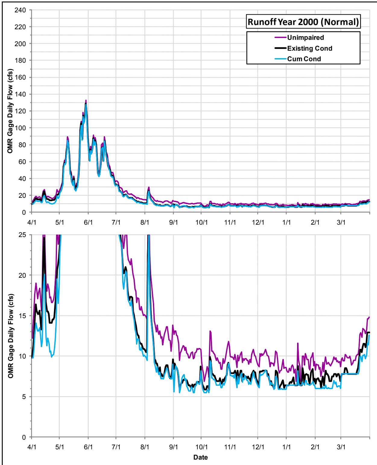
Daily Flows (cfs) at the OMR Gage under the Cumulative Condition, the Existing Condition and the Index of Unimpaired Conditions during Runoff Year 2000
