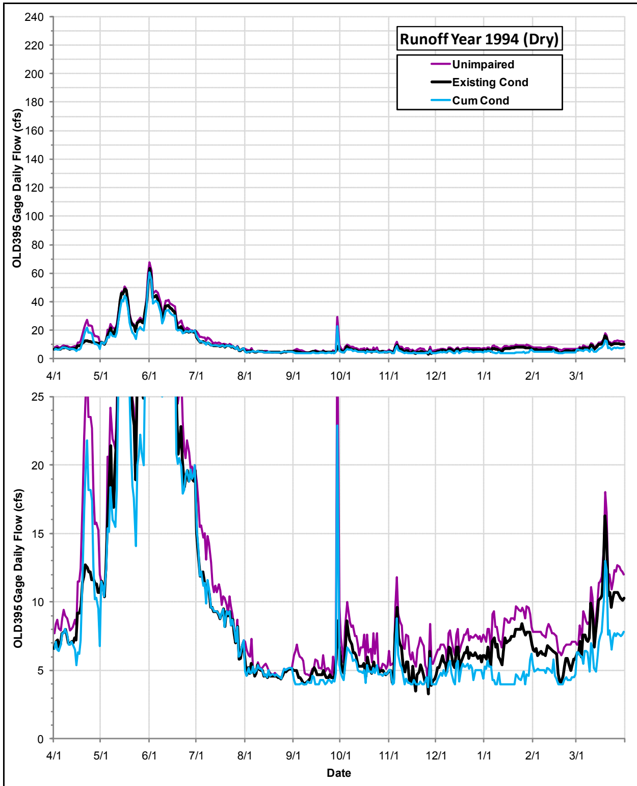
Daily Flows (cfs) at the OLD395 Gage under the Cumulative Condition, the Existing Condition and the Index of Unimpaired Conditions during Runoff Year 1994
