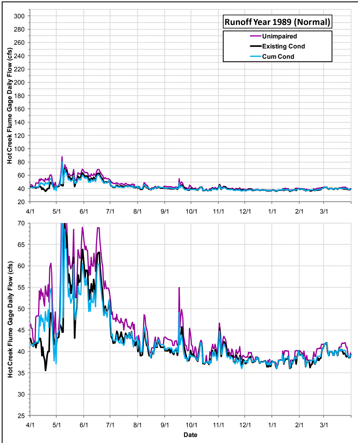
Daily Flows (cfs) at the USGS Hot Creek Flume Gage under the Cumulative Condition, the Existing Condition and the Index of Unimpaired Conditions during Runoff Year 1989
