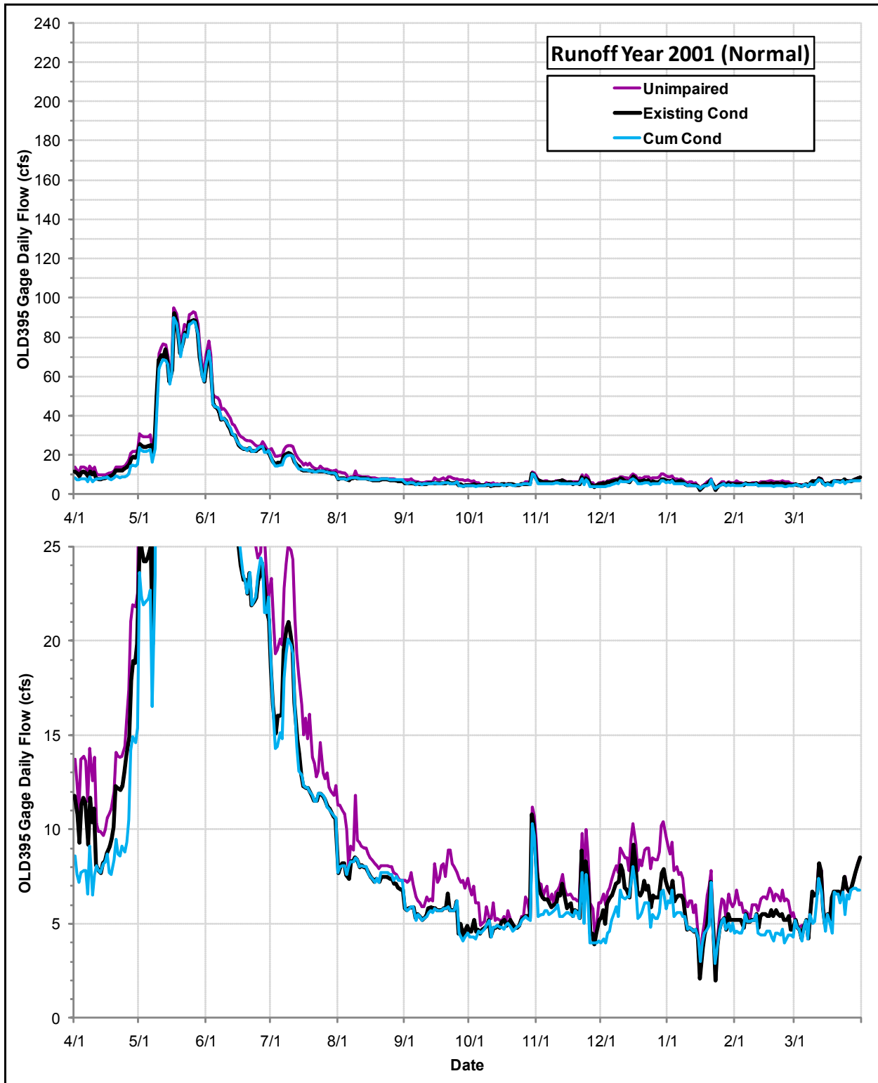
Daily Flows (cfs) at the OLD395 Gage under the Cumulative Condition, the Existing Condition and the Index of Unimpaired Conditions during Runoff Year 2001
