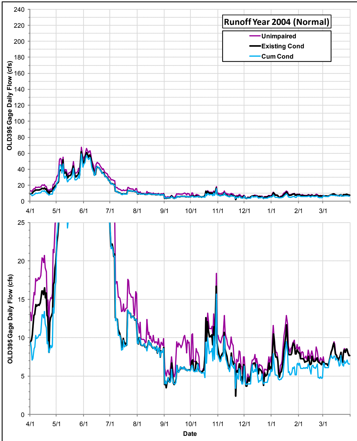
Daily Flows (cfs) at the OLD395 Gage under the Cumulative Condition, the Existing Condition and the Index of Unimpaired Conditions during Runoff Year 2004
