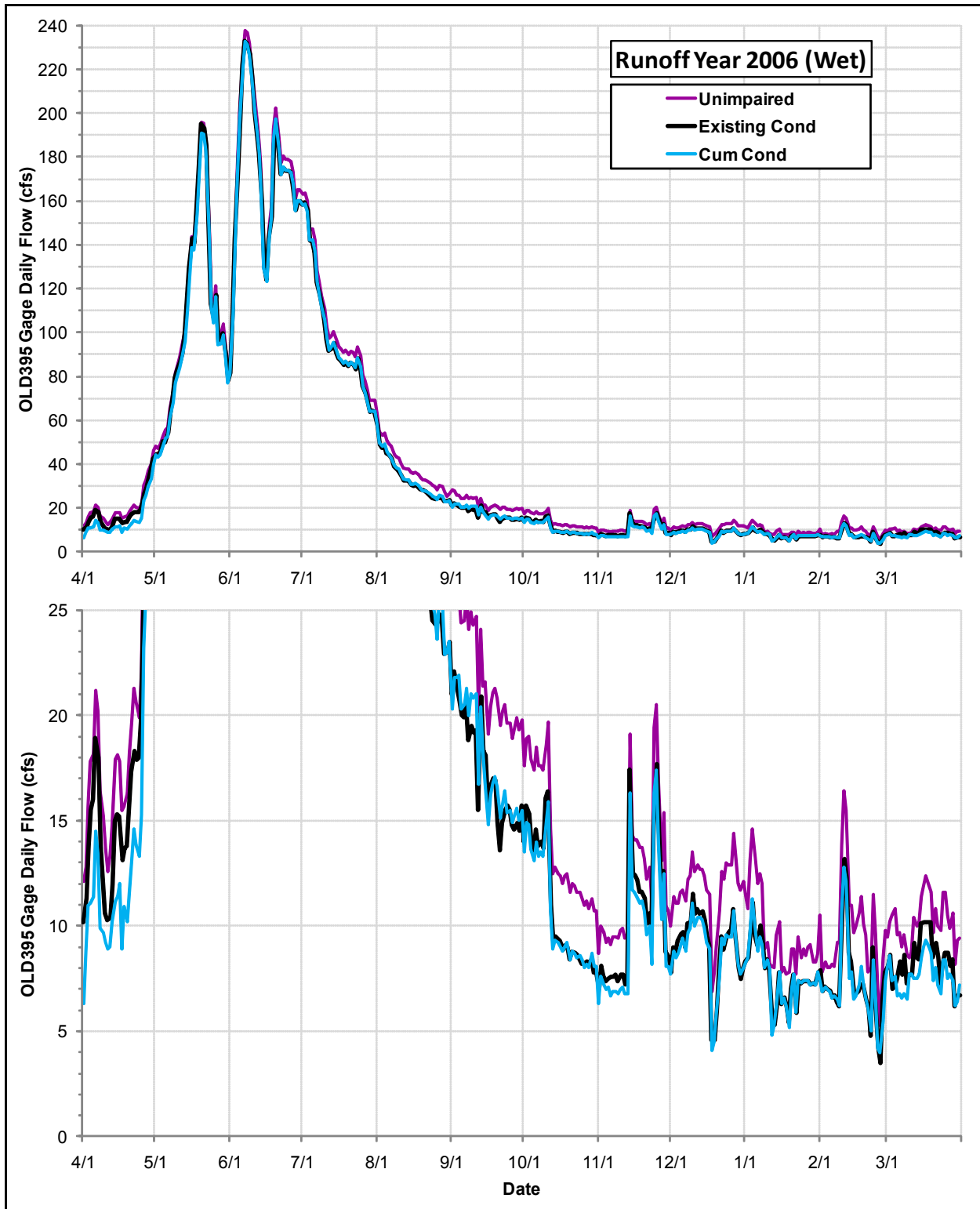
Daily Flows (cfs) at the OLD395 Gage under the Cumulative Condition, the Existing Condition and the Index of Unimpaired Conditions during Runoff Year 2006
