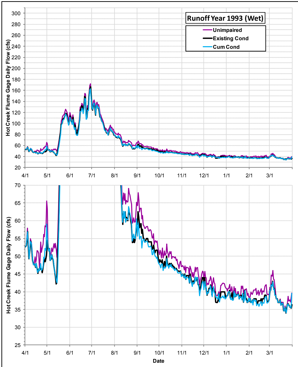
Daily Flows (cfs) at the USGS Hot Creek Flume Gage under the Cumulative Condition, the Existing Condition and the Index of Unimpaired Conditions during Runoff Year 1993
