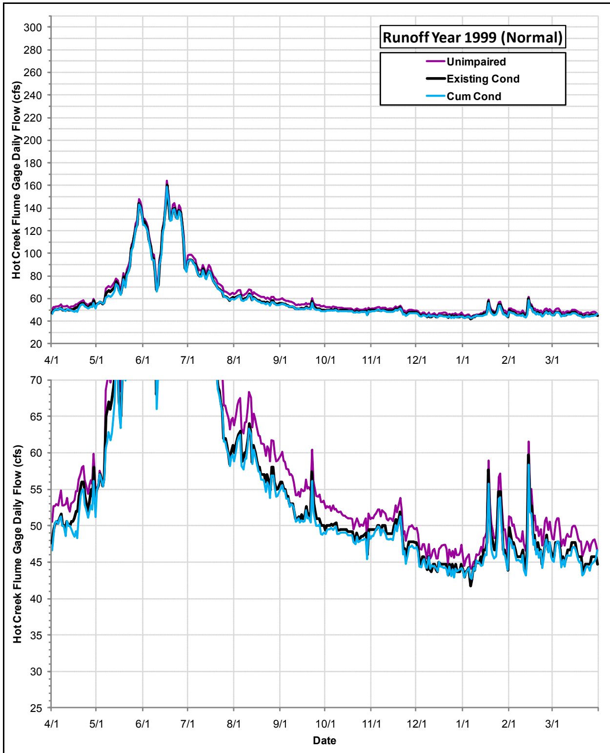
Daily Flows (cfs) at the USGS Hot Creek Flume Gage under the Cumulative Condition, the Existing Condition and the Index of Unimpaired Conditions during Runoff Year 1999
