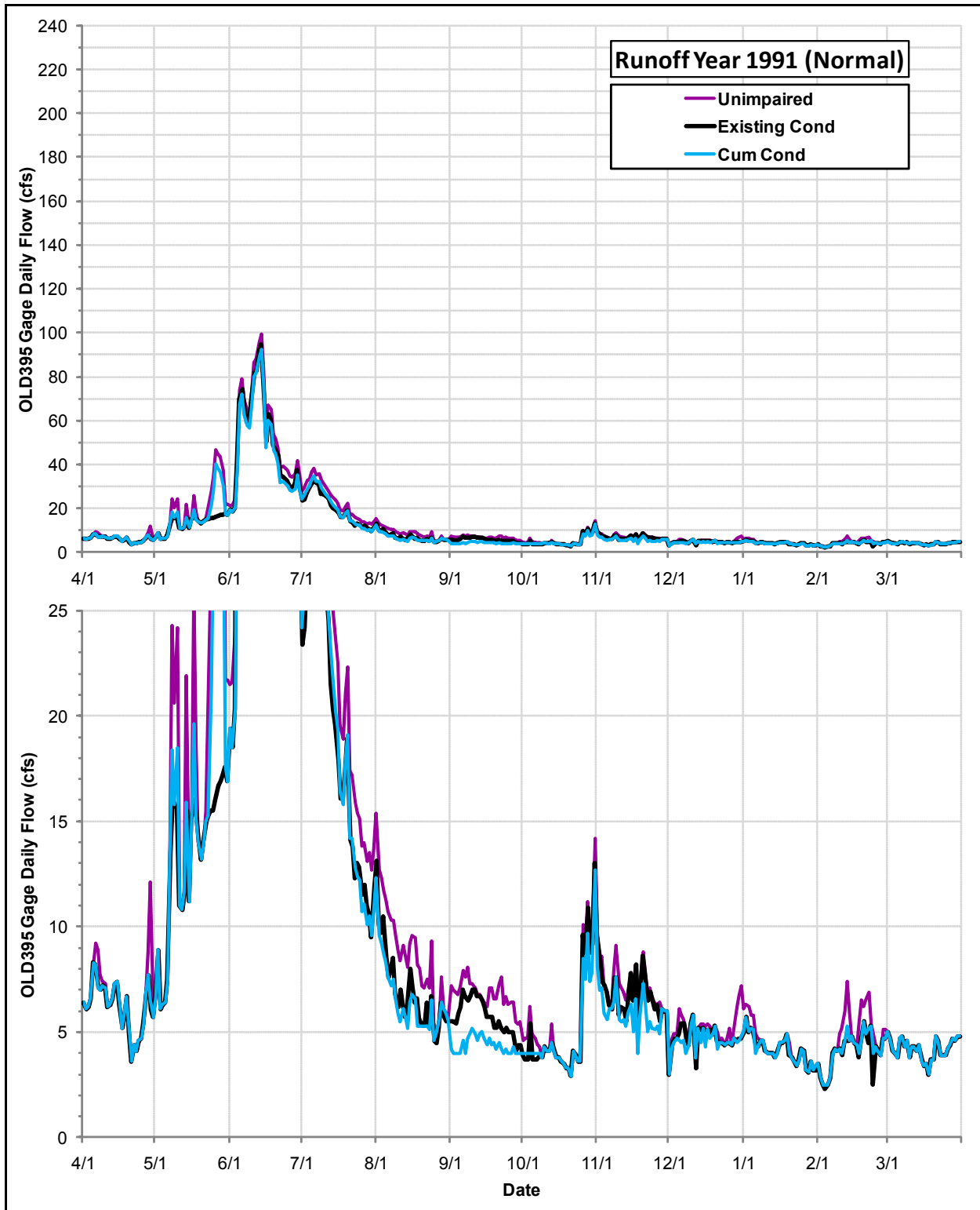
Daily Flows (cfs) at the OLD395 Gage under the Cumulative Condition, the Existing Condition and the Index of Unimpaired Conditions during Runoff Year 1991
