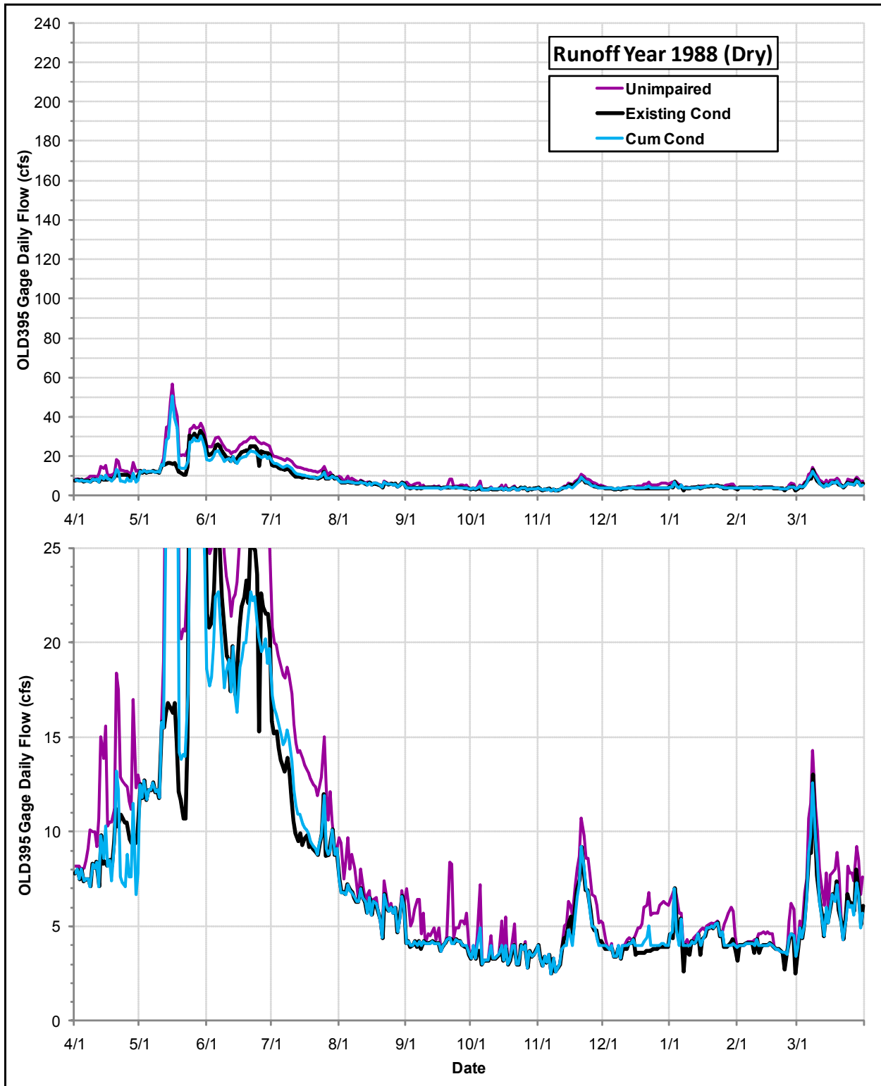
Daily Flows (cfs) at the OLD395 Gage under the Cumulative Condition, the Existing Condition and the Index of Unimpaired Conditions during Runoff Year 1988
