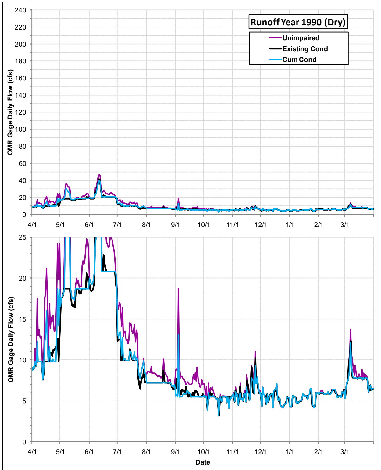
Daily Flows (cfs) at the OMR Gage under the Cumulative Condition, the Existing Condition and the Index of Unimpaired Conditions during Runoff Year 1990
