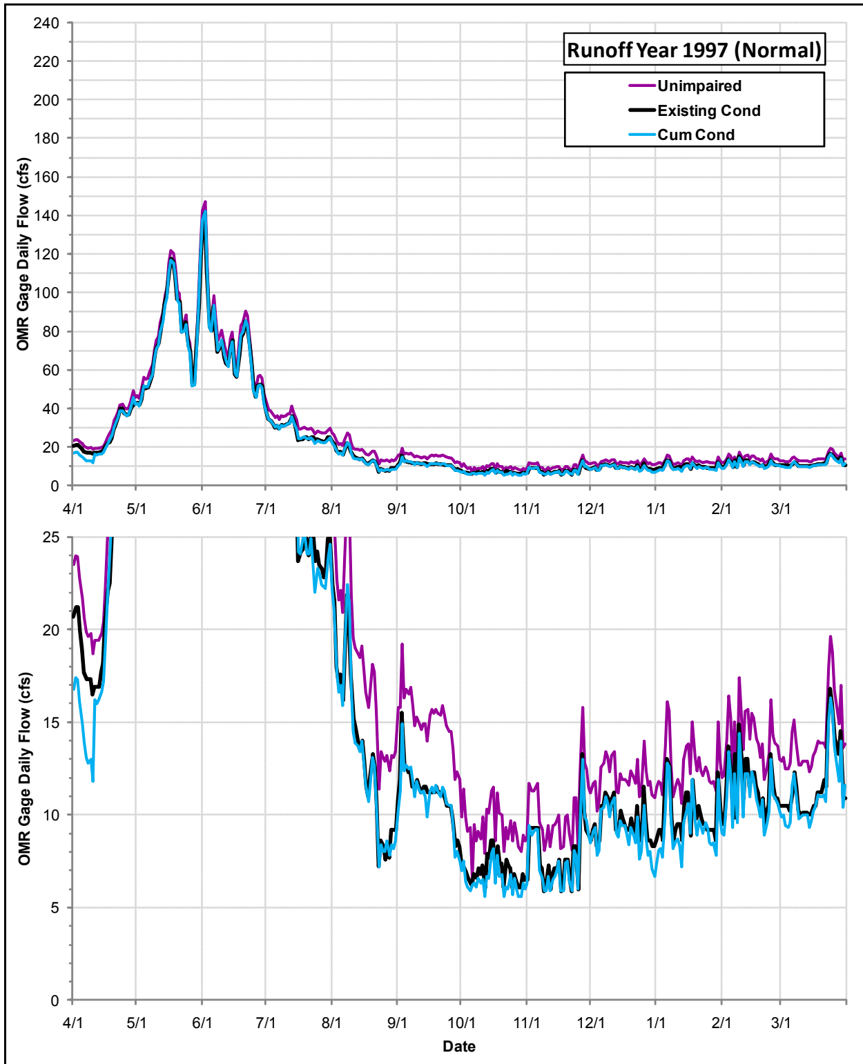
Daily Flows (cfs) at the OMR Gage under the Cumulative Condition, the Existing Condition and the Index of Unimpaired Conditions during Runoff Year 1997
