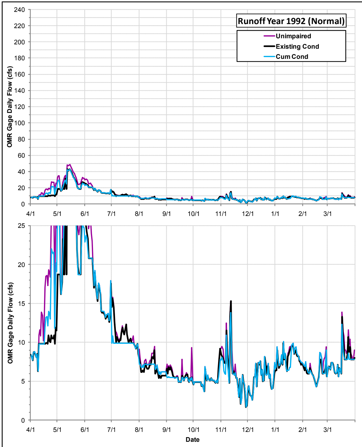
Daily Flows (cfs) at the OMR Gage under the Cumulative Condition, the Existing Condition and the Index Unimpaired Conditions during Runoff Year 1992
