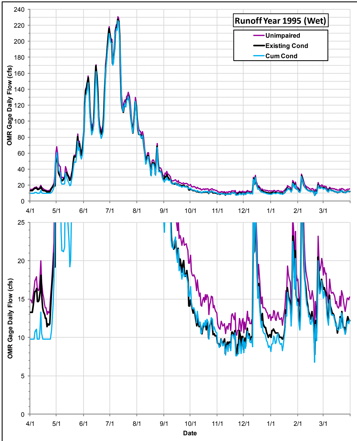
Daily Flows (cfs) at the OMR Gage under the Cumulative Condition, the Existing Condition and the Index of Unimpaired Conditions during Runoff Year 1995
