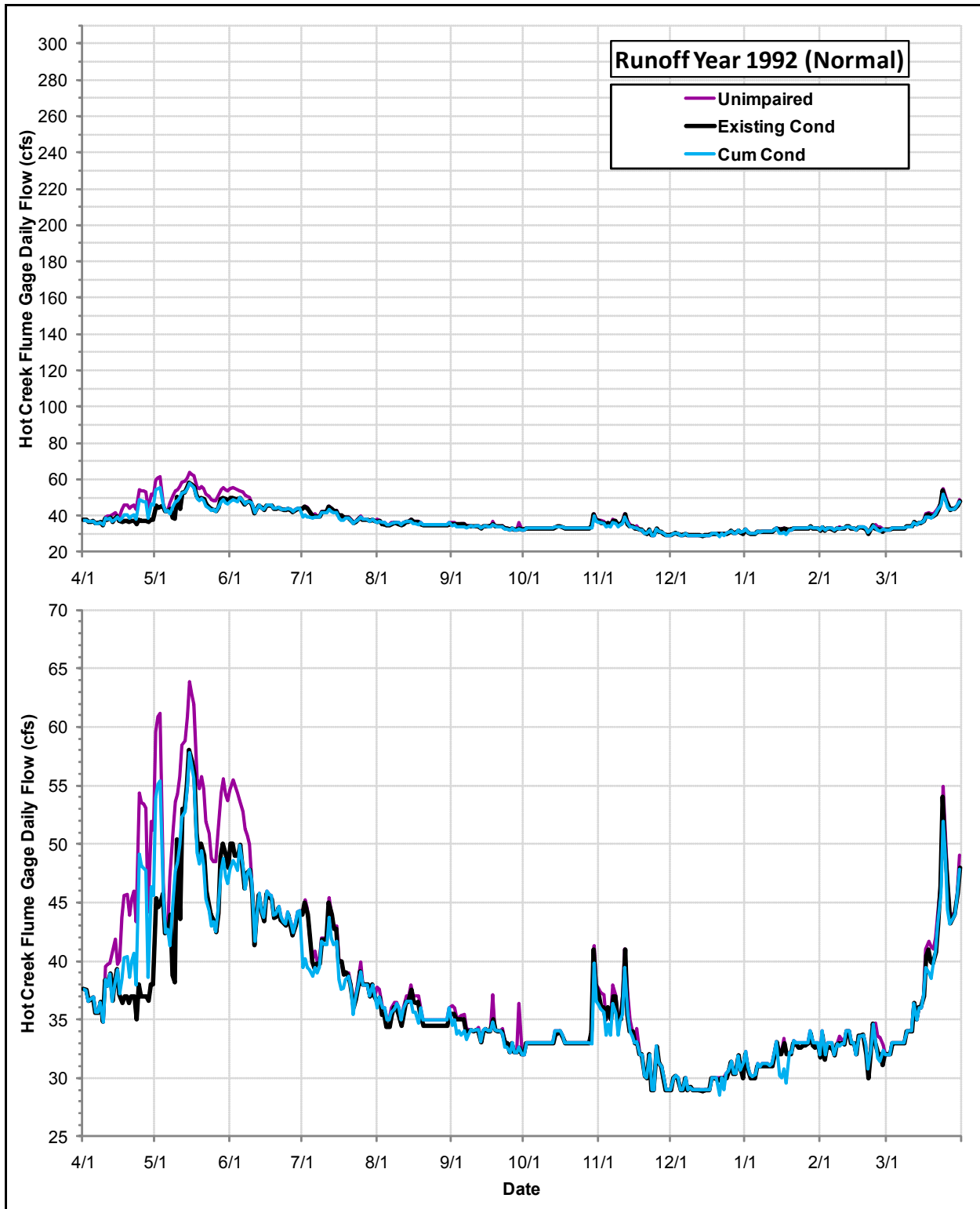
Daily Flows (cfs) at the USGS Hot Creek Flume Gage under the Cumulative Condition, the Existing Condition and the Index of Unimpaired Conditions during Runoff Year 1992
