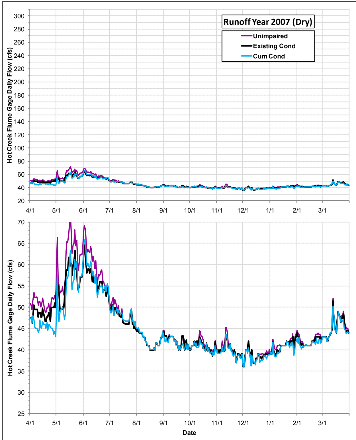
Daily Flows (cfs) at the USGS Hot Creek Flume Gage under the Cumulative Condition, the Existing Condition and the Index of Unimpaired Conditions during Runoff Year 2007
