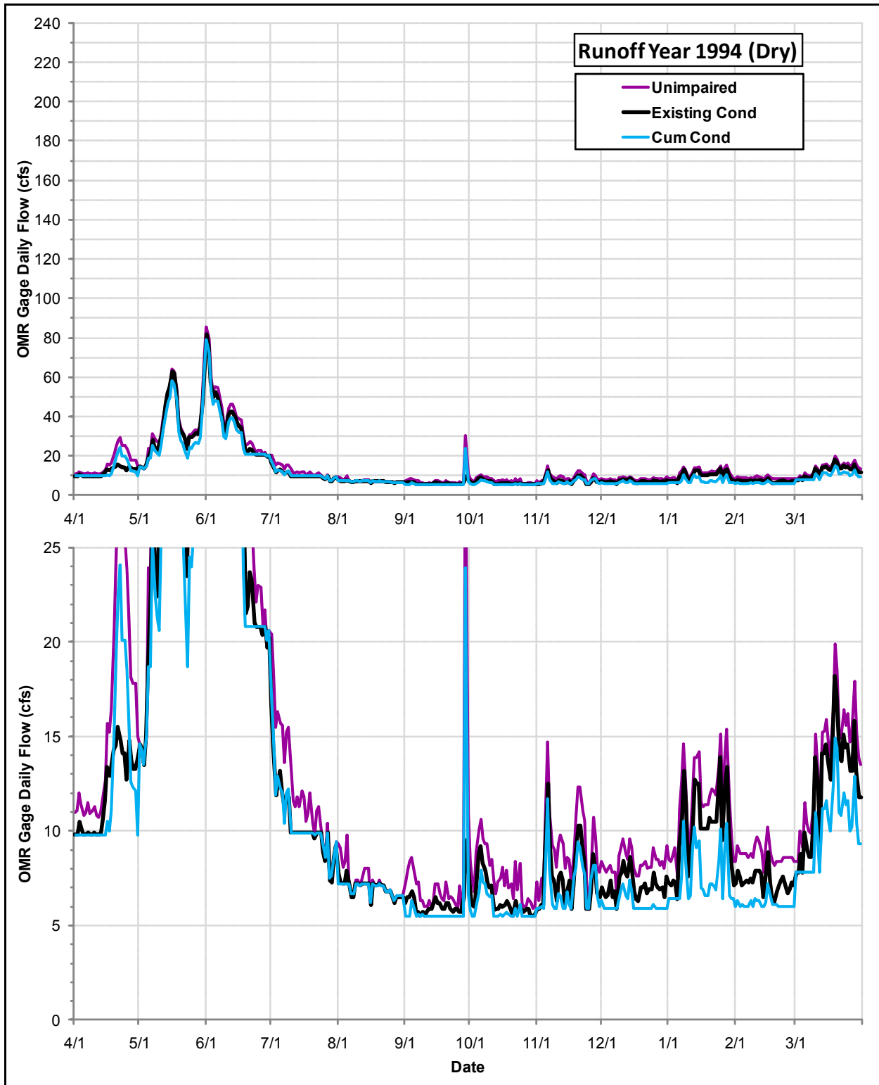
Daily Flows (cfs) at the OMR Gage under the Cumulative Condition, the Existing Condition and the Index of Unimpaired Conditions during Runoff Year 1994
