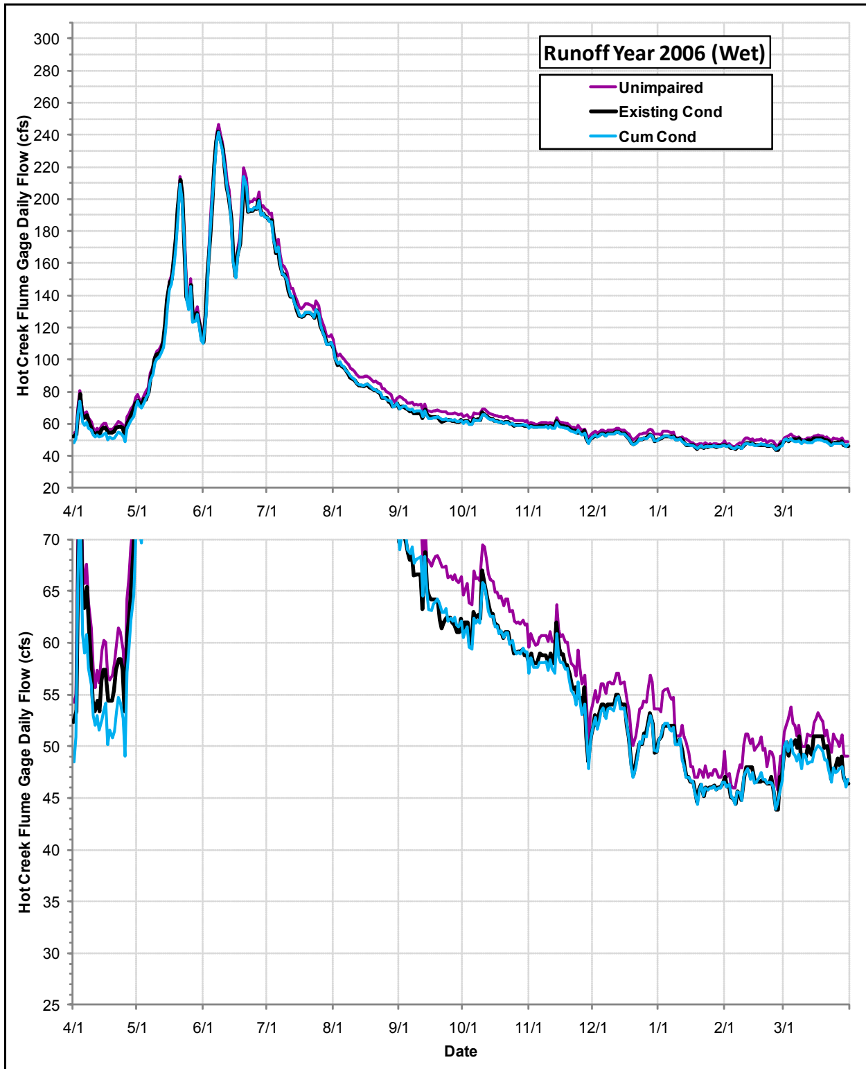
Daily Flows (cfs) at the USGS Hot Creek Flume Gage under the Cumulative Condition, the Existing Condition and the Index of Unimpaired Conditions during Runoff Year 2006
