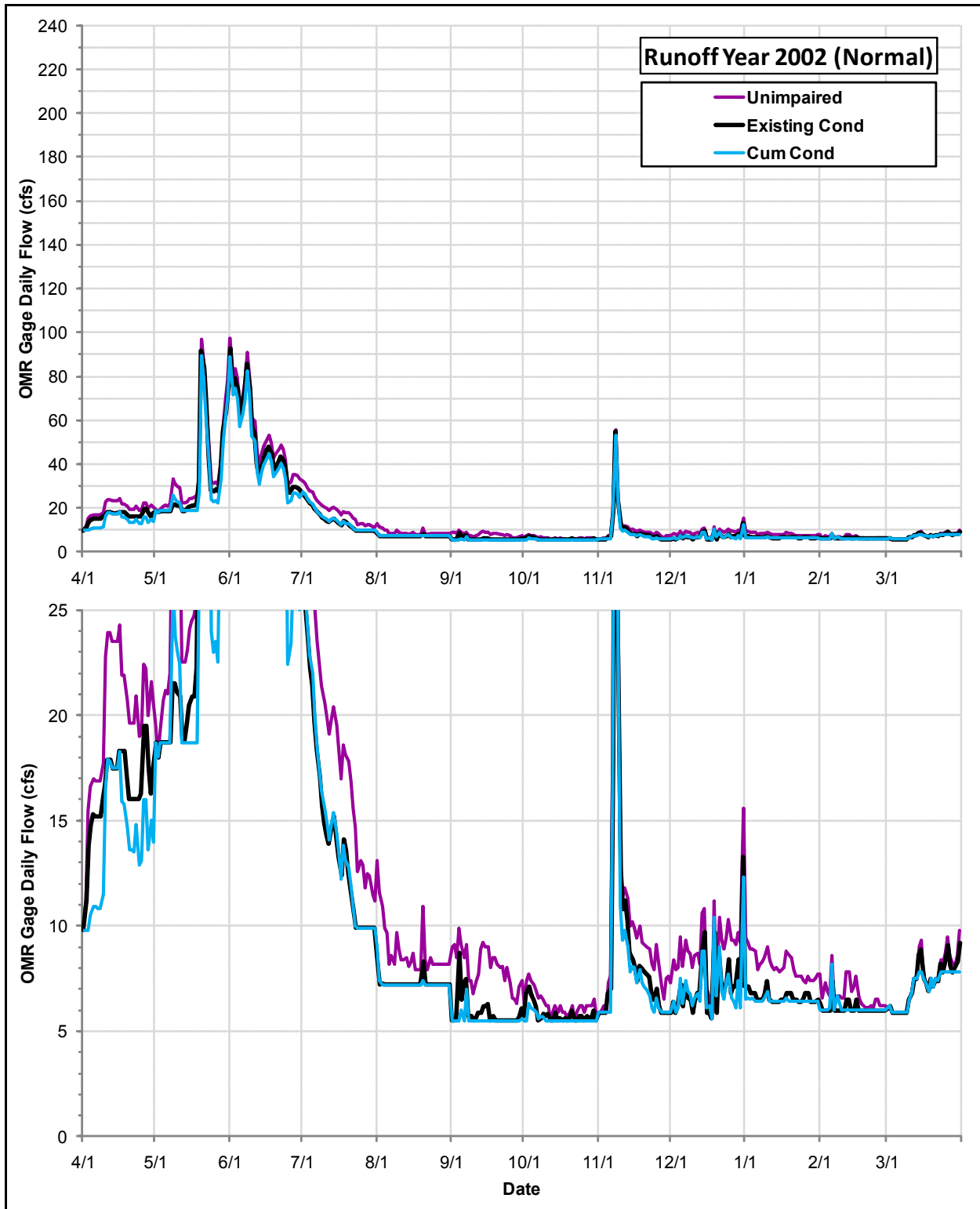
Daily Flows (cfs) at the OMR Gage under the Cumulative Condition, the Existing Condition and the Index of Unimpaired Conditions during Runoff Year 2002
