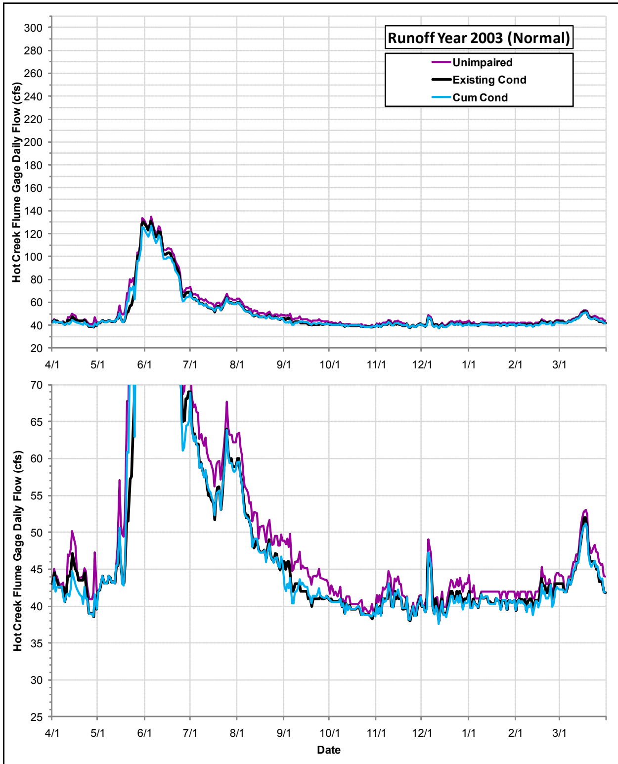
Daily Flows (cfs) at the USGS Hot Creek Flume Gage under the Cumulative Condition, the Existing Condition and the Index of Unimpaired Conditions during Runoff Year 2003
