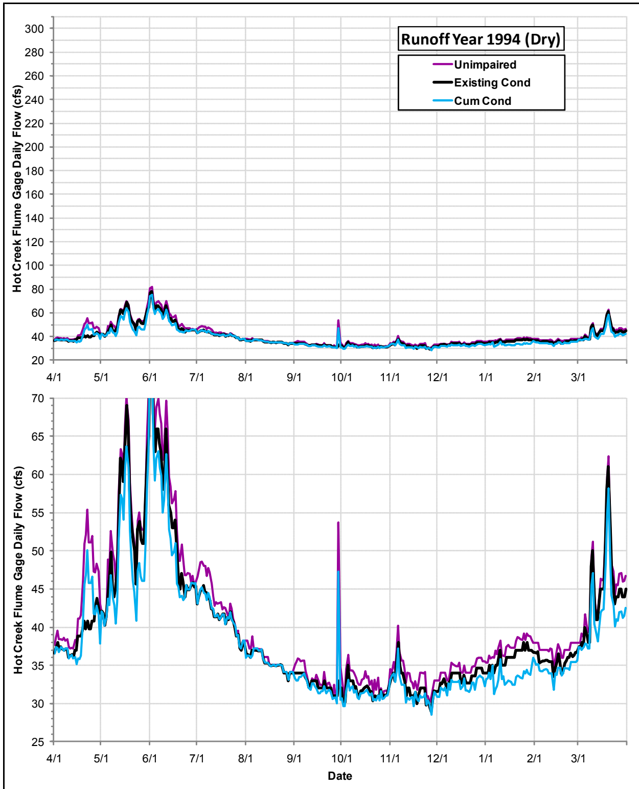
Daily Flows (cfs) at the USGS Hot Creek Flume Gage under the Cumulative Condition, the Existing Condition and the Index of Unimpaired Conditions during Runoff Year 1994
