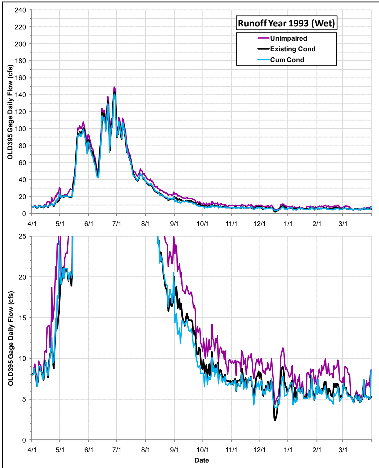
Daily Flows (cfs) at the OLD395 Gage under the Cumulative Condition, the Existing Condition and the Index of Unimpaired Conditions during Runoff Year 1993
