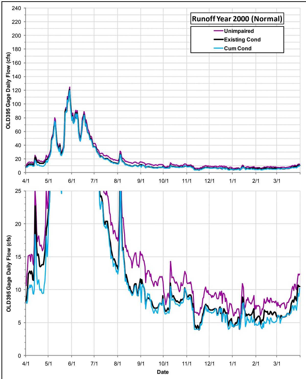
Daily Flows (cfs) at the OLD395 Gage under the Cumulative Condition, the Existing Condition and the Index of Unimpaired Conditions during Runoff Year 2000
