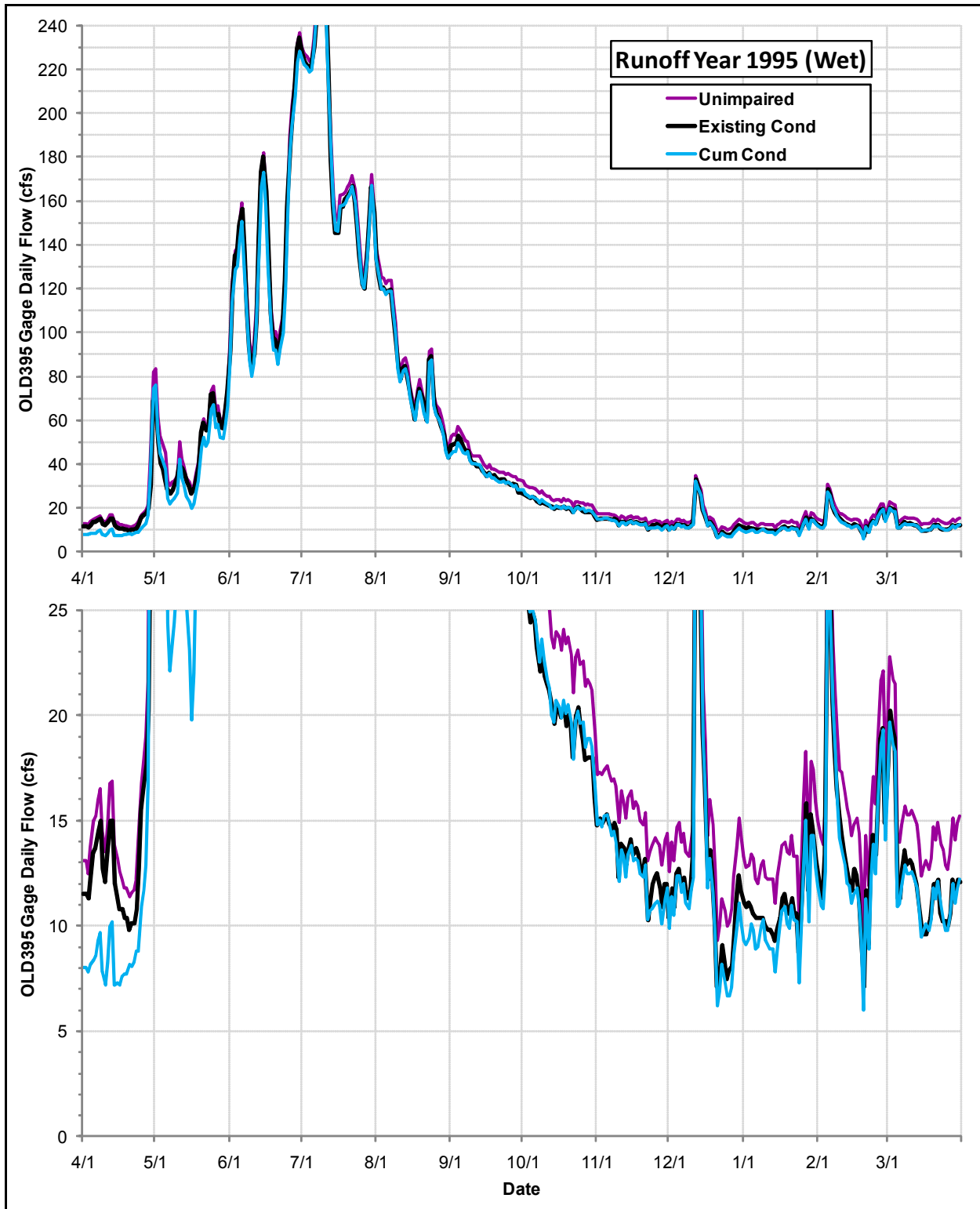
Daily Flows (cfs) at the OLD395 Gage under the Cumulative Condition, the Existing Condition and the Index of Unimpaired Conditions during Runoff Year 1995
