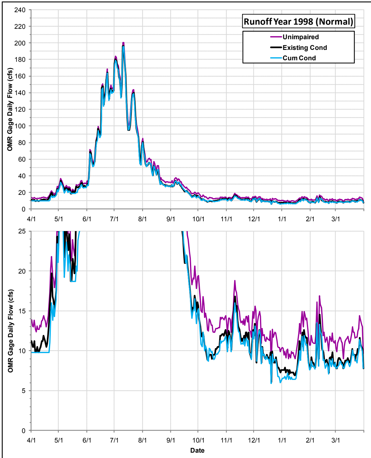
Daily Flows (cfs) at the OMR Gage under the Cumulative Condition, the Existing Condition and the Index of Unimpaired Conditions during Runoff Year 1998
