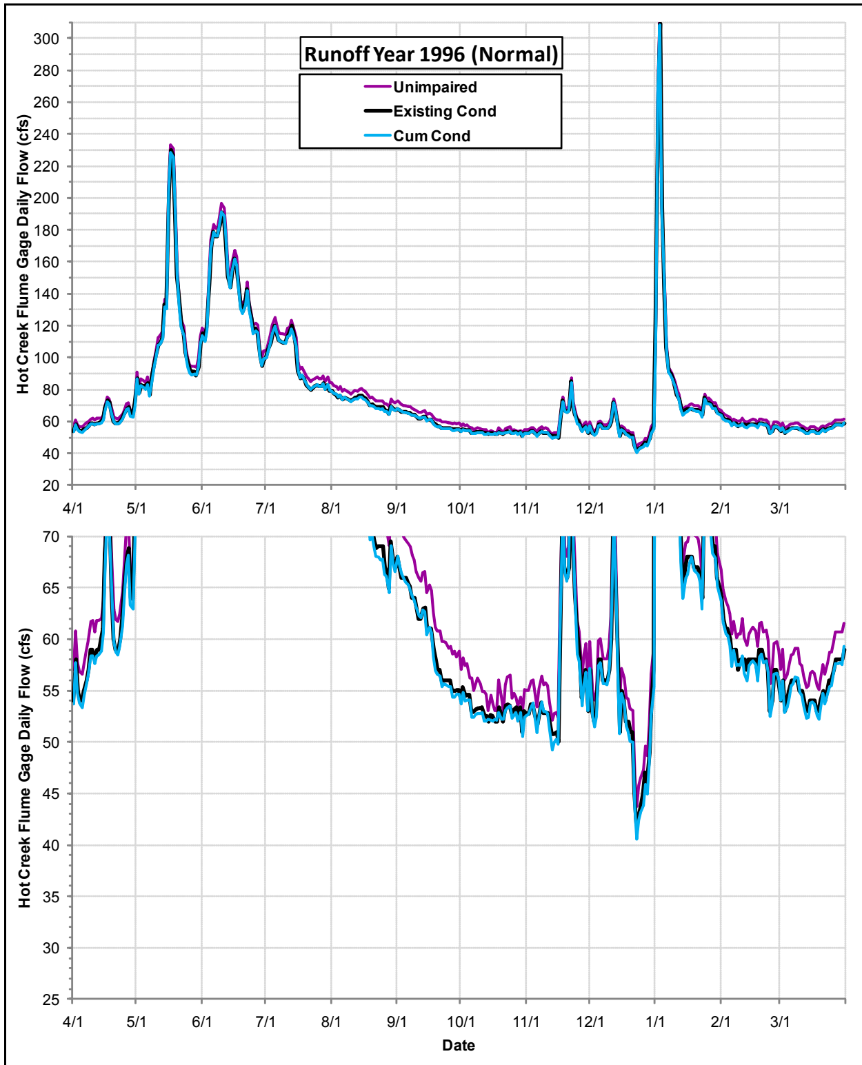
Daily Flows (cfs) at the USGS Hot Creek Flume Gage under the Cumulative Condition, the Existing Condition and the Index of Unimpaired Conditions during Runoff Year 1996
