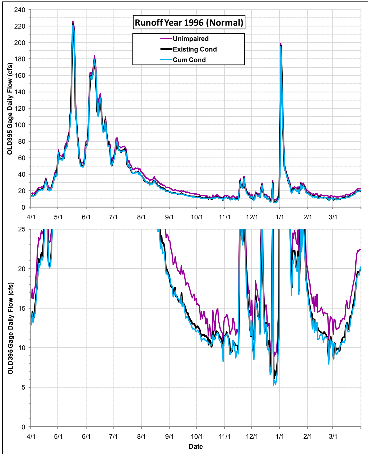
Daily Flows (cfs) at the OLD395 Gage under the Cumulative Condition, the Existing Condition and the Index of Unimpaired Conditions during Runoff Year 1996
