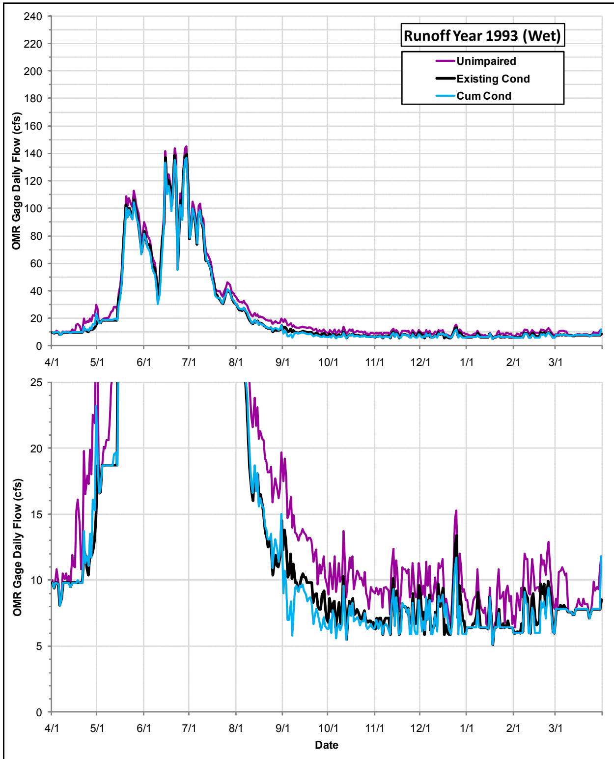
Daily Flows (cfs) at the OMR Gage under the Cumulative Condition, the Existing Condition and the Index of Unimpaired Conditions during Runoff Year 1993
