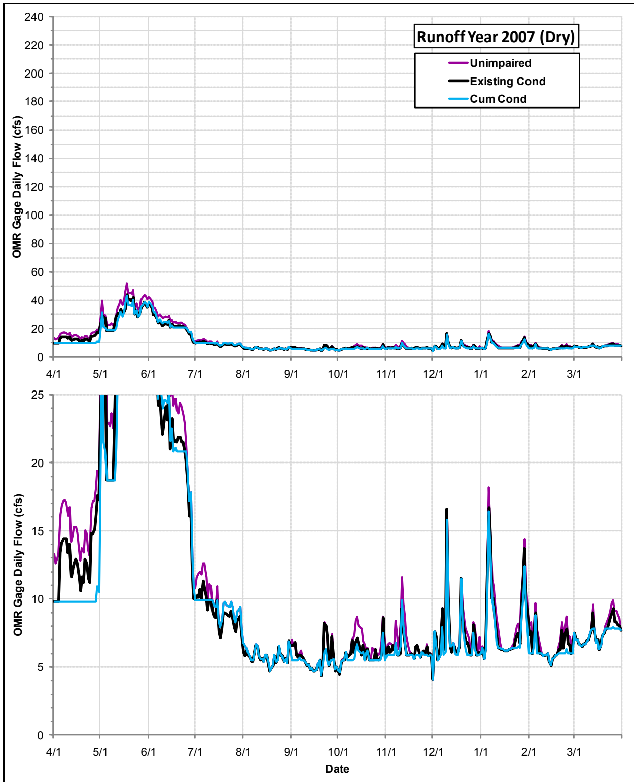
Daily Flows (cfs) at the OMR Gage under the Cumulative Condition, the Existing Condition and the Index of Unimpaired Conditions during Runoff Year 2007
