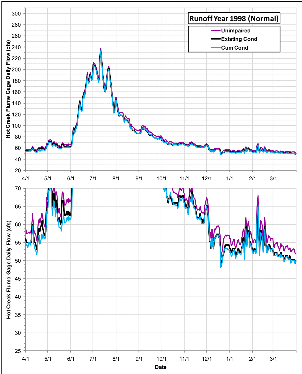
Daily Flows (cfs) at the USGS Hot Creek Flume Gage under the Cumulative Condition, the Existing Condition and the Index of Unimpaired Conditions during Runoff Year 1998
