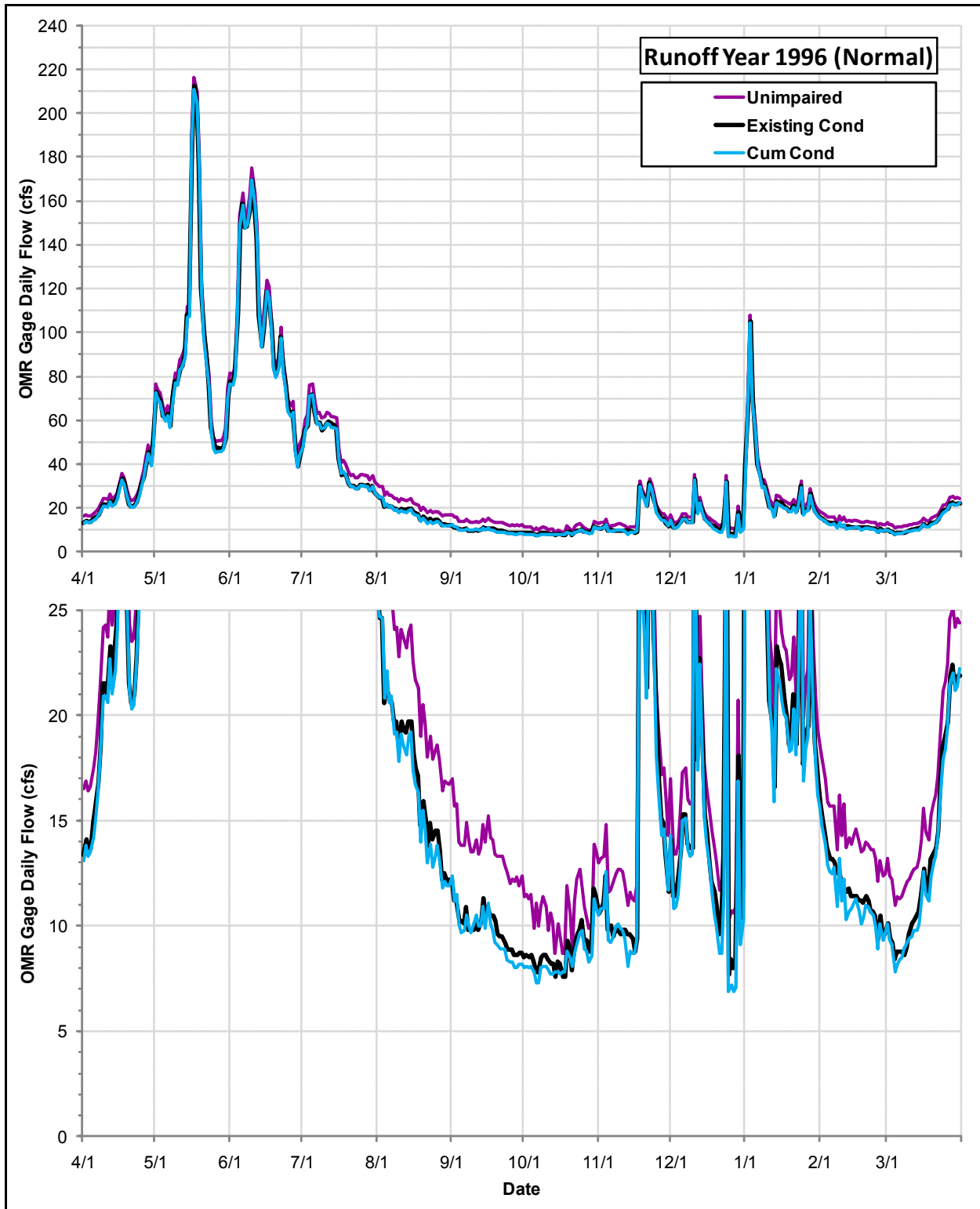
Daily Flows (cfs) at the OMR Gage under the Cumulative Condition, the Existing Condition and the Index of Unimpaired Conditions during Runoff Year 1996
