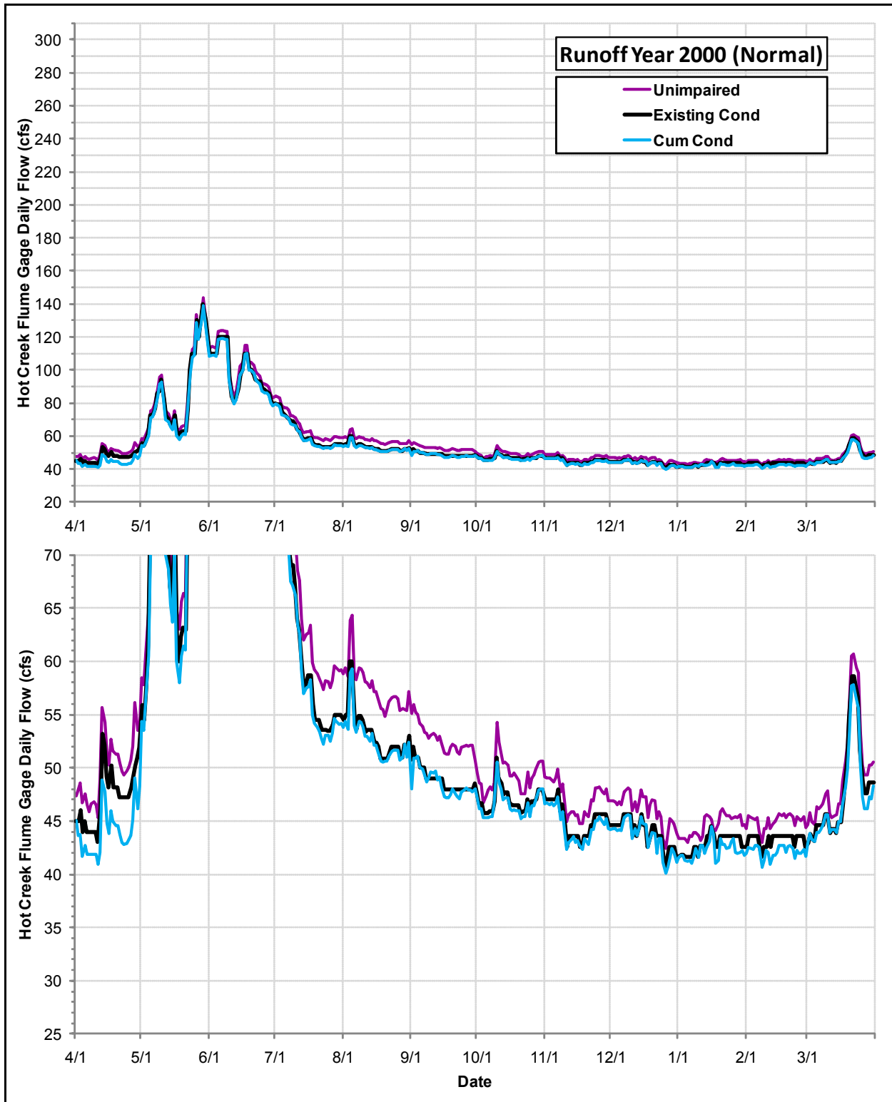
Daily Flows (cfs) at the USGS Hot Creek Flume Gage under the Cumulative Condition, the Existing Condition and the Index of Unimpaired Conditions during Runoff Year 2000
