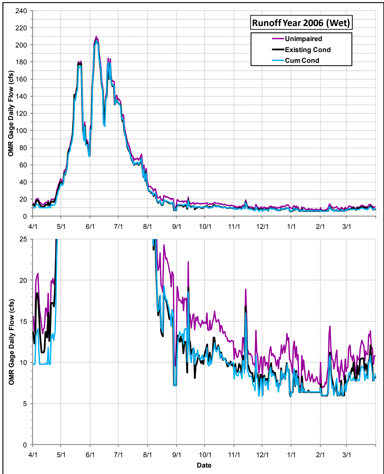
Daily Flows (cfs) at the OMR Gage under the Cumulative Condition, the Existing Condition and the Index of Unimpaired Conditions during Runoff Year 2006
