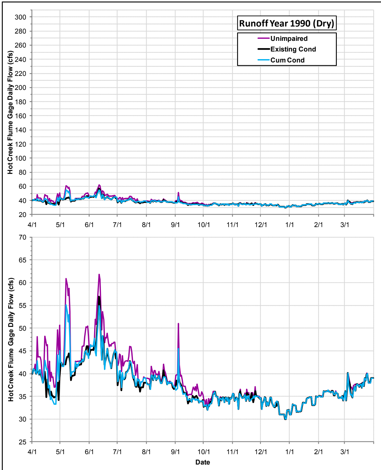
Daily Flows (cfs) at the USGS Hot Creek Flume Gage under the Cumulative Condition, the Existing Condition and the Index of Unimpaired Conditions during Runoff Year 1990
