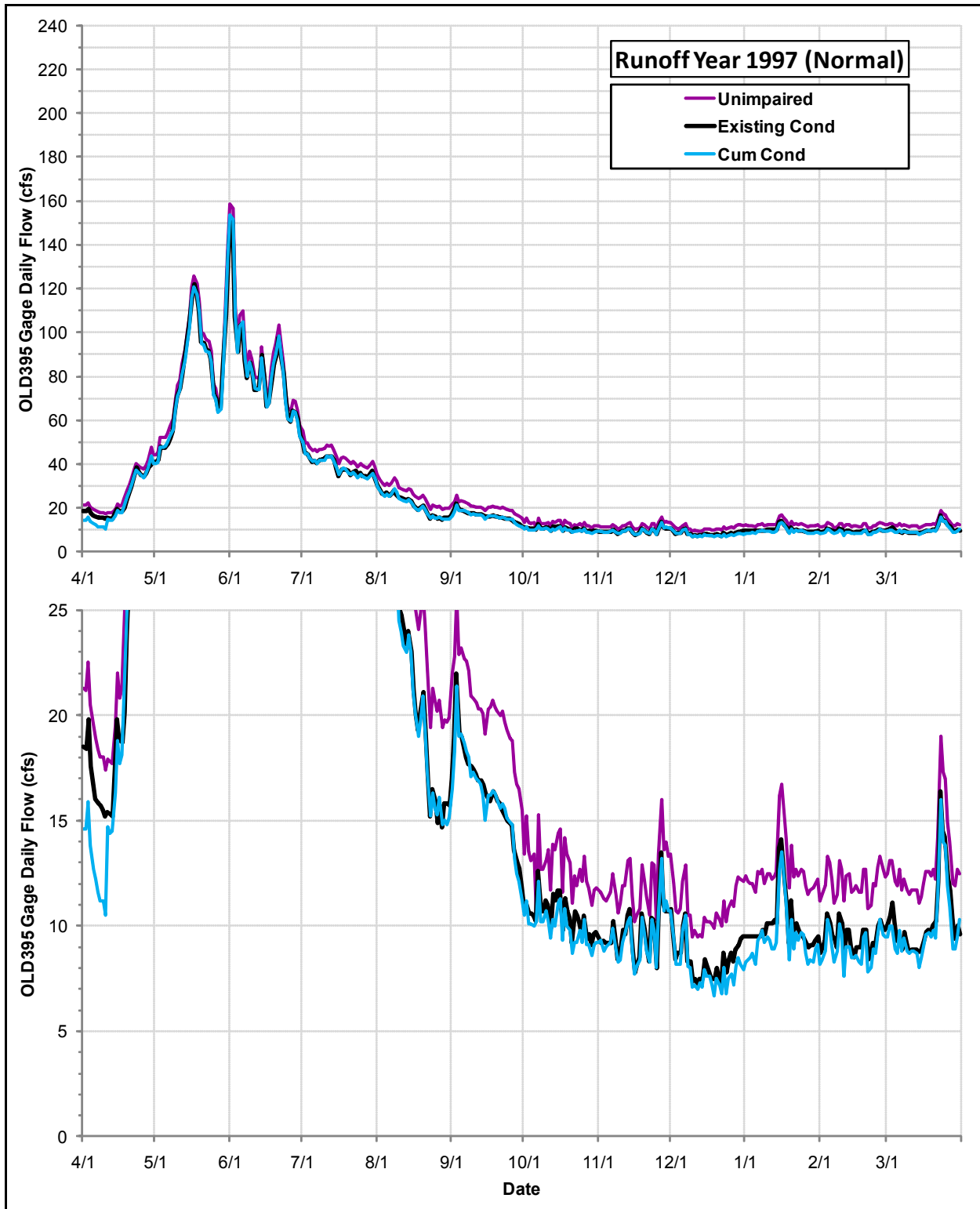
Daily Flows (cfs) at the OLD395 Gage under the Cumulative Condition, the Existing Condition and the Index of Unimpaired Conditions during Runoff Year 1997
