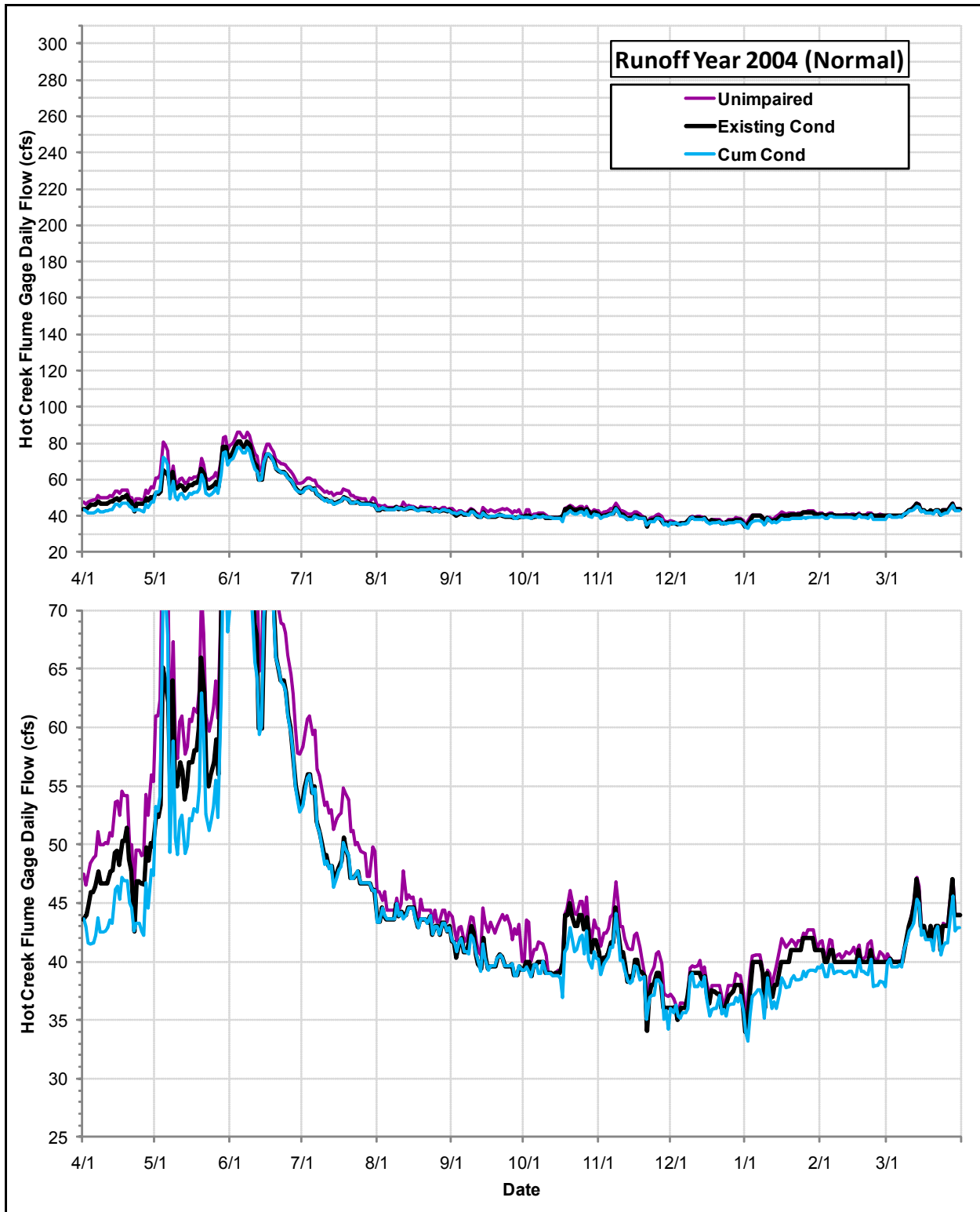
Daily Flows (cfs) at the USGS Hot Creek Flume Gage under the Cumulative Condition, the Existing Condition and the Index of Unimpaired Conditions during Runoff Year 2004
