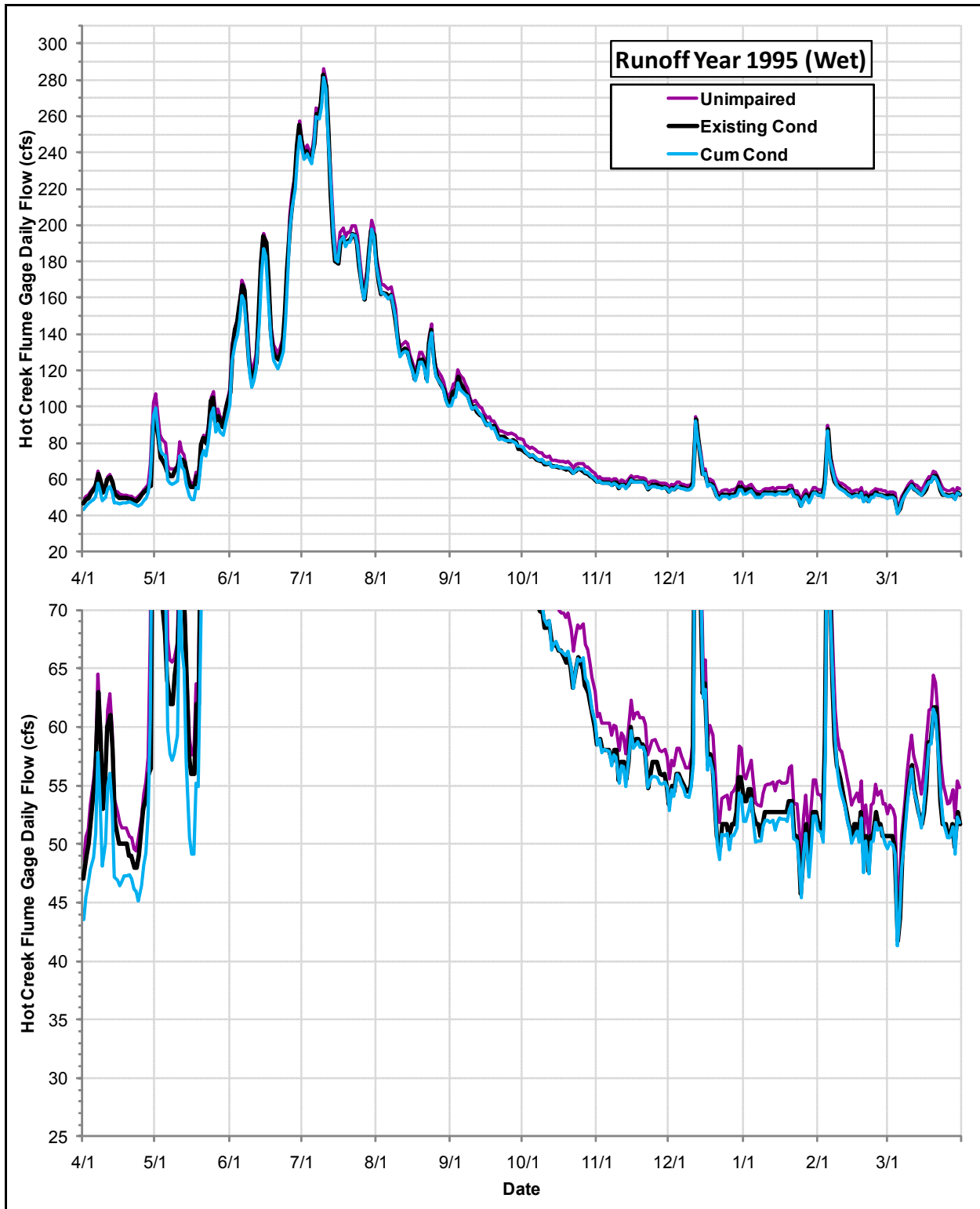
Daily Flows (cfs) at the USGS Hot Creek Flume Gage under the Cumulative Condition, the Existing Condition and the Index of Unimpaired Conditions during Runoff Year 1995
