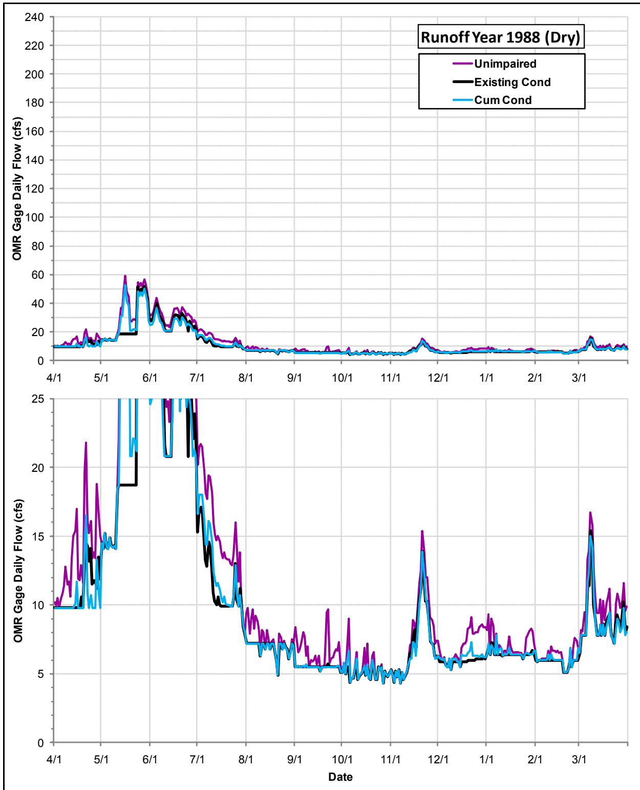
Daily Flows (cfs) at the OMR Gage under the Cumulative Condition, the Existing Condition and the Index of Unimpaired Conditions during Runoff Year 1988
