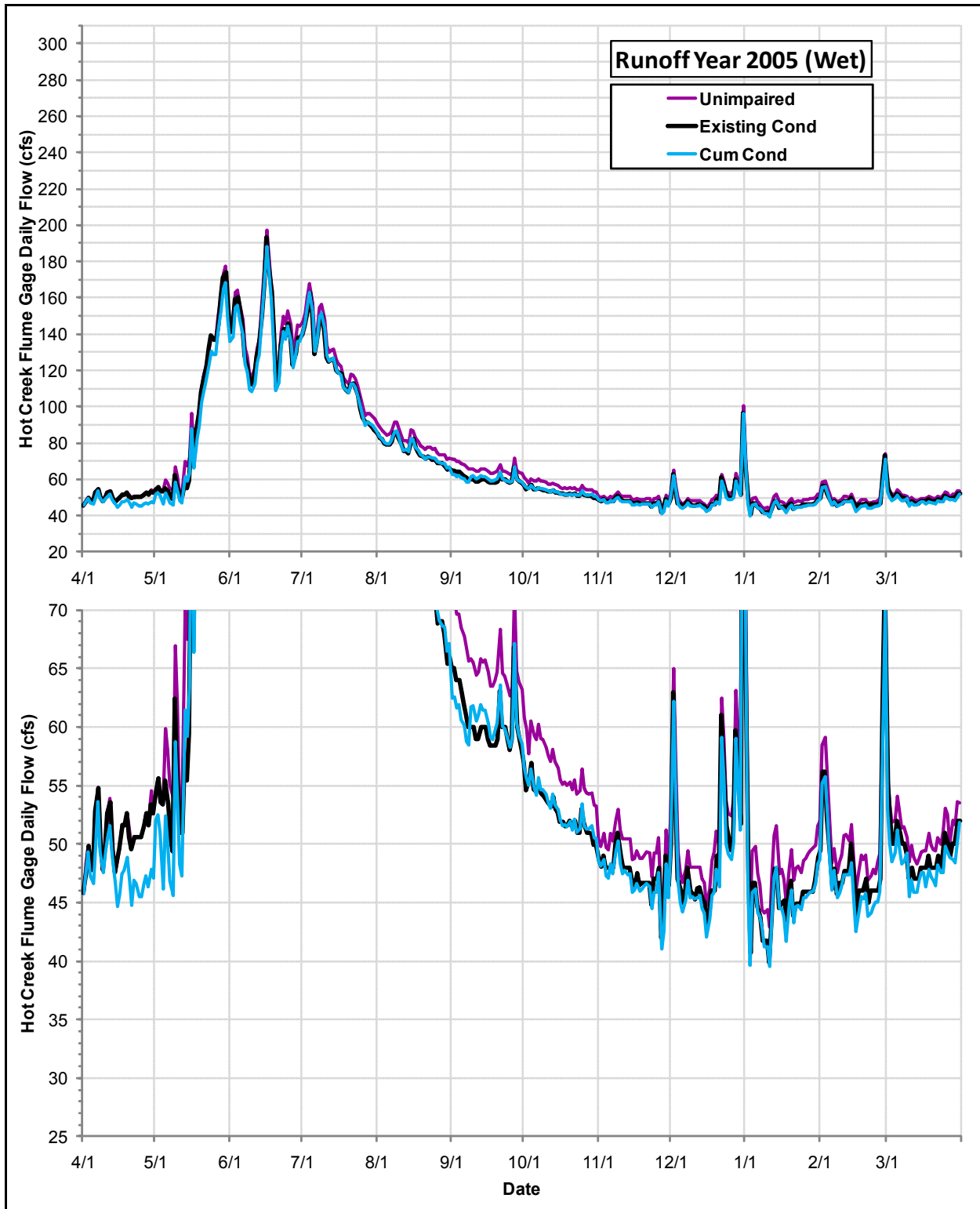
Daily Flows (cfs) at the USGS Hot Creek Flume Gage under the Cumulative Condition, the Existing Condition and the Index of Unimpaired Conditions during Runoff Year 2005
