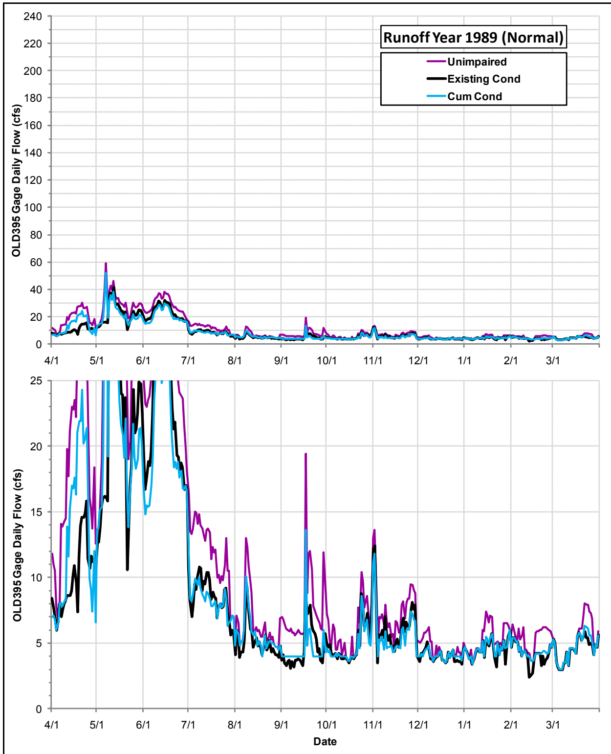
Daily Flows (cfs) at the OLD395 Gage under the Cumulative Condition, the Existing Condition and the Index of Unimpaired Conditions during Runoff Year 1989
