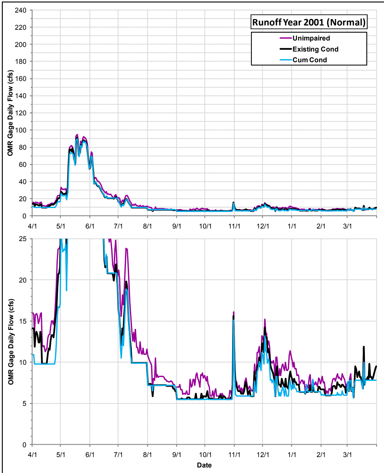
Daily Flows (cfs) at the OMR Gage under the Cumulative Condition, the Existing Condition and the Index of Unimpaired Conditions during Runoff Year 2001
