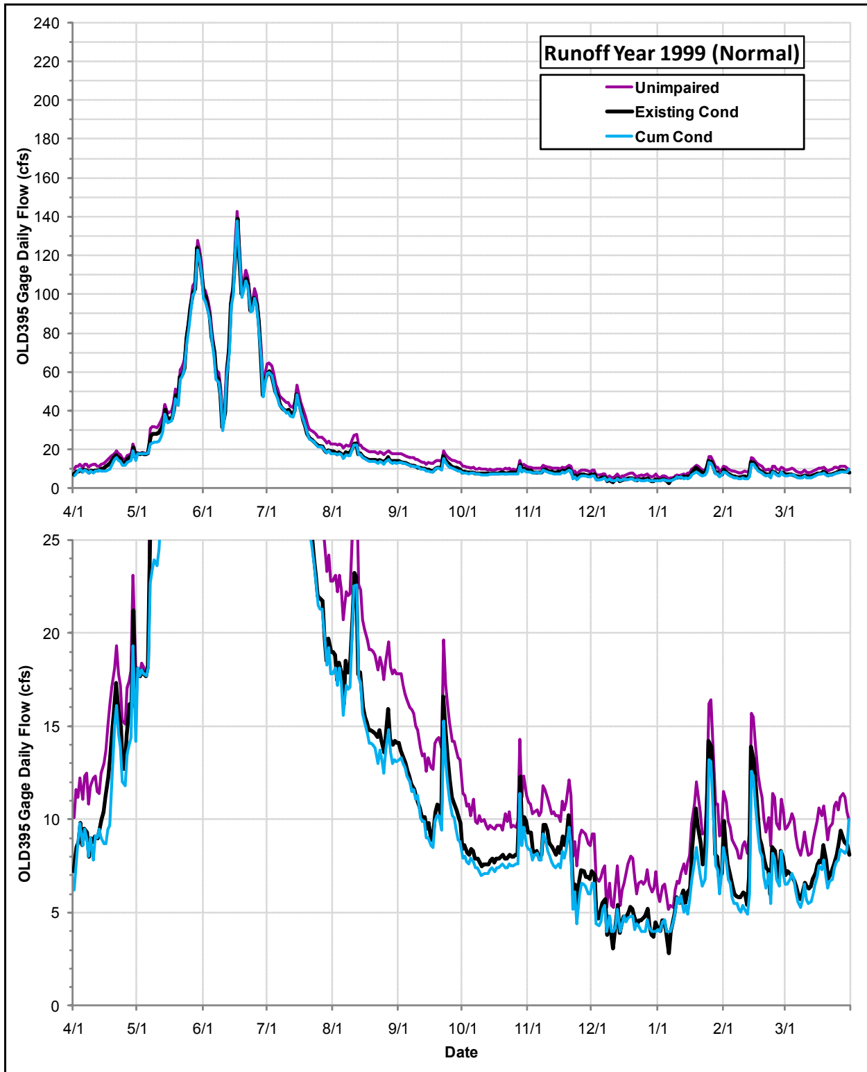
Daily Flows (cfs) at the OLD395 Gage under the Cumulative Condition, the Existing Condition and the Index of Unimpaired Conditions during Runoff Year 1999
