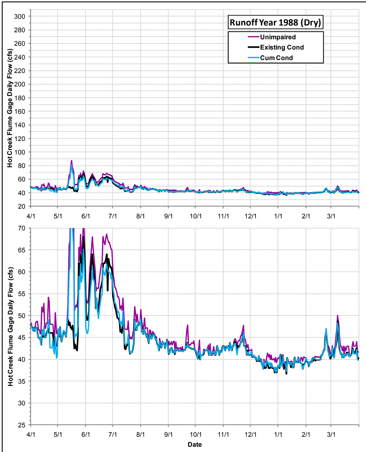
Daily Flows (cfs) at the USGS Hot Creek Flume Gage under the Cumulative Condition, the Existing Condition and the Index of Unimpaired Conditions during Runoff Year 1988
