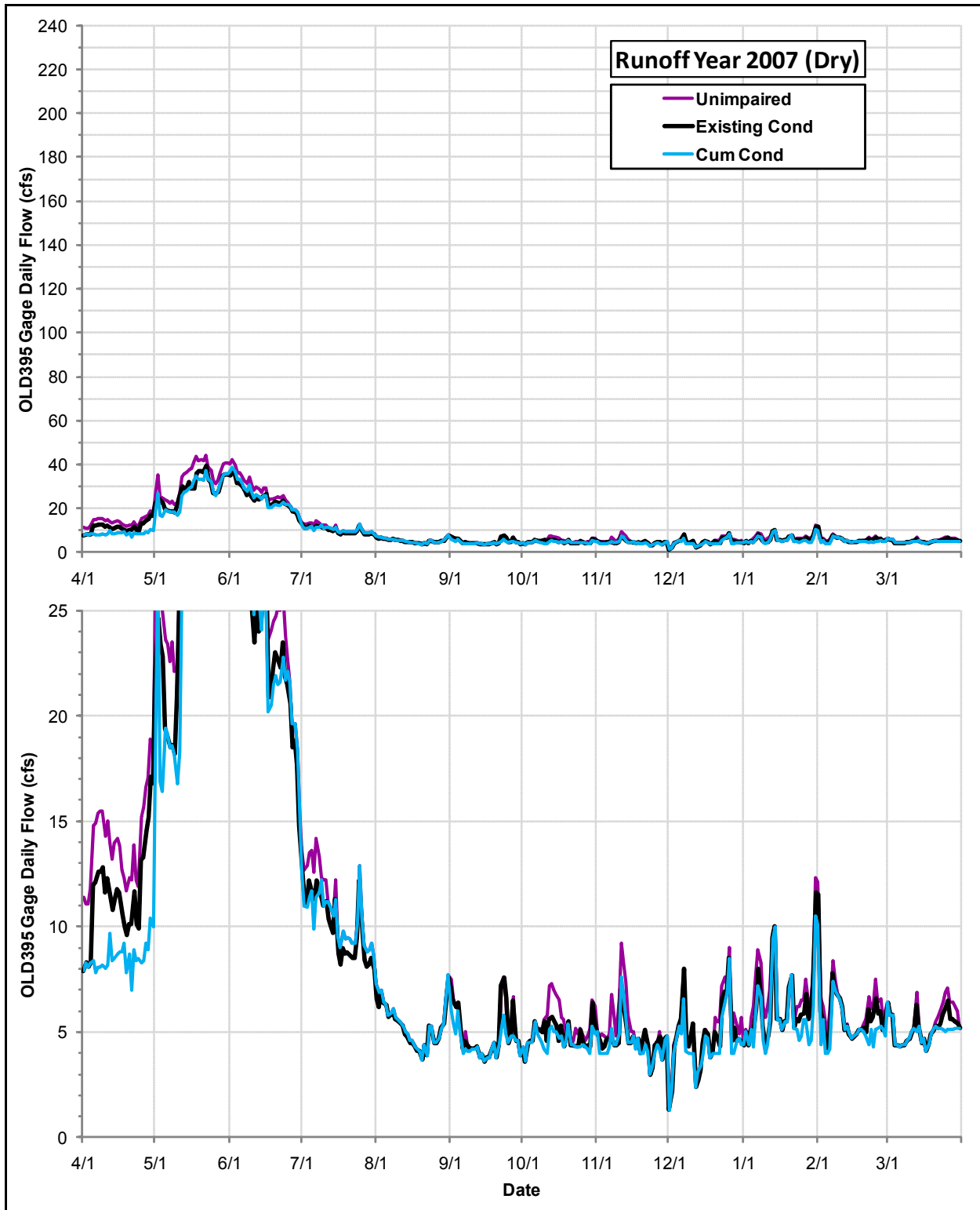
Daily Flows (cfs) at the OLD395 Gage under the Cumulative Condition, the Existing Condition and the Index of Unimpaired Conditions during Runoff Year 2007
