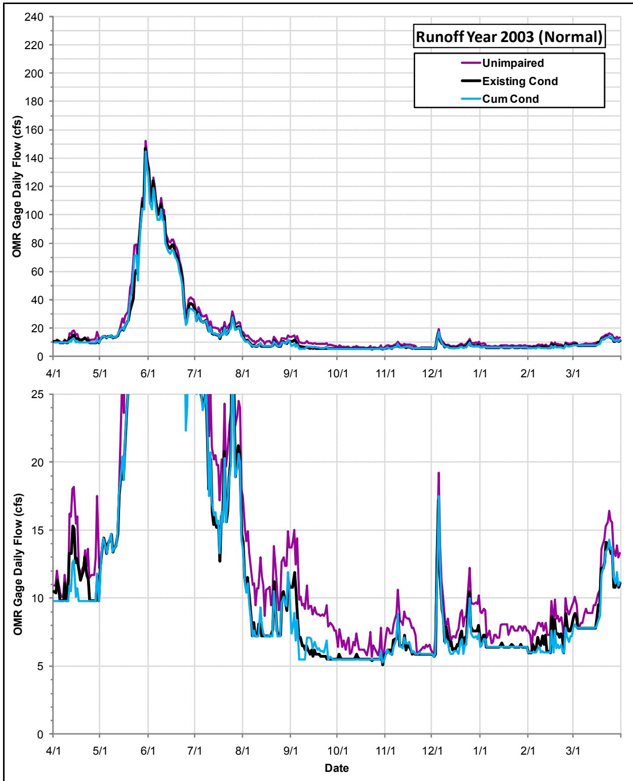
Daily Flows (cfs) at the OMR Gage under the Cumulative Condition, the Existing Condition and the Index of Unimpaired Conditions during Runoff Year 2003
