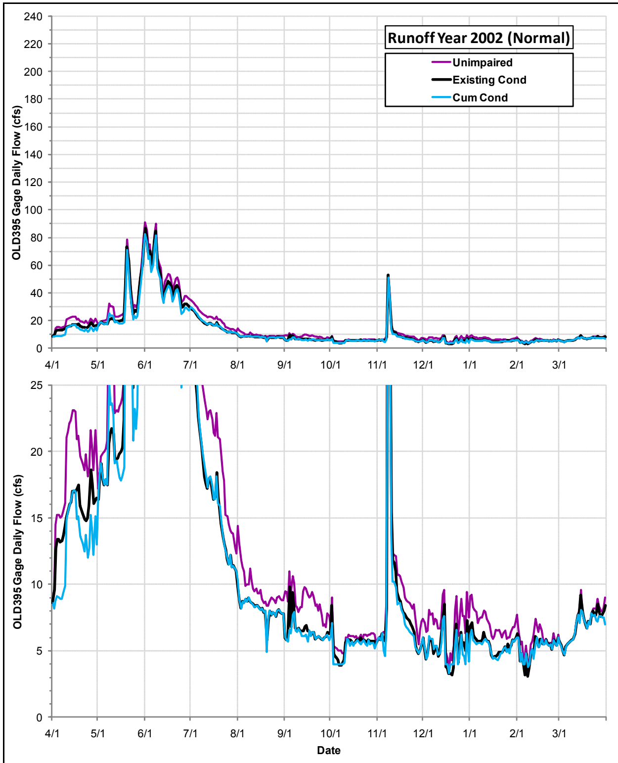
Daily Flows (cfs) at the OLD395 Gage under the Cumulative Condition, the Existing Condition and the Index of Unimpaired Conditions during Runoff Year 2002
