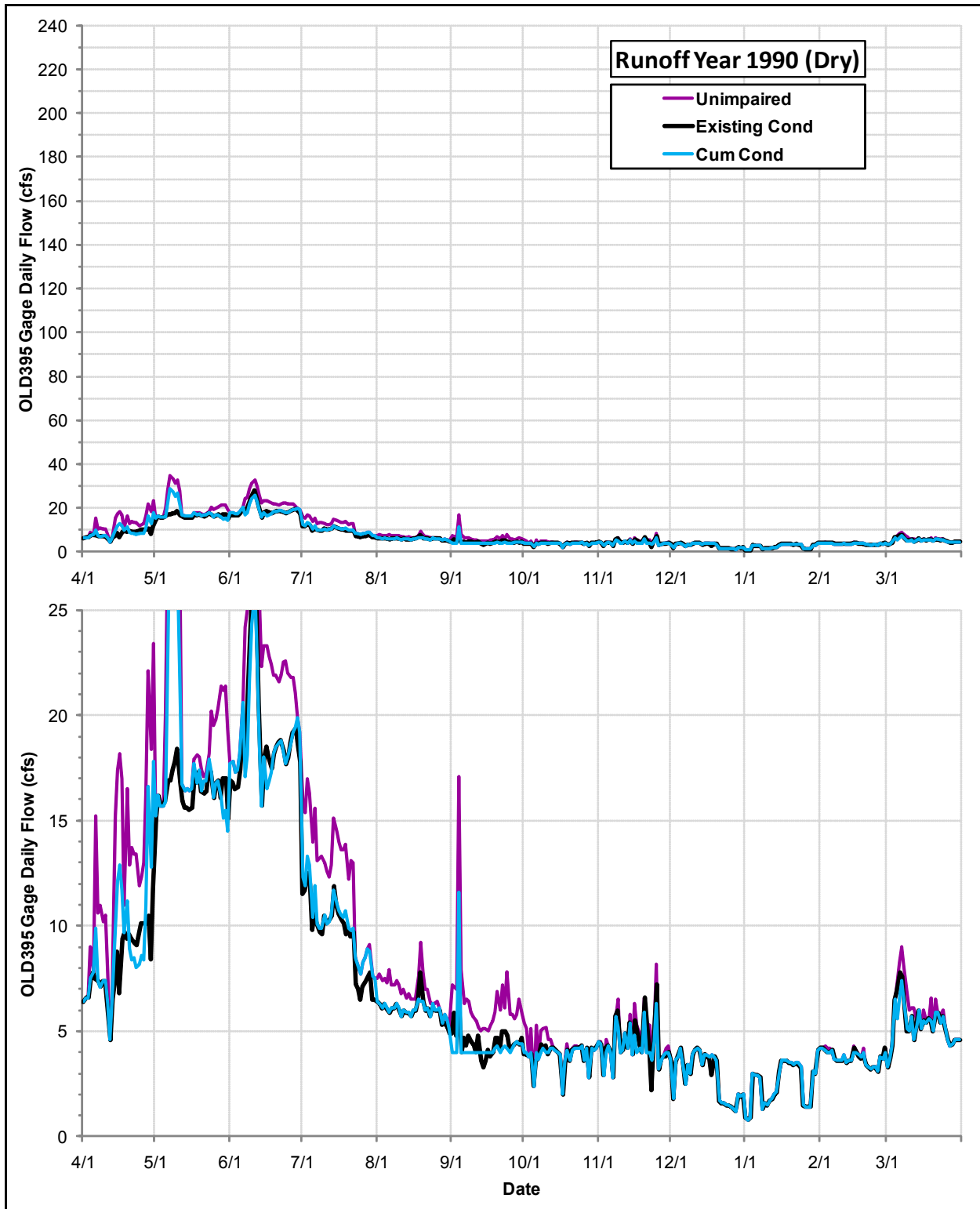
Daily Flows (cfs) at the OLD395 Gage under the Cumulative Condition, the Existing Condition and the Index of Unimpaired Conditions during Runoff Year 1990
