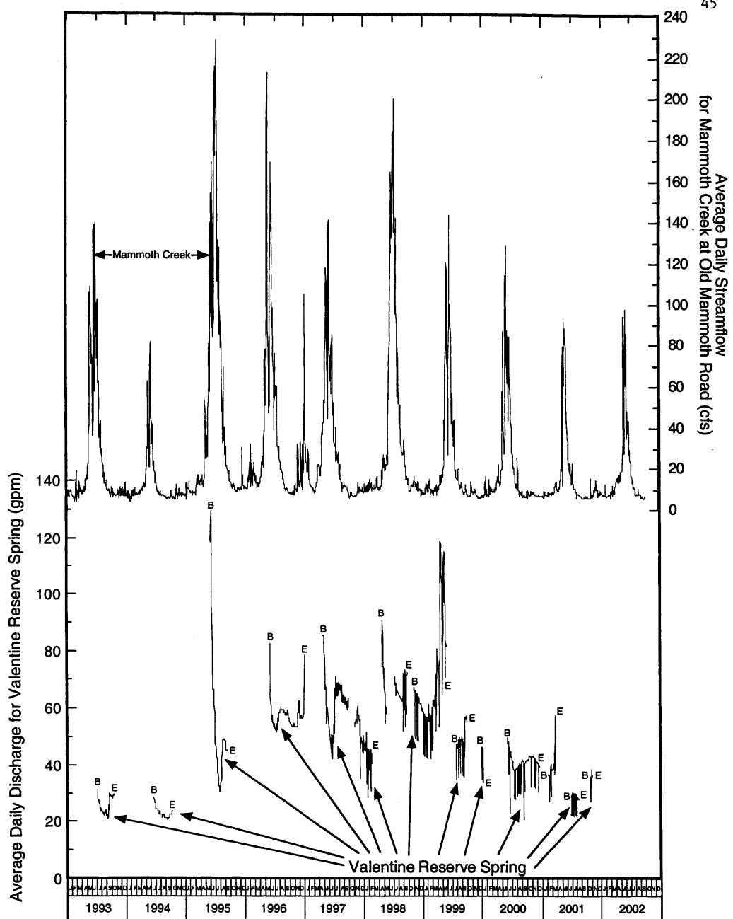
FIGURE 20 - FLOW FOR VALENTINE SPRING (1993-2001) AND MAMMOTH CREEK STREAMFLOW (1993-2002)
