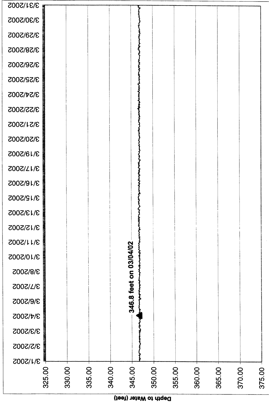
WATER-LEVEL HYDROGRAPH FOR WELL NO. 19 IN MARCH 2002
