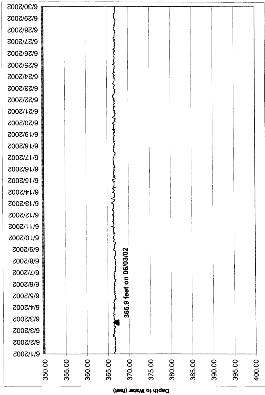
WATER-LEVEL HYDROGRAPH FOR WELL NO. 24 IN JUNE 2002
