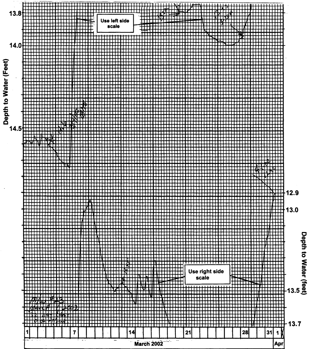
WATER-LEVEL HYDROGRAPH FOR MW-23
