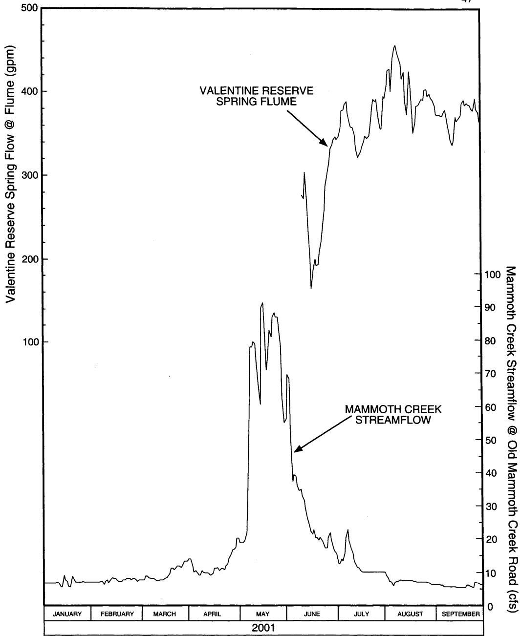
FIGURE 22 - FLOW AT FLUME FOR NEWLY MONITORED VALENTINE RESERVE SPRING AND MAMMOTH CREEK STREAMFLOW (2001)
