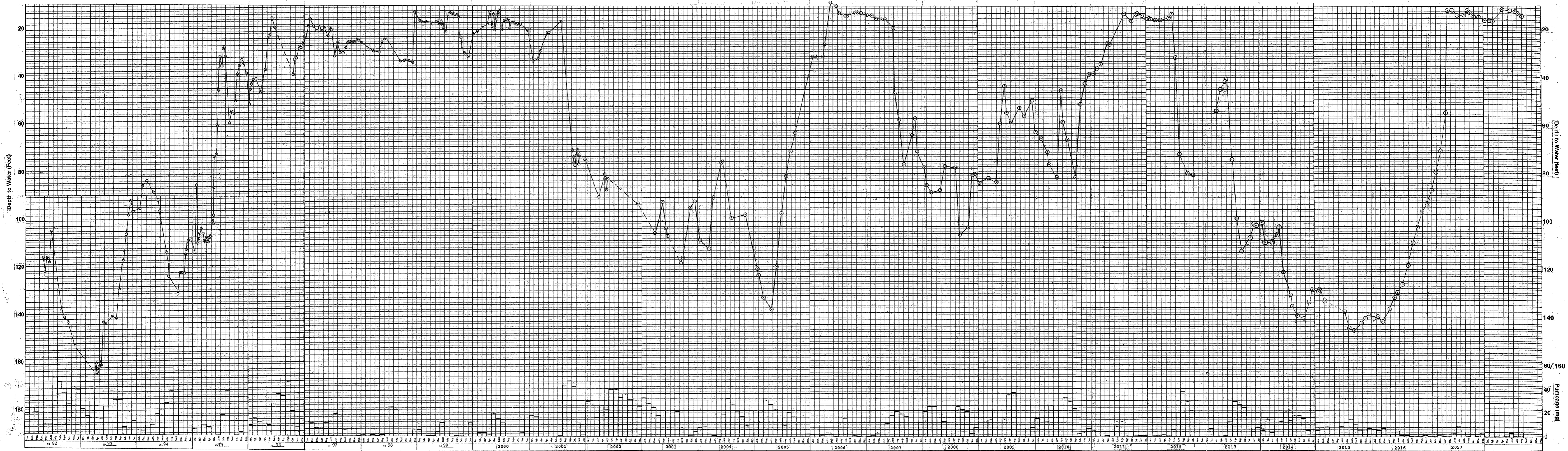
WATER-LEVEL AND PUMPAGE HYDROGRAPH FOR WELL NO. 10
