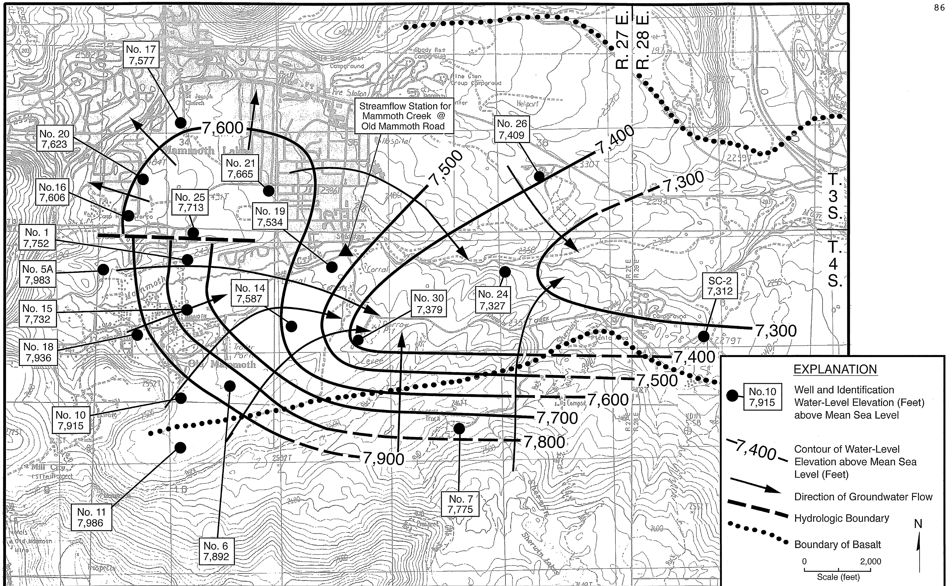
FIGURE 21 - WATER-LEVEL ELEVATIONS IN LATE SEPTEMBER 2018
