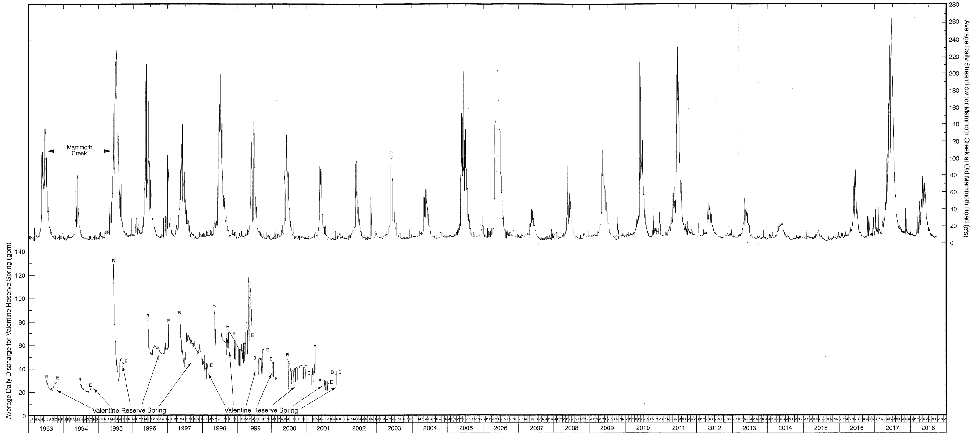
FIGURE 23 - FLOW FOR VALENTINE SPRING (1993-2001) AND MAMMOTH CREEK STREAMFLOW (1993-2018)
