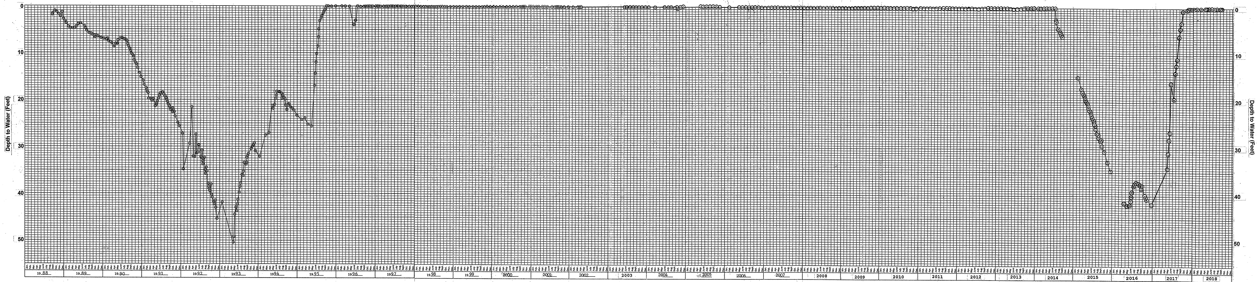
WATER-LEVEL HYDROGRAPH FOR WELL NO. 11
