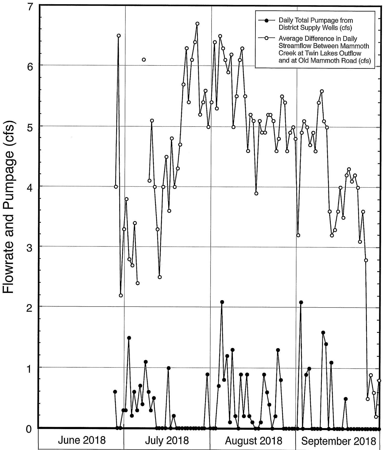
FIGURE 22 - RELATIONSHIP BETWEEN DIFFERENCE IN MAMMOTH CREEK STREAMFLOW AT TWIN LAKES OUTFLOW AND OLD MAMMOTH ROAD AND DISTRICT SUPPLY WELL PUMPAGE (JUNE - SEPTEMBER 2018)
