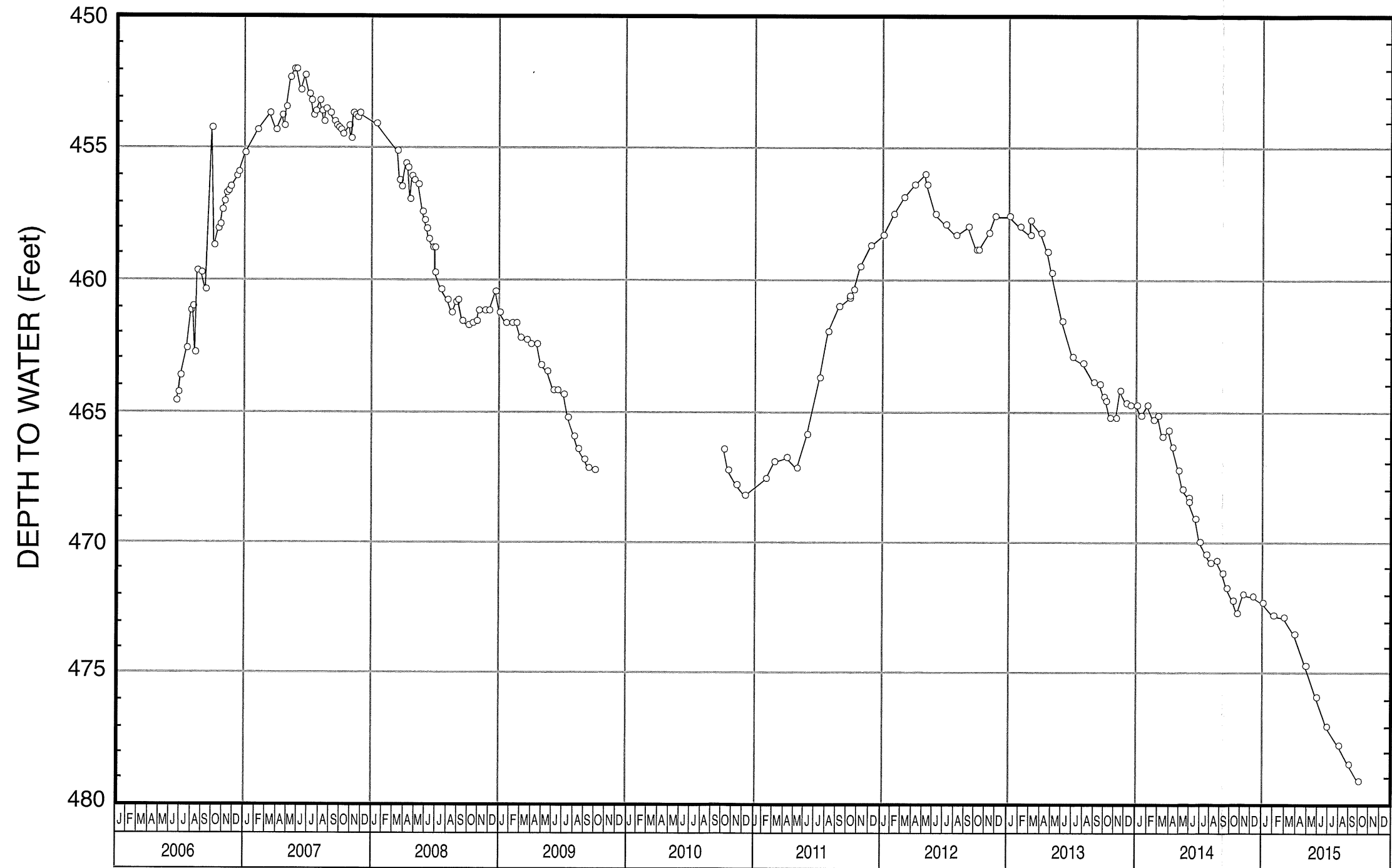
WATER-LEVEL HYDROGRAPH FOR WELL NO. 30
