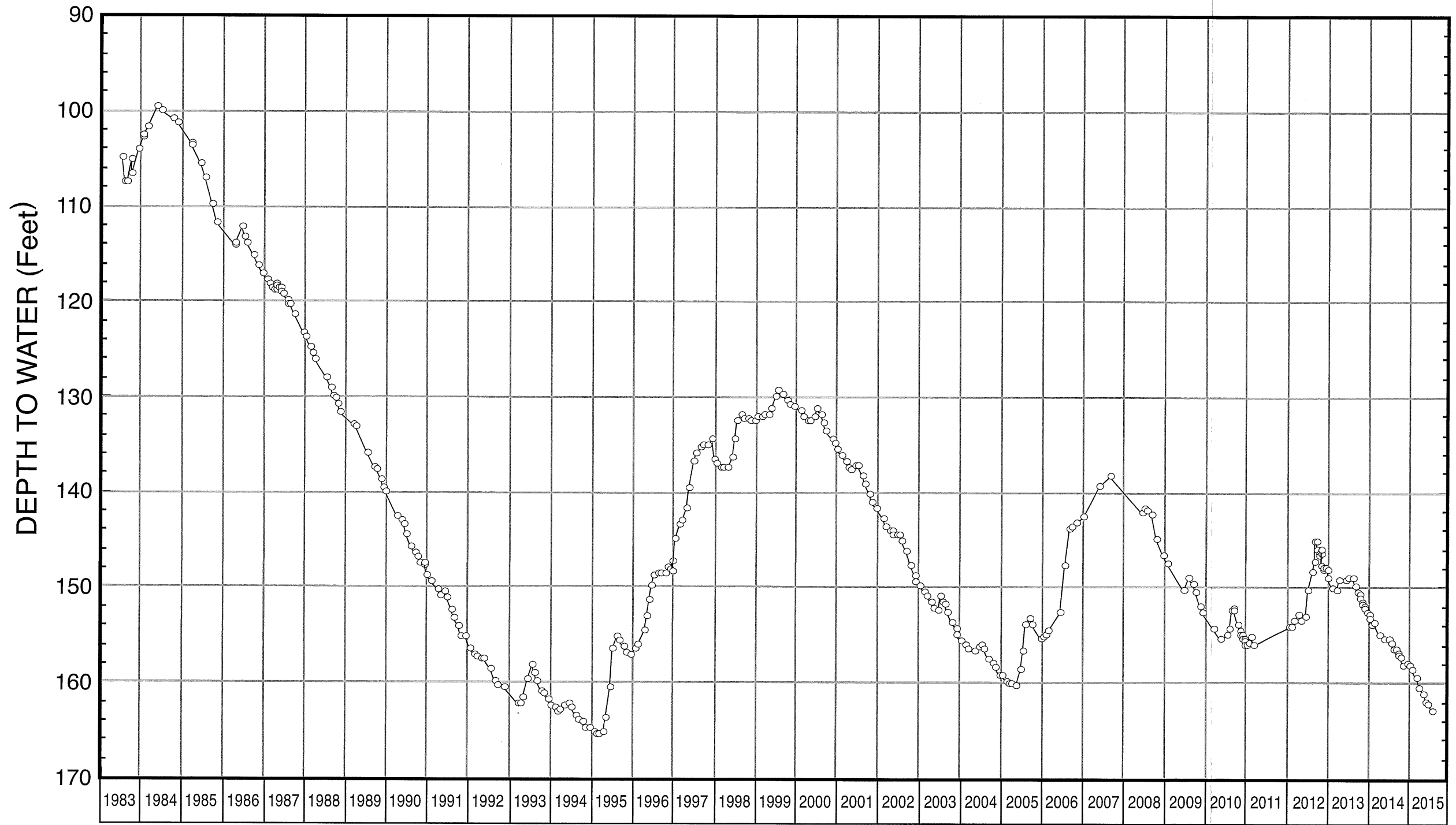
FIGURE 14 - WATER-LEVEL HYDROGRAPH FOR SC-2
