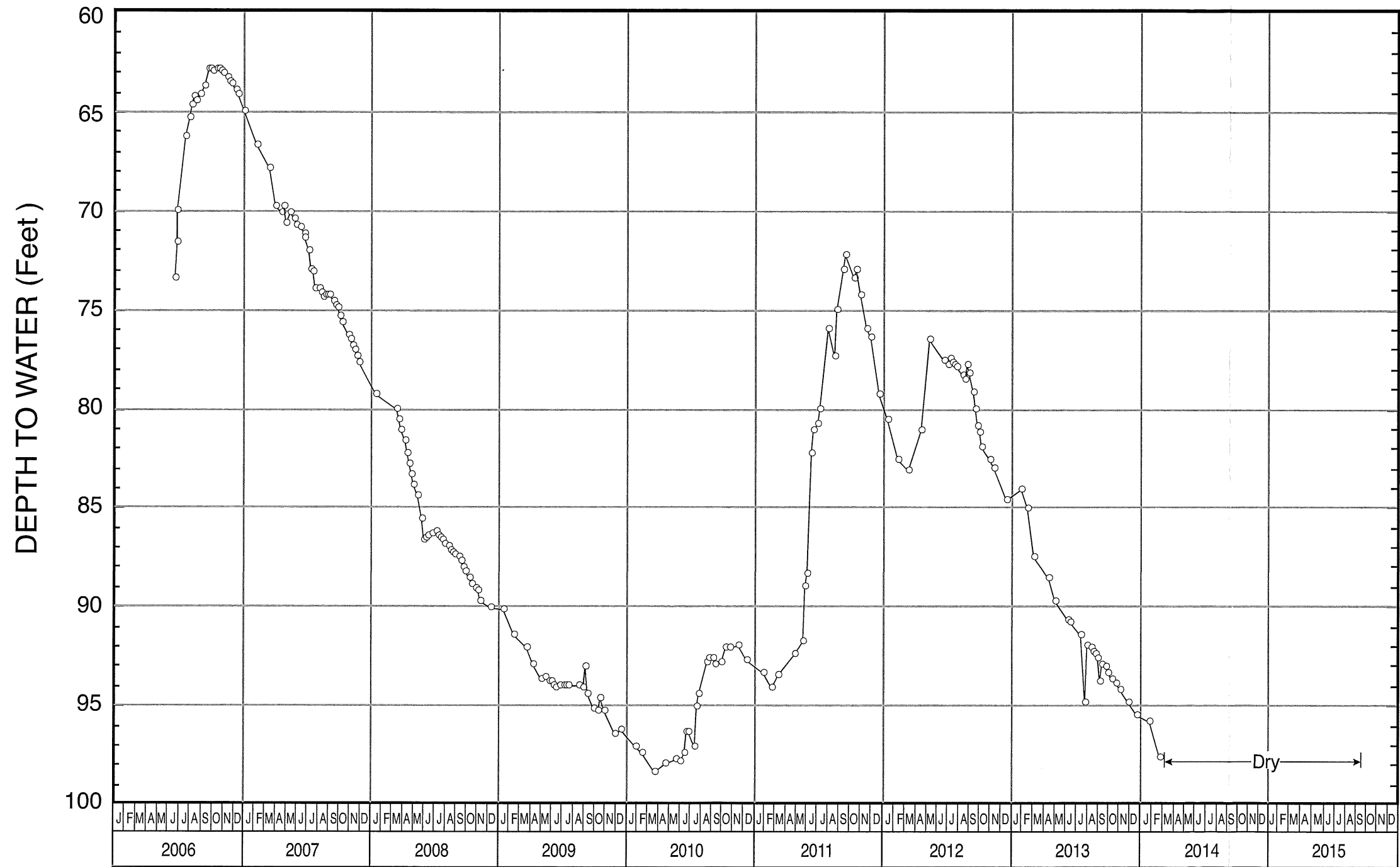
WATER-LEVEL HYDROGRAPH FOR WELL NO. 29
