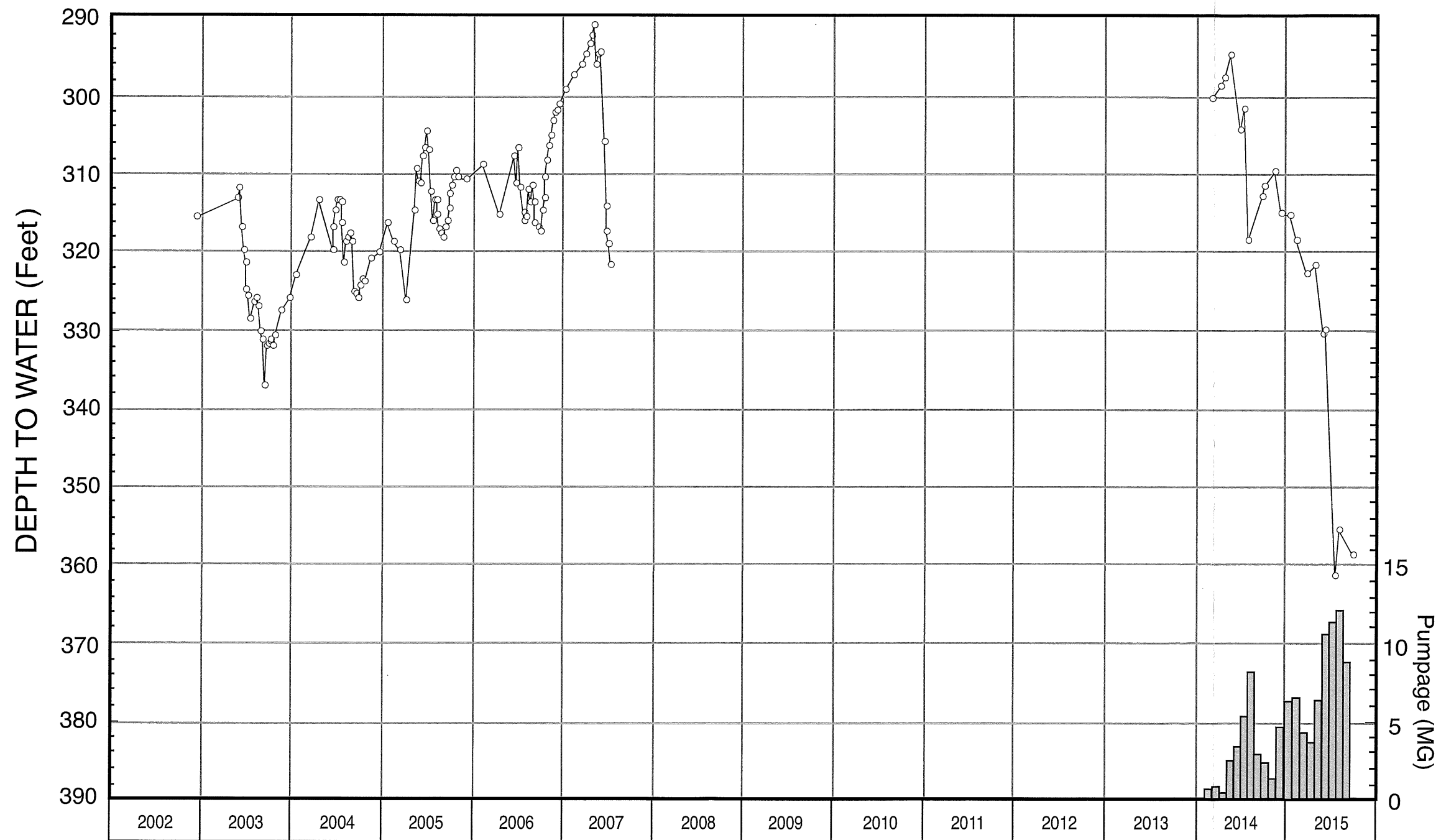
FIGURE 8 - WATER-LEVEL HYDROGRAPH FOR WELL NO. 25
