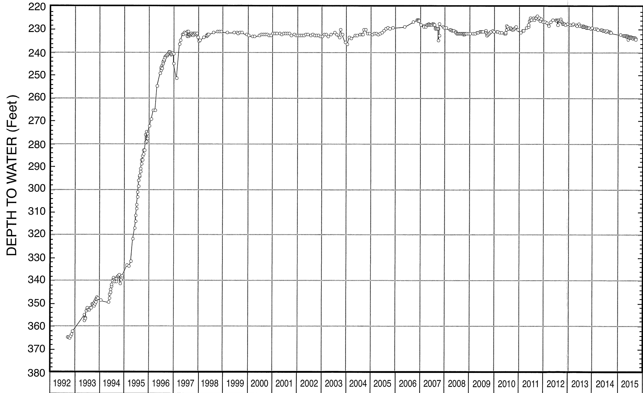
FIGURE 11 - WATER-LEVEL HYDROGRAPH FOR WELL NO. 21
