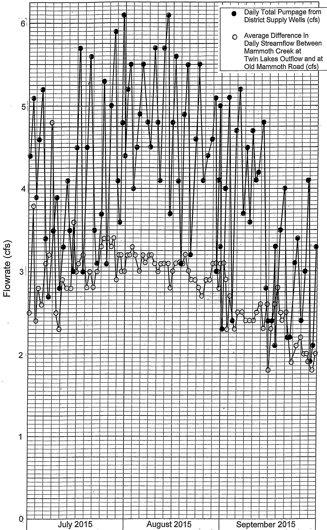
FIGURE 23-RELATIONSHIP BETWEEN DIFFERENCE IN MAMMOTH CREEK STREAMFLOW AT TWIN LAKES OUTFLOW AND OLD MAMMOTH ROAD AND DISTRICT SUPPLY WELL PUMPAGE (JULY-SEPTEMBER, 2015)
