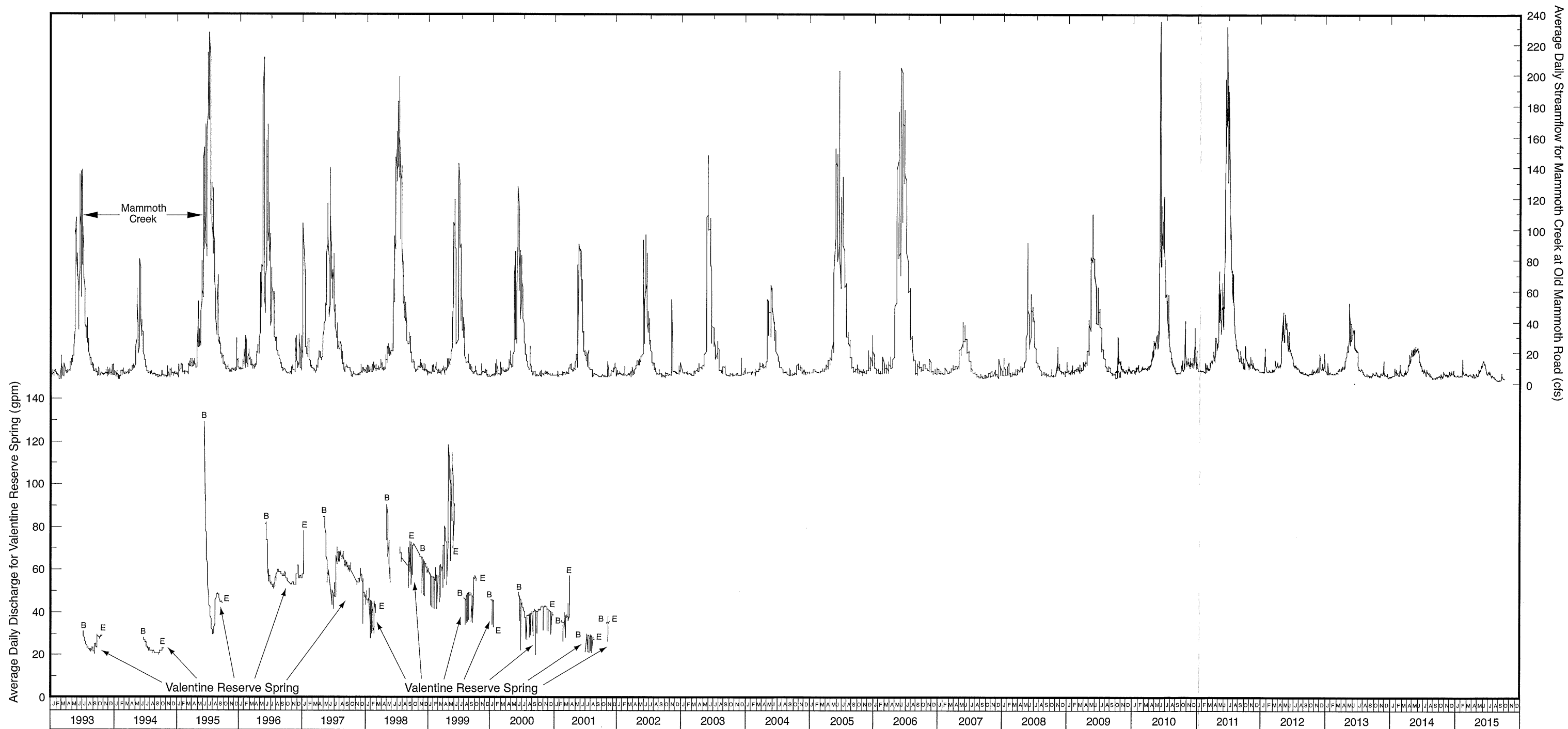
FIGURE 24 - FLOW FOR VALENTINE SPRING (1993-2001) AND MAMMOTH CREEK STREAMFLOW (1993-2015)
