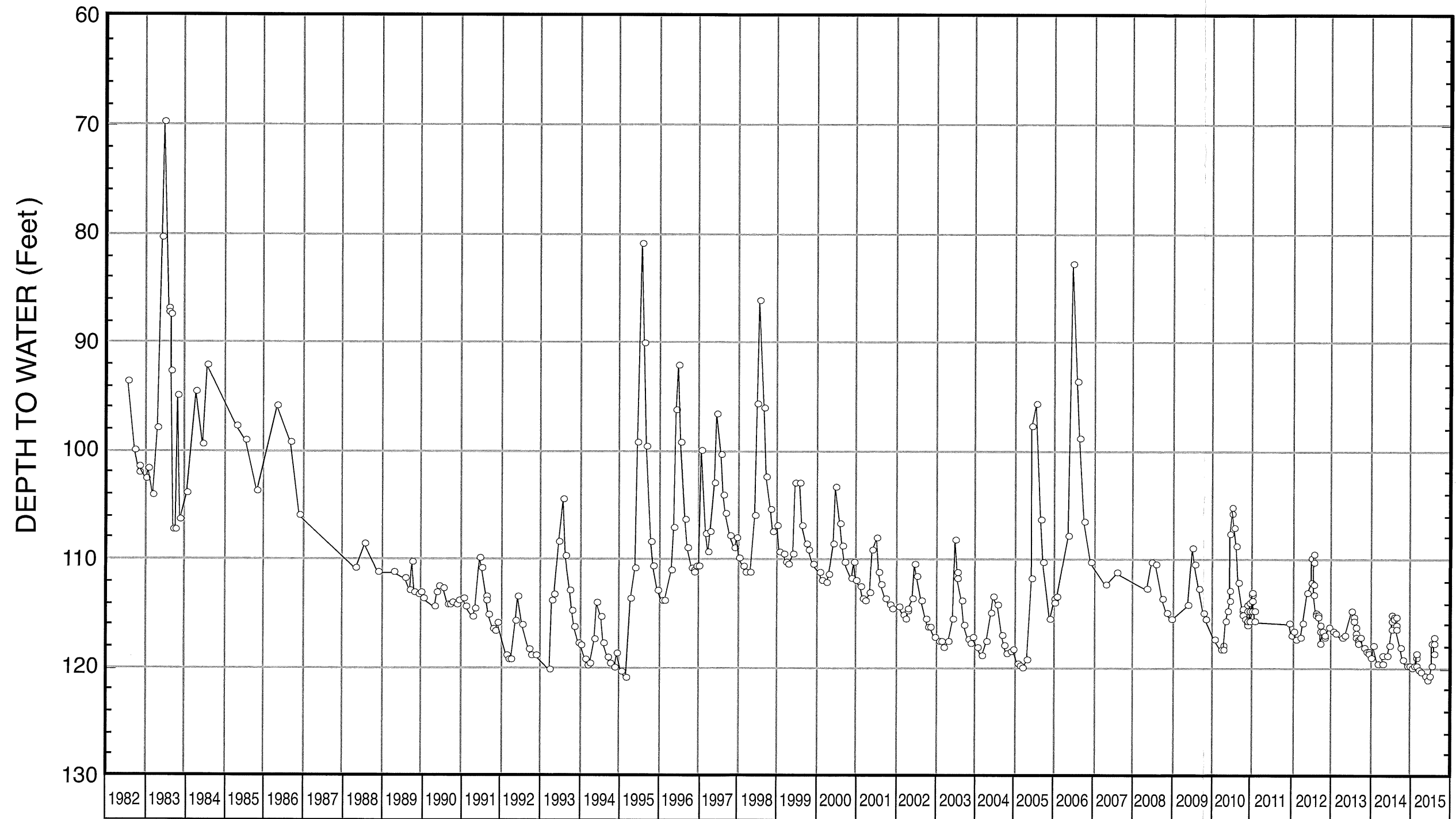
FIGURE 13 - WATER-LEVEL HYDROGRAPH FOR SC-1
