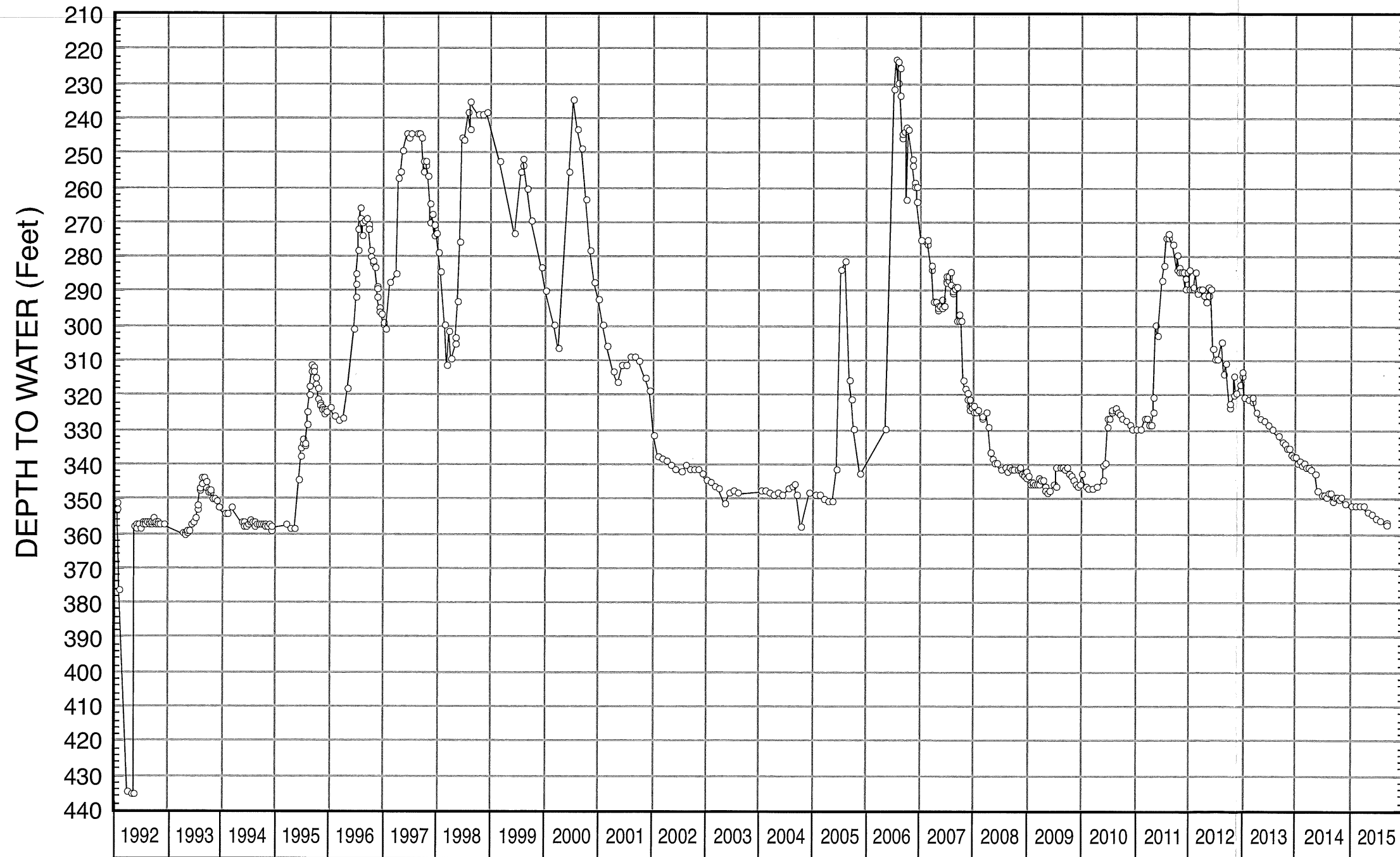
FIGURE 9 - WATER-LEVEL HYDROGRAPH FOR WELL NO. 14M
