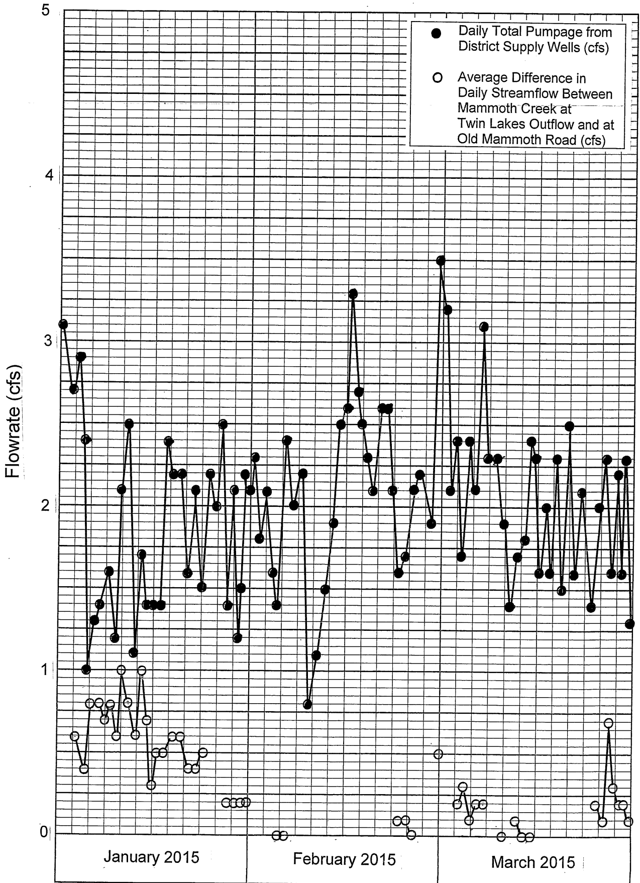
FIGURE 21-RELATIONSHIP BETWEEN DIFFERENCE IN MAMMOTH CREEK STREAMFLOW AT TWIN LAKES OUTFLOW AND OLD MAMMOTH ROAD AND DISTRICT SUPPLY WELL PUMPAGE (JANUARY-MARCH, 2015)
