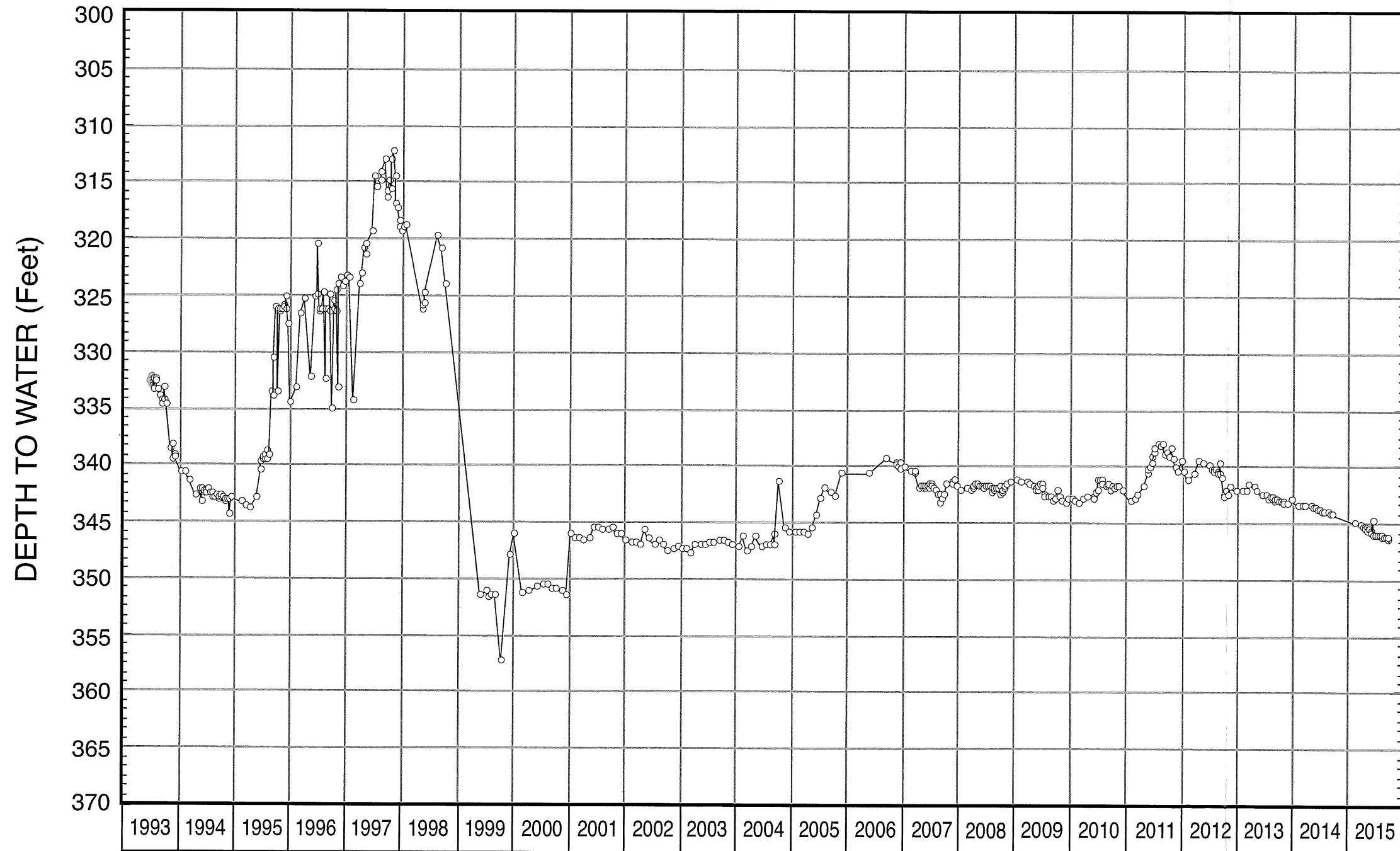
FIGURE 10 - WATER-LEVEL HYDROGRAPH FOR WELL NO. 19
