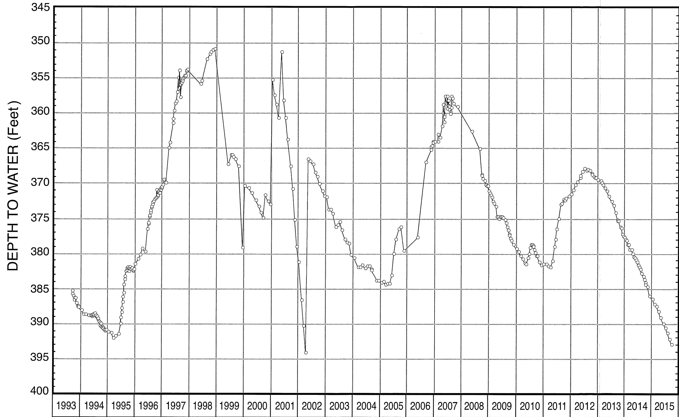
FIGURE 12 - WATER-LEVEL HYDROGRAPH FOR WELL NO. 24
