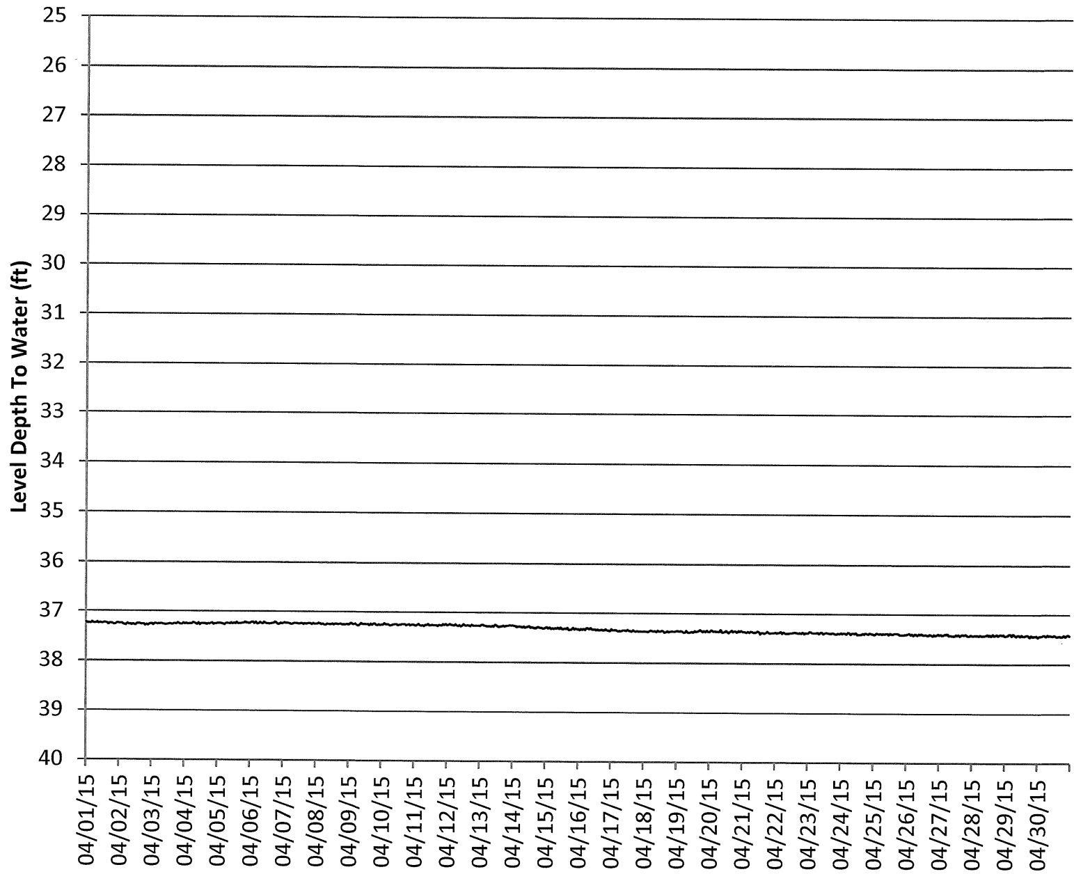
WATER LEVEL HYDROGRAPH FOR MW-11M
