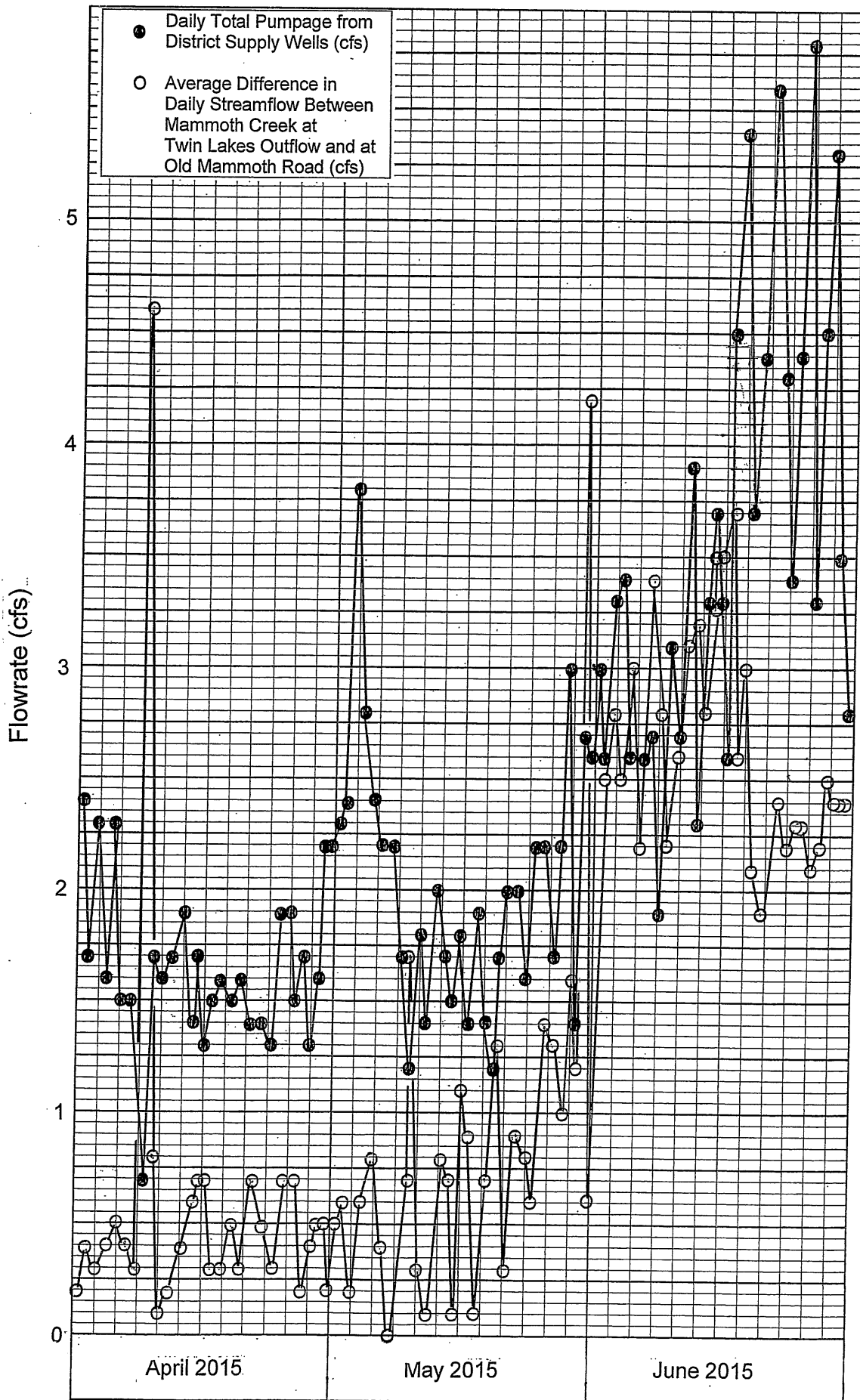
FIGURE 22-RELATIONSHIP BETWEEN DIFFERENCE IN MAMMOTH CREEK STREAMFLOW AT TWIN LAKES OUTFLOW AND OLD MAMMOTH ROAD AND DISTRICT SUPPLY WELL PUMPAGE (APRIL-JUNE, 2015)
