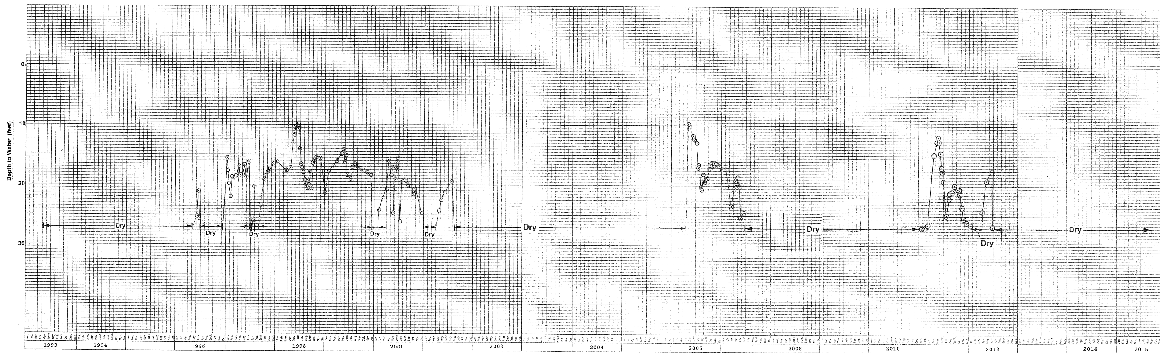
WATER-LEVEL HYDROGRAPH FOR WELL NO. 10M
