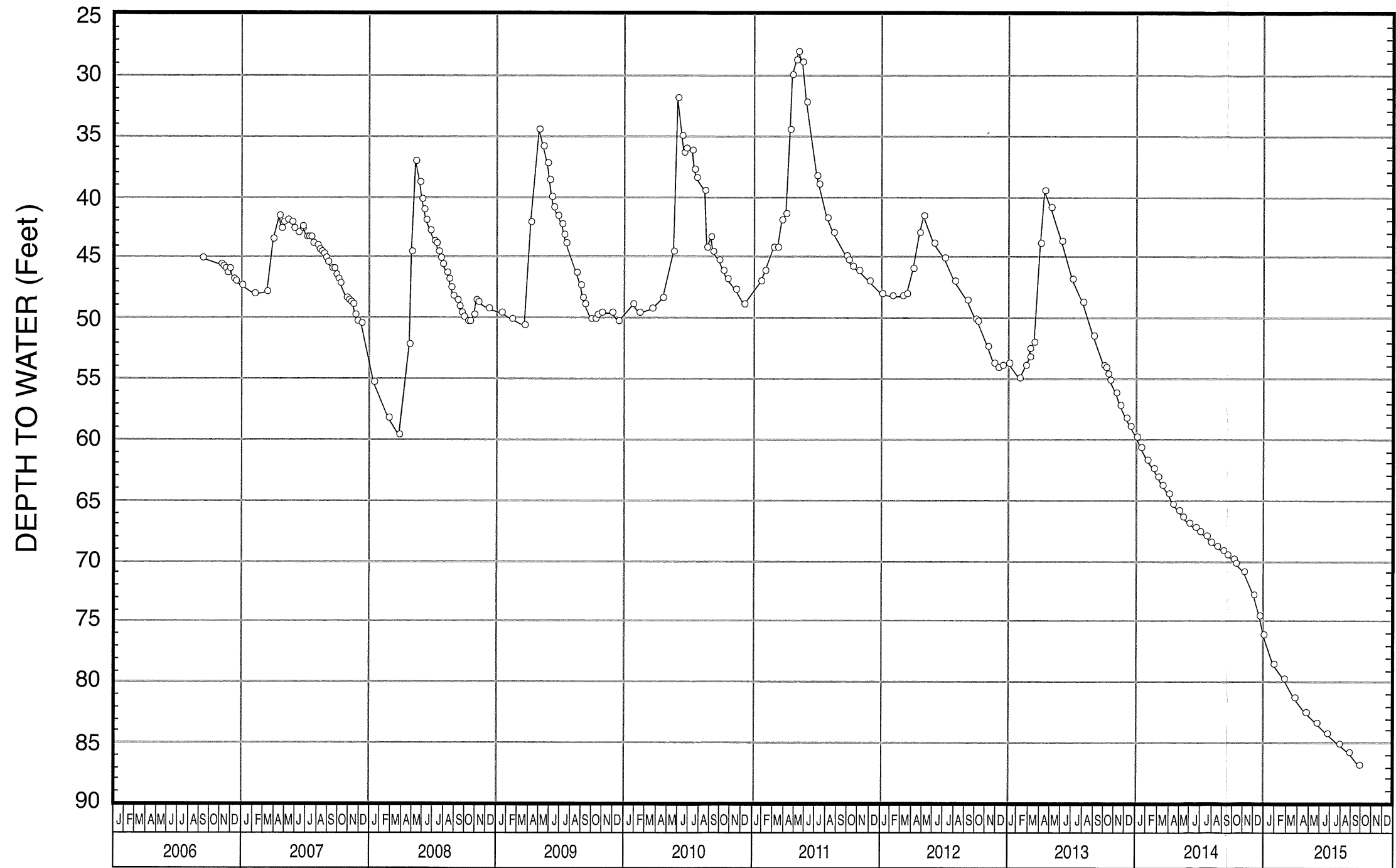
WATER-LEVEL HYDROGRAPH FOR WELL NO. 27
