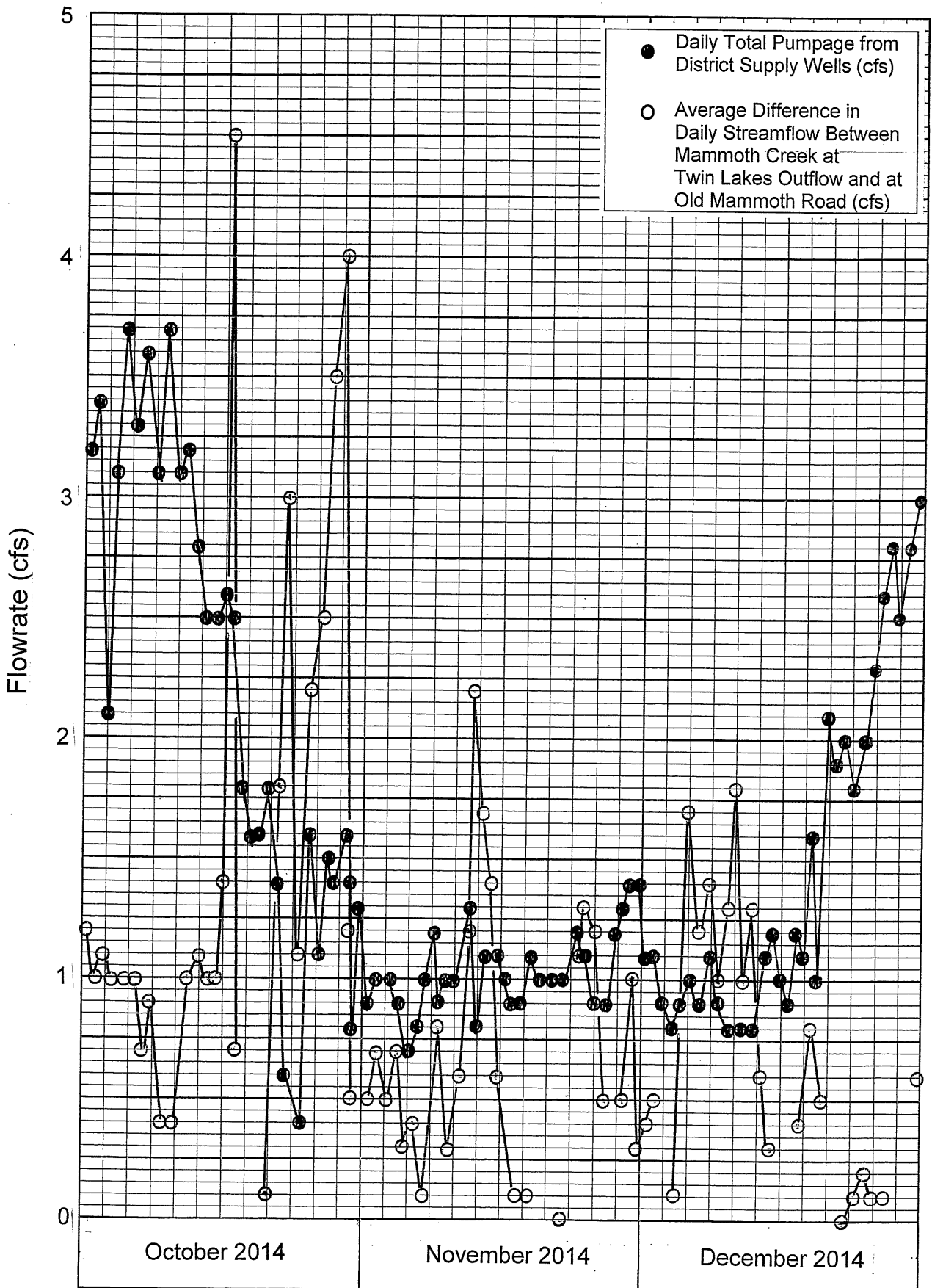
FIGURE 20-RELATIONSHIP BETWEEN DIFFERENCE IN MAMMOTH CREEK STREAMFLOW AT TWIN LAKES OUTFLOW AND OLD MAMMOTH ROAD AND DISTRICT SUPPLY WELL PUMPAGE (OCTOBER-DECEMBER, 2014)
