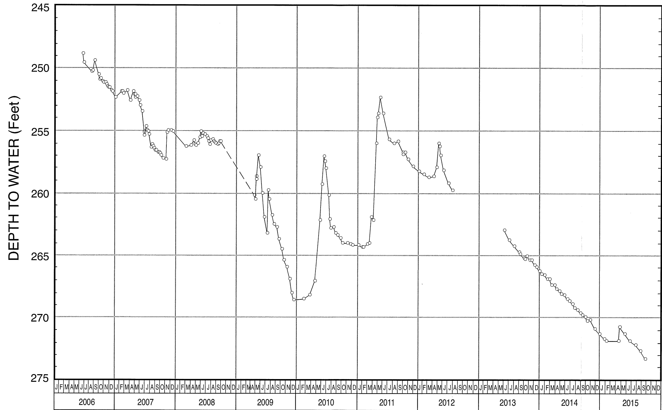
WATER-LEVEL HYDROGRAPH FOR WELL NO. 26
