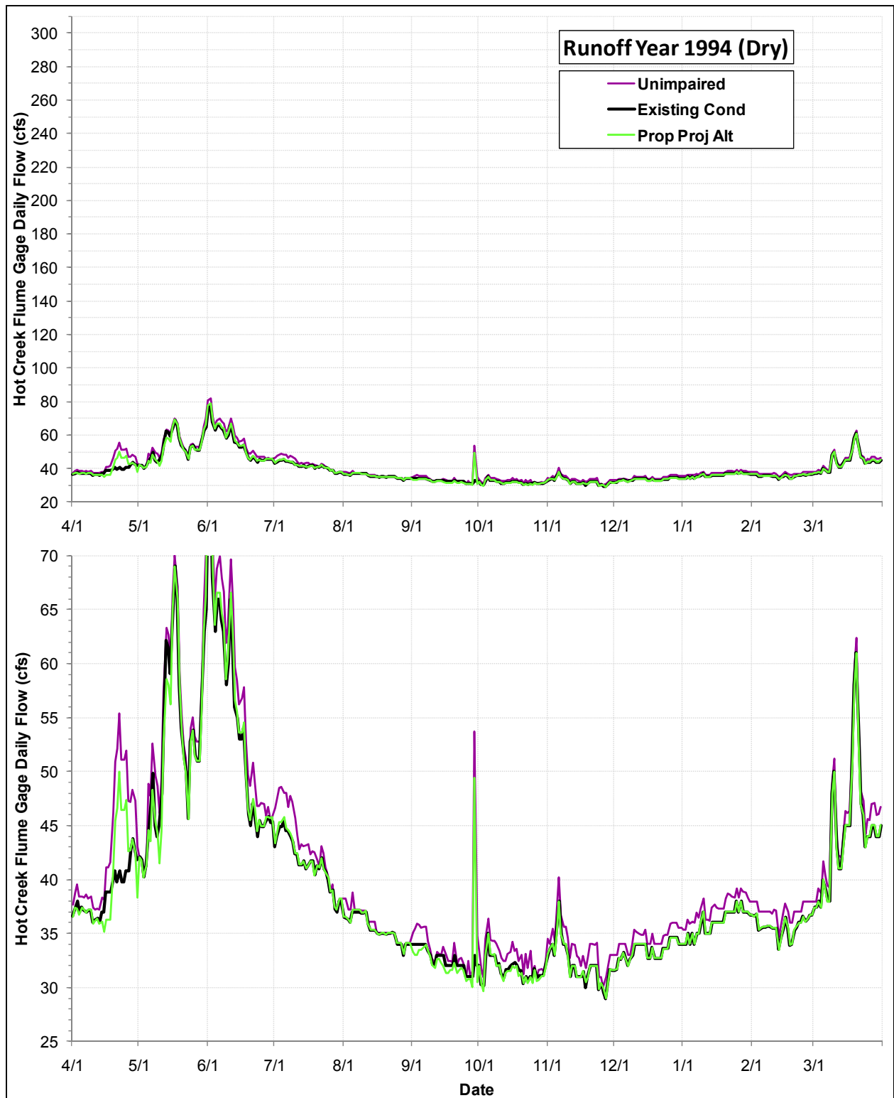
Daily Flows (cfs) at the USGS Hot Creek Flume Gage under the Proposed Project Alternative, the Existing Condition and the Index of Unimpaired Conditions during Runoff Year 1994
