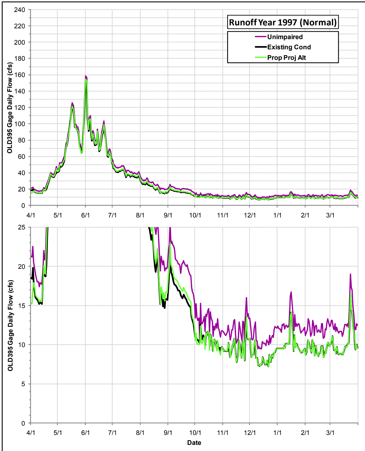
Daily Flows (cfs) at the OLD395 Gage under the Proposed Project Alternative, the Existing Condition and the Index of Unimpaired Conditions during Runoff Year 1997
