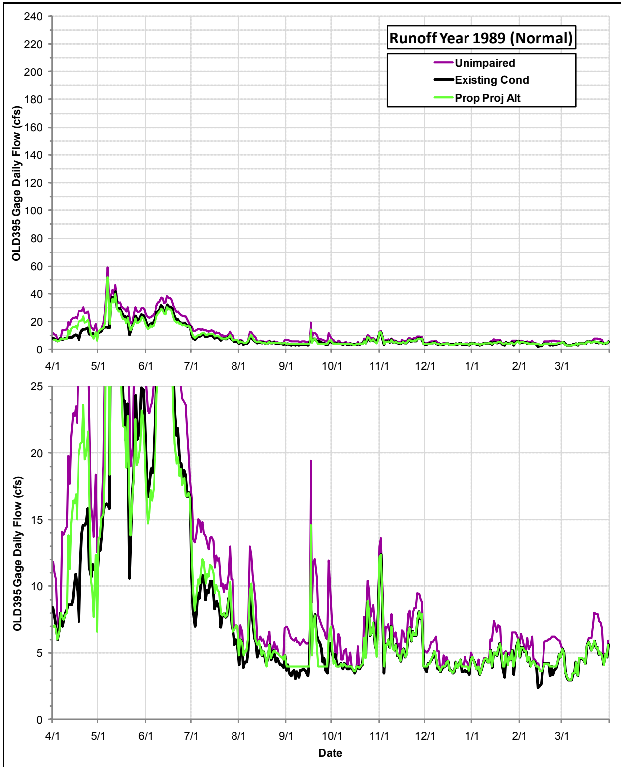
Daily Flows (cfs) at the OLD395 Gage under the Proposed Project Alternative, the Existing Condition and the Index of Unimpaired Conditions during Runoff Year 1989
