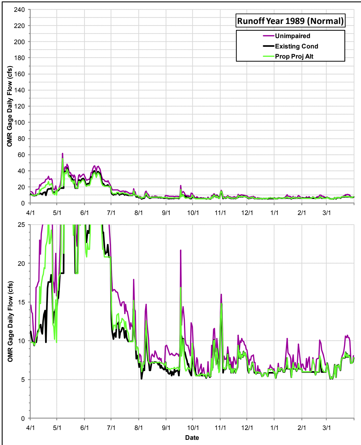
Daily Flows (cfs) at the OMR Gage under the Proposed Project Alternative, the Existing Condition and the Index of Unimpaired Conditions during Runoff Year 1989
