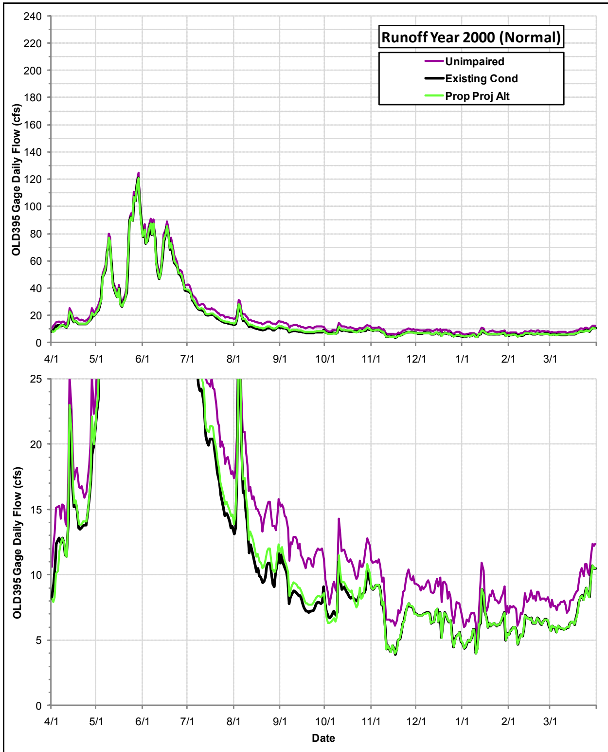
Daily Flows (cfs) at the OLD395 Gage under the Proposed Project Alternative, the Existing Condition and the Index of Unimpaired Conditions during Runoff Year 2000
