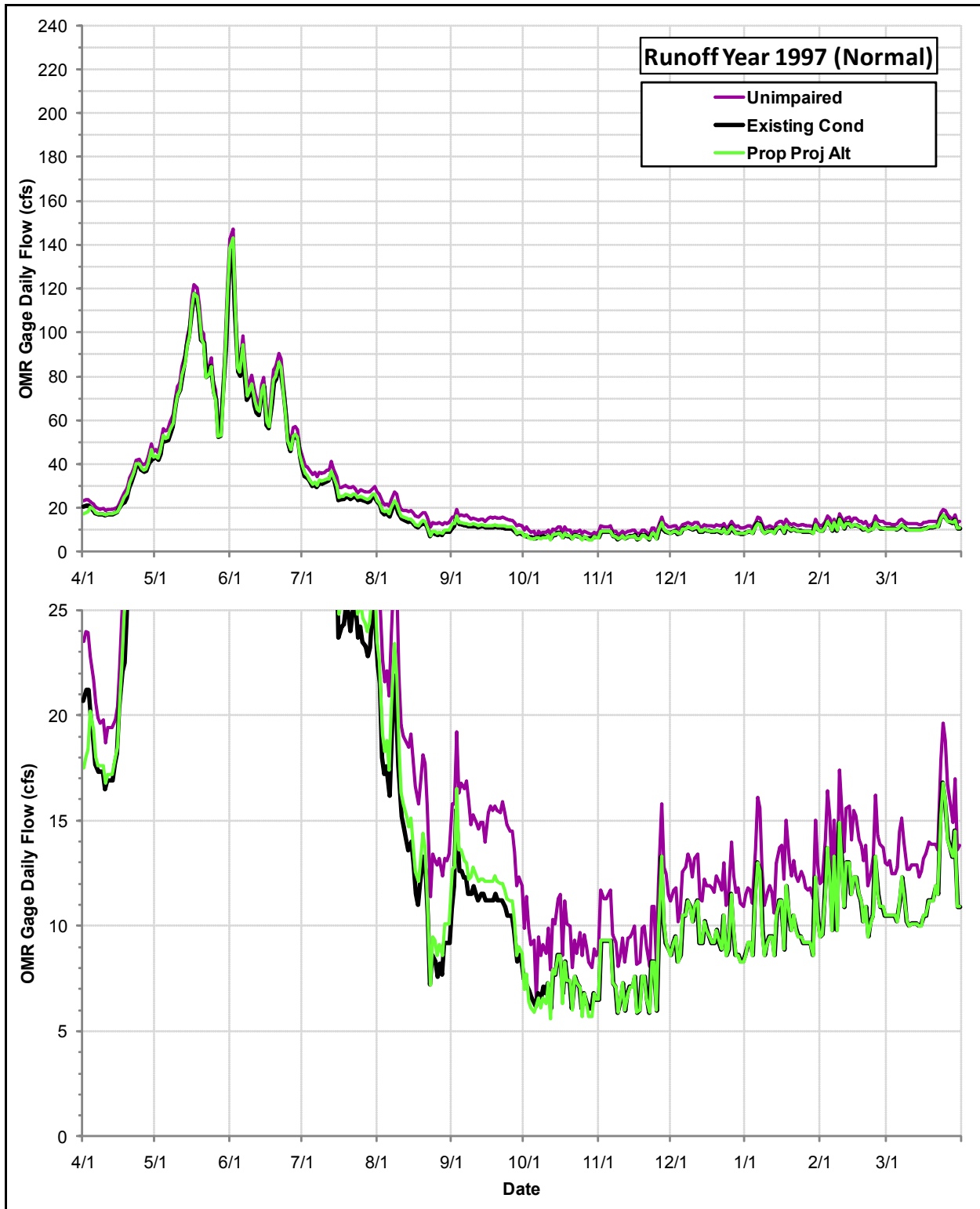
Daily Flows (cfs) at the OMR Gage under the Proposed Project Alternative, the Existing Condition and the Index of Unimpaired Conditions during Runoff Year 1997
