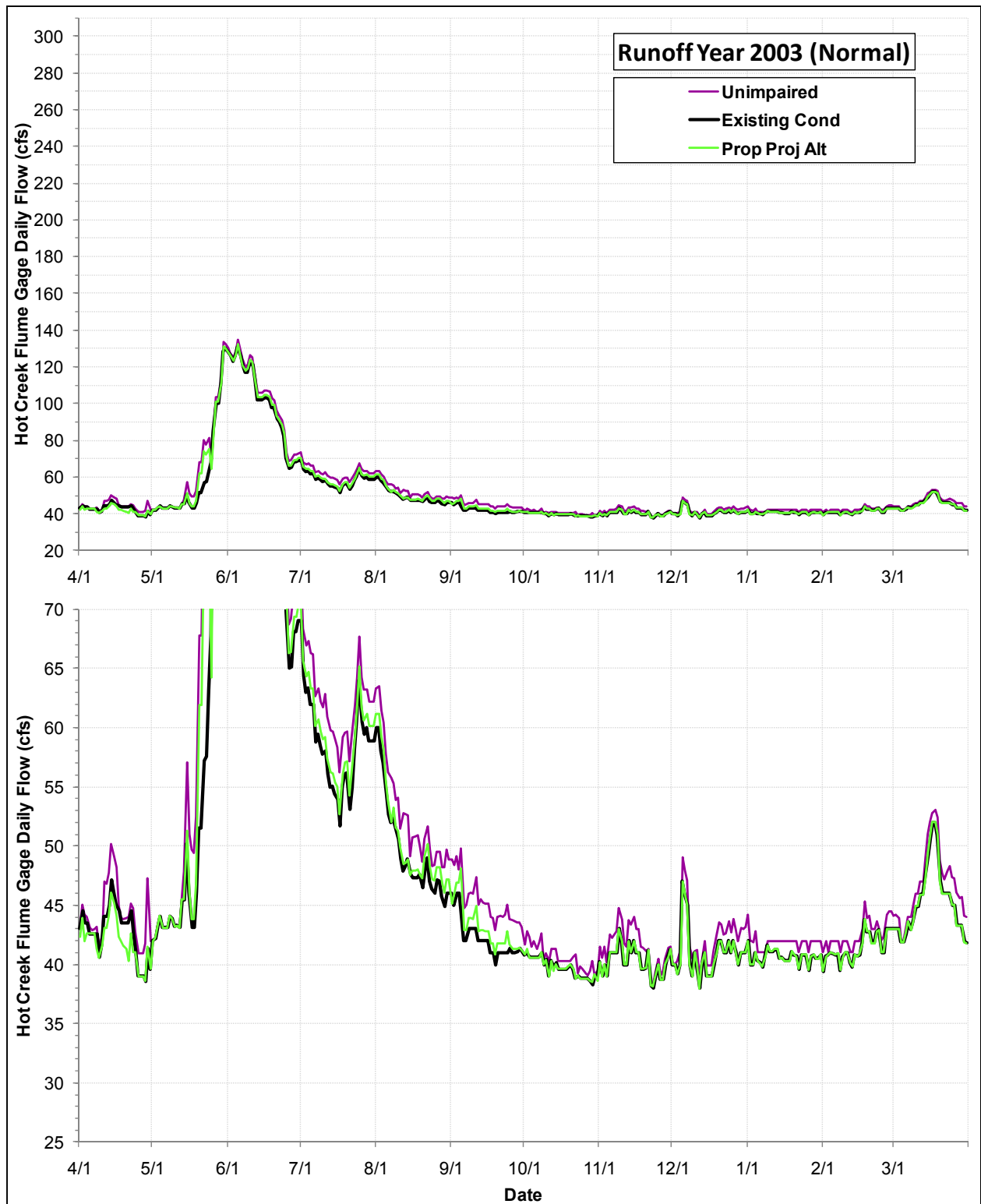
Daily Flows (cfs) at the USGS Hot Creek Flume Gage under the Proposed Project Alternative, the Existing Condition and the Index of Unimpaired Conditions during Runoff Year 2003
