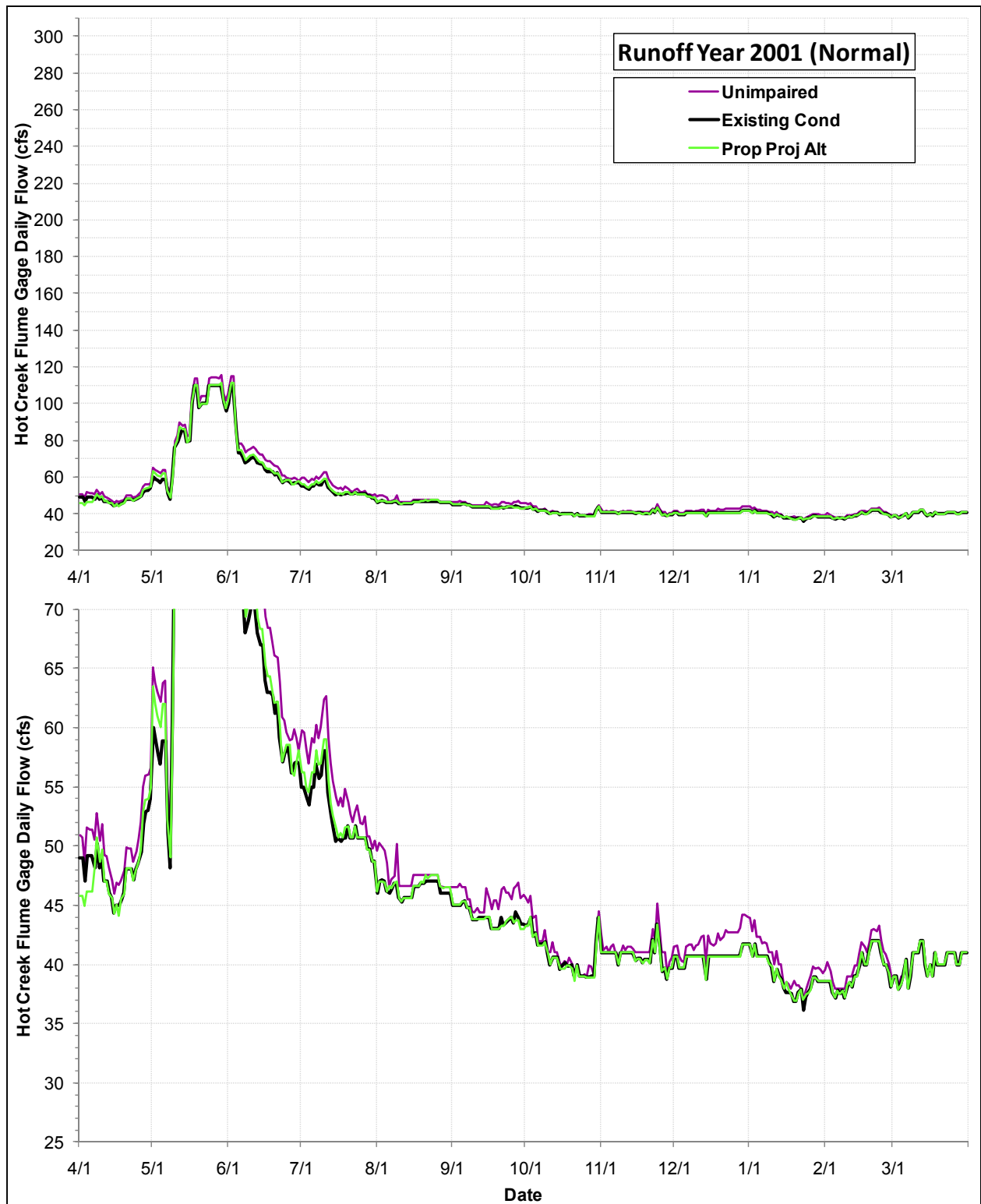
Daily Flows (cfs) at the USGS Hot Creek Flume Gage under the Proposed Project Alternative, the Existing Condition and the Index of Unimpaired Conditions during Runoff Year 2001
