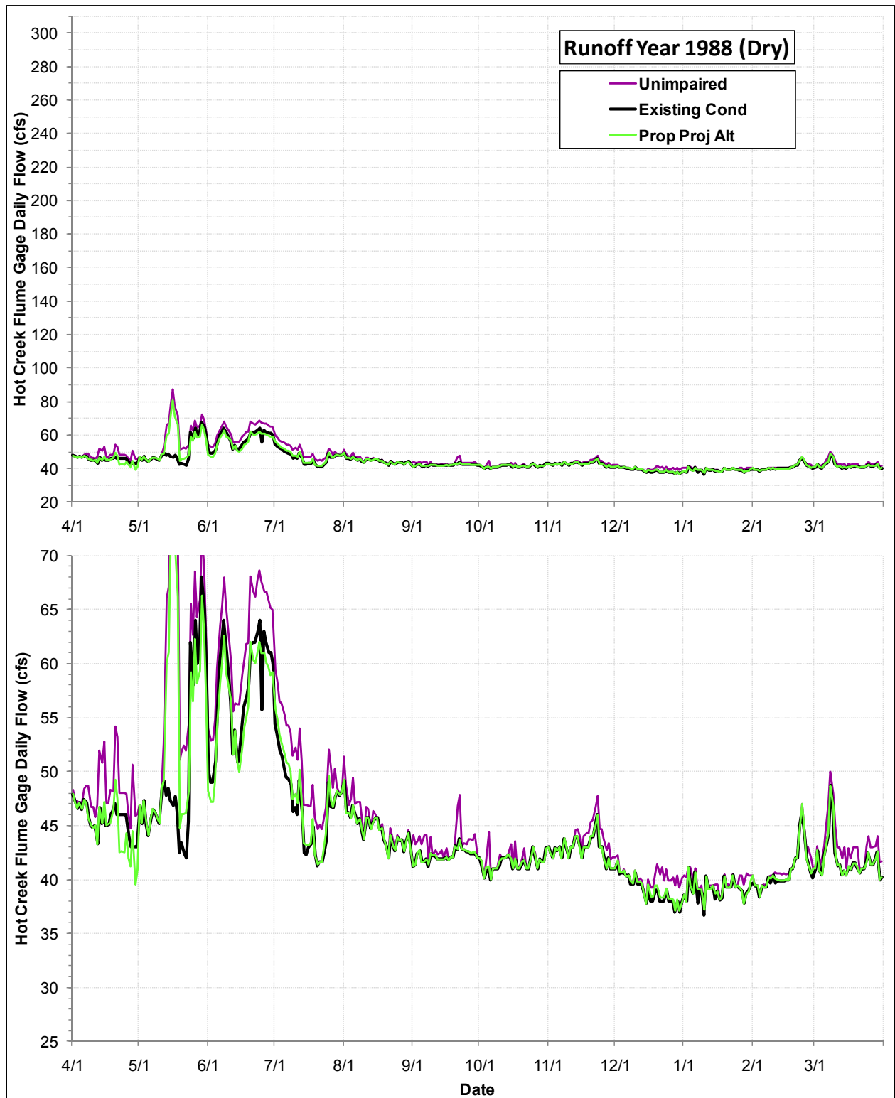
Daily Flows (cfs) at the USGS Hot Creek Flume Gage under the Proposed Project Alternative, the Existing Condition and the Index of Unimpaired Conditions during Runoff Year 1988
