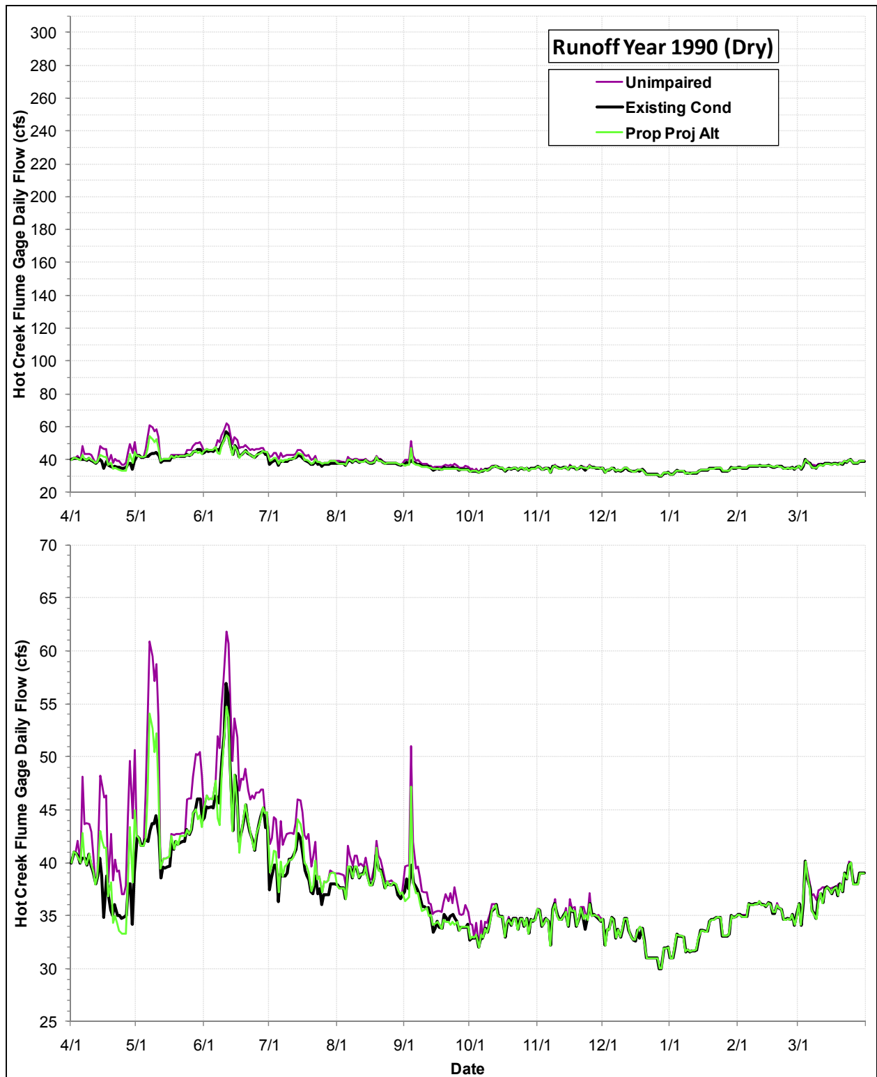
Daily Flows (cfs) at the USGS Hot Creek Flume Gage under the Proposed Project Alternative, the Existing Condition and the Index of Unimpaired Conditions during Runoff Year 1990
