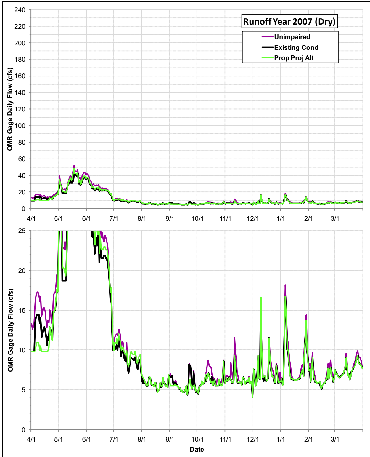
Daily Flows (cfs) at the OMR Gage under the Proposed Project Alternative, the Existing Condition and the Index of Unimpaired Conditions during Runoff Year 2007
