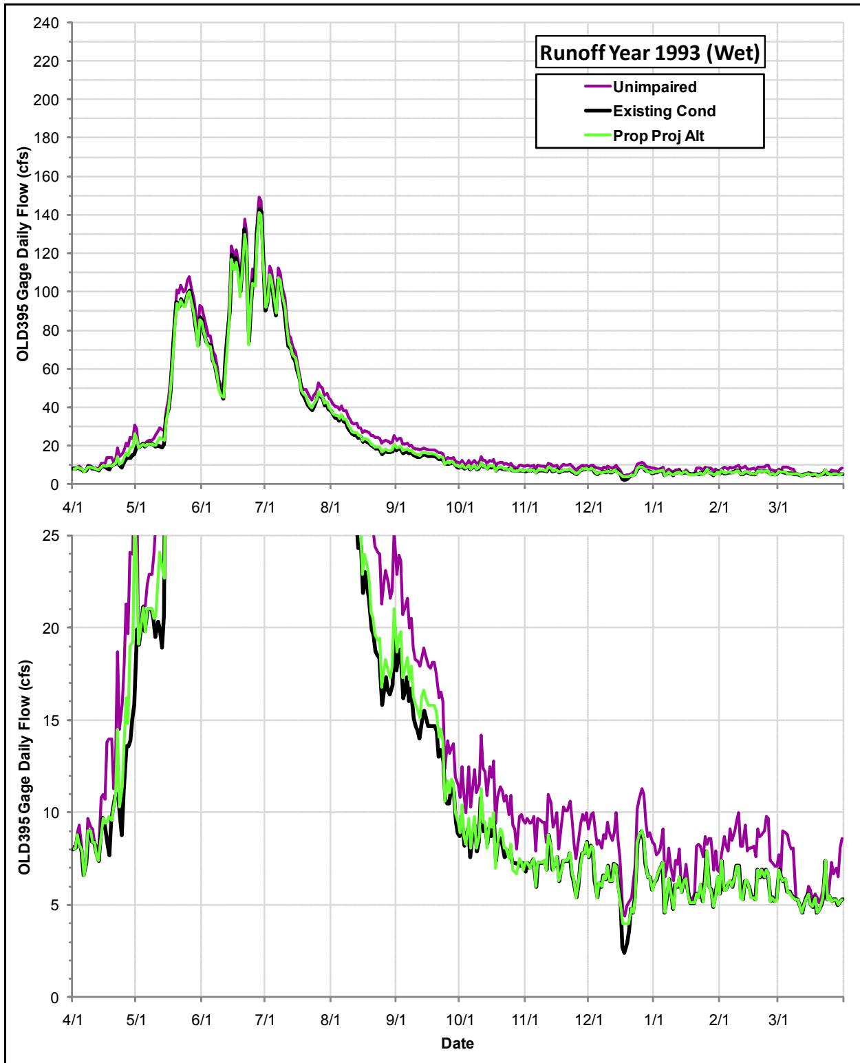
Daily Flows (cfs) at the OLD395 Gage under the Proposed Project Alternative, the Existing Condition and the Index of Unimpaired Conditions during Runoff Year 1993
