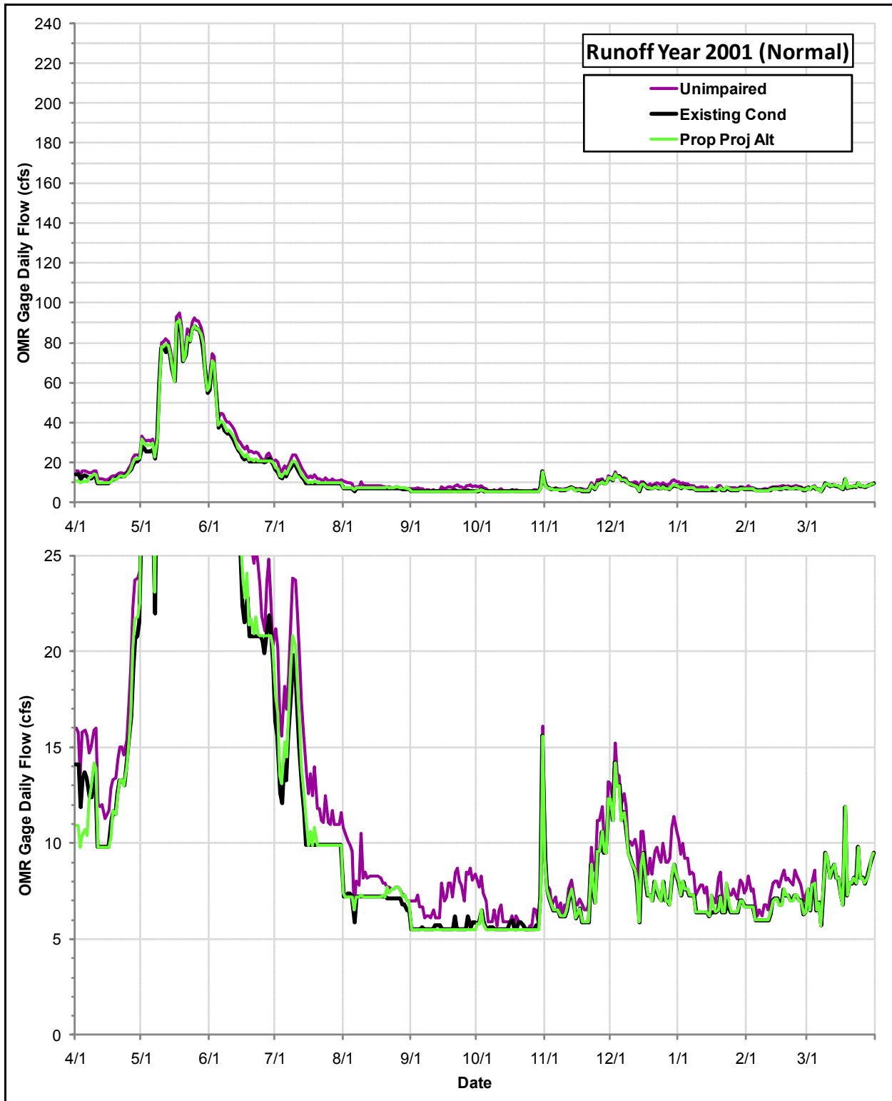
Daily Flows (cfs) at the OMR Gage under the Proposed Project Alternative, the Existing Condition and the Index of Unimpaired Conditions during Runoff Year 2001
