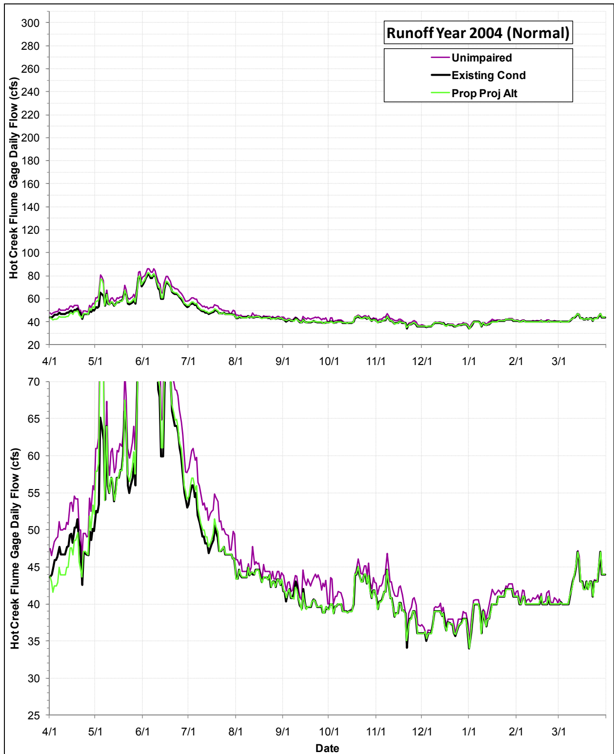
Daily Flows (cfs) at the USGS Hot Creek Flume Gage under the Proposed Project Alternative, the Existing Condition and the Index of Unimpaired Conditions during Runoff Year 2004
