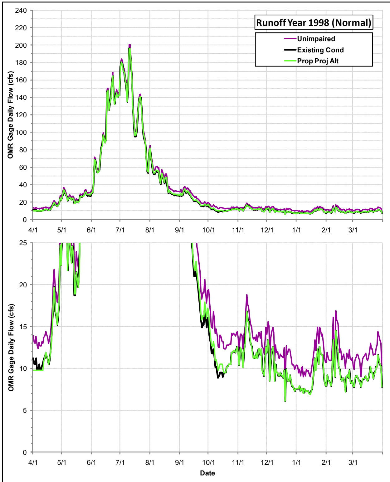
Daily Flows (cfs) at the OMR Gage under the Proposed Project Alternative, the Existing Condition and the Index of Unimpaired Conditions during Runoff Year 1998
