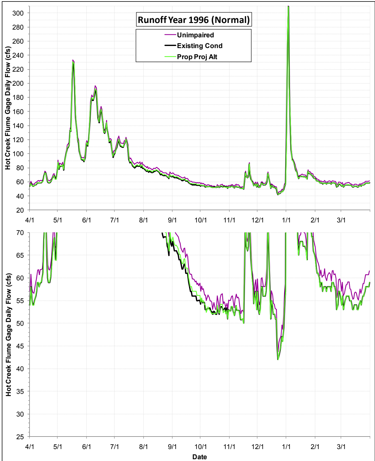
Daily Flows (cfs) at the USGS Hot Creek Flume Gage under the Proposed Project Alternative, the Existing Condition and the Index of Unimpaired Conditions during Runoff Year 1996
