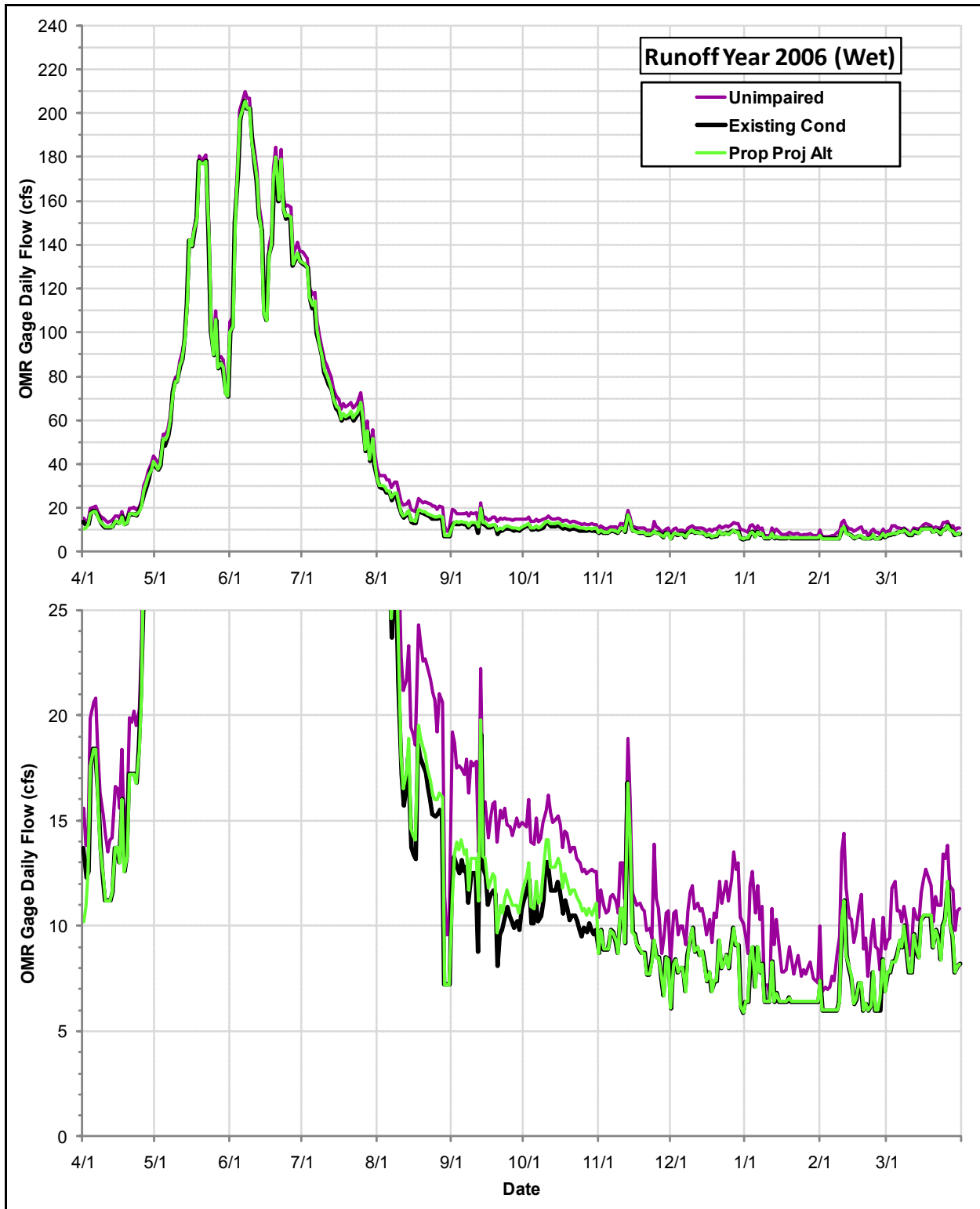
Daily Flows (cfs) at the OMR Gage under the Proposed Project Alternative, the Existing Condition and the Index of Unimpaired Conditions during Runoff Year 2006
