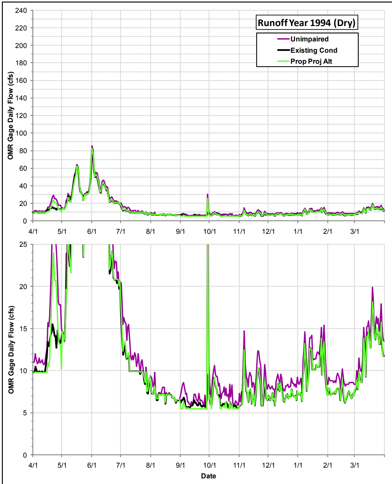
Daily Flows (cfs) at the OMR Gage under the Proposed Project Alternative, the Existing Condition and the Index of Unimpaired Conditions during Runoff Year 1994
