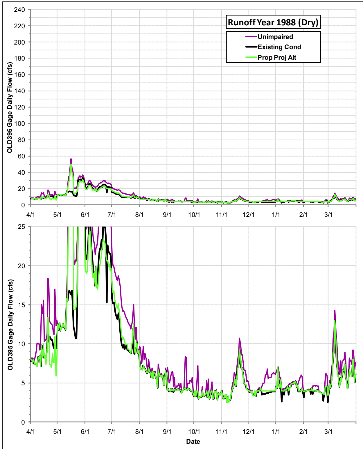
Daily Flows (cfs) at the OLD395 Gage under the Proposed Project Alternative, the Existing Condition and the Index of Unimpaired Conditions during Runoff Year 1988
