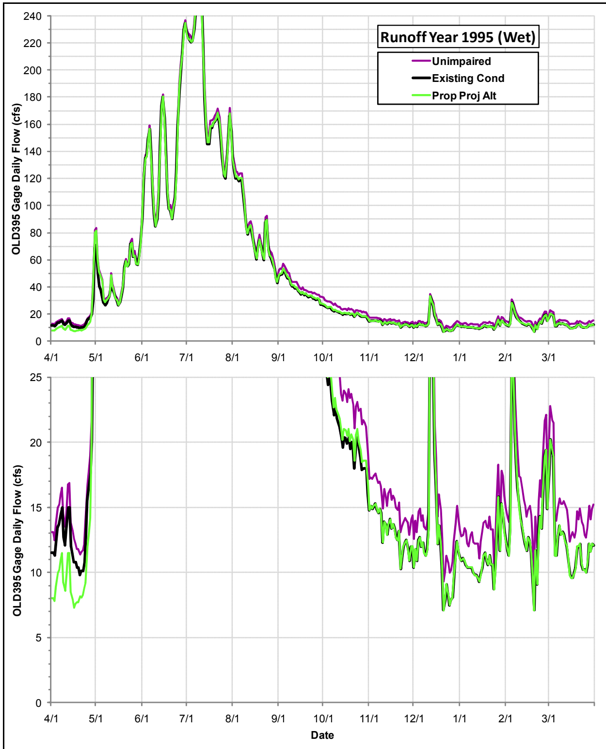
Daily Flows (cfs) at the OLD395 Gage under the Proposed Project Alternative, the Existing Condition and the Index of Unimpaired Conditions during Runoff Year 1995
