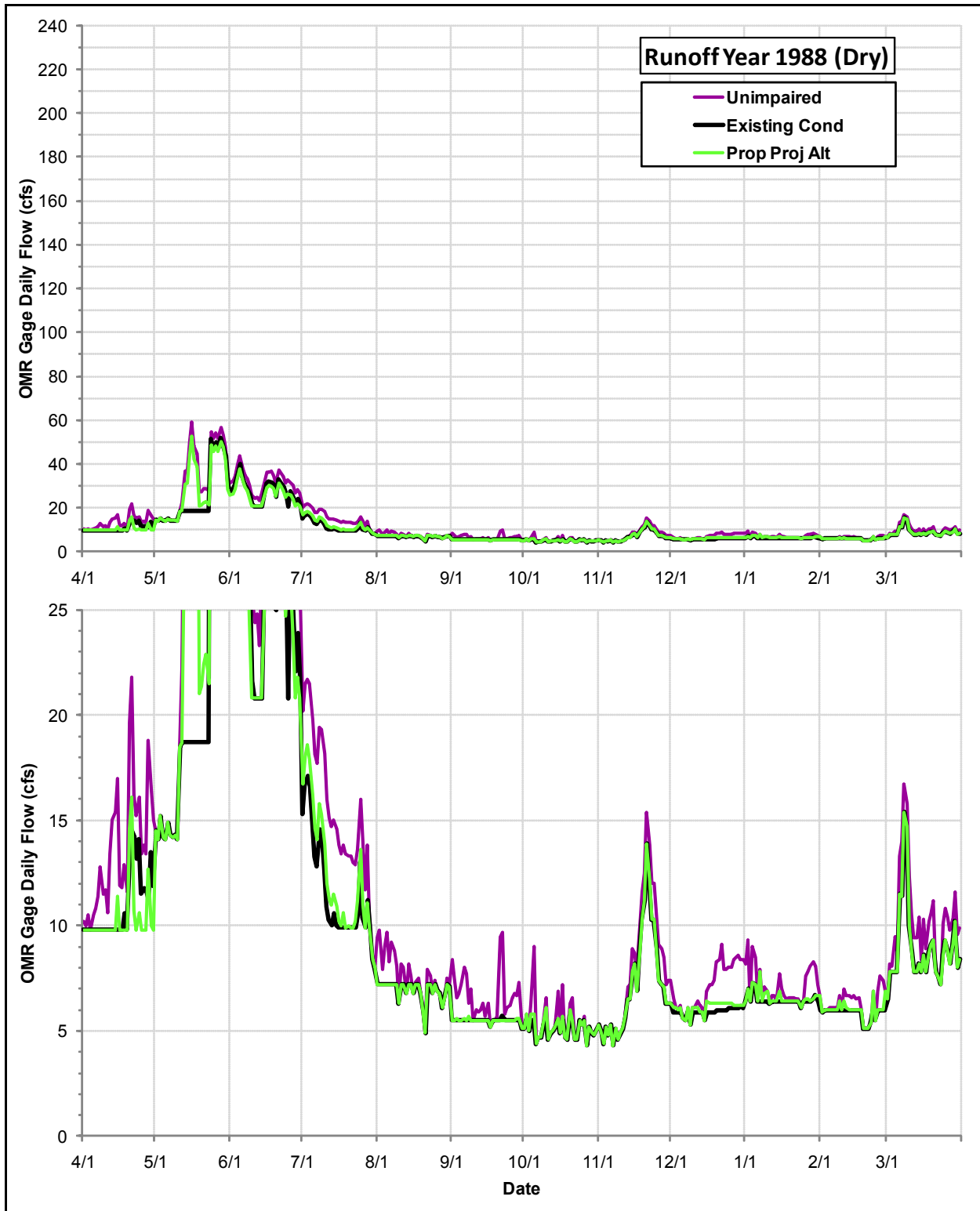
Daily Flows (cfs) at the OMR Gage under the Proposed Project Alternative, the Existing Condition and the Index of Unimpaired Conditions during Runoff Year 1988
