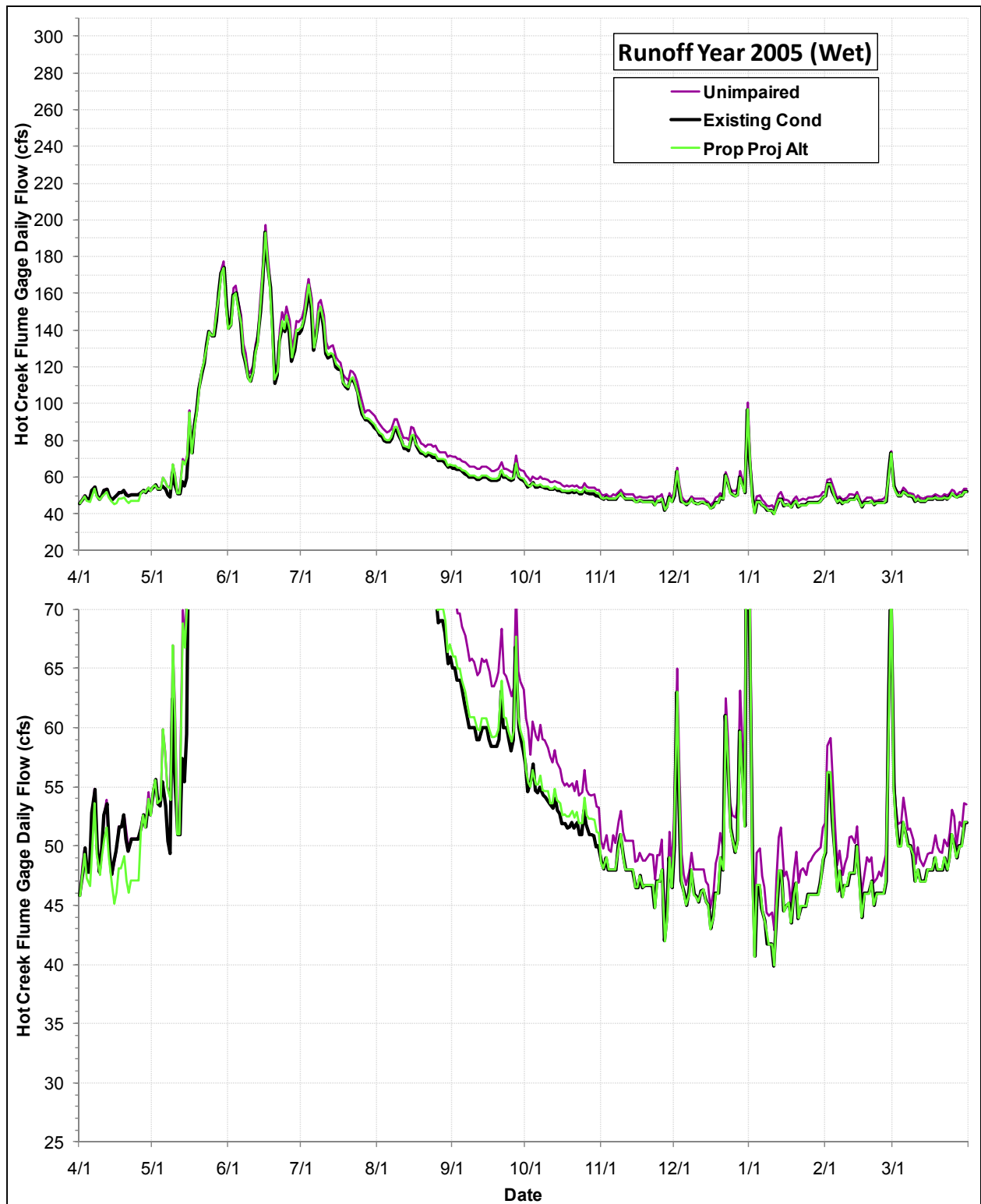
Daily Flows (cfs) at the USGS Hot Creek Flume Gage under the Proposed Project Alternative, the Existing Condition and the Index of Unimpaired Conditions during Runoff Year 2005
