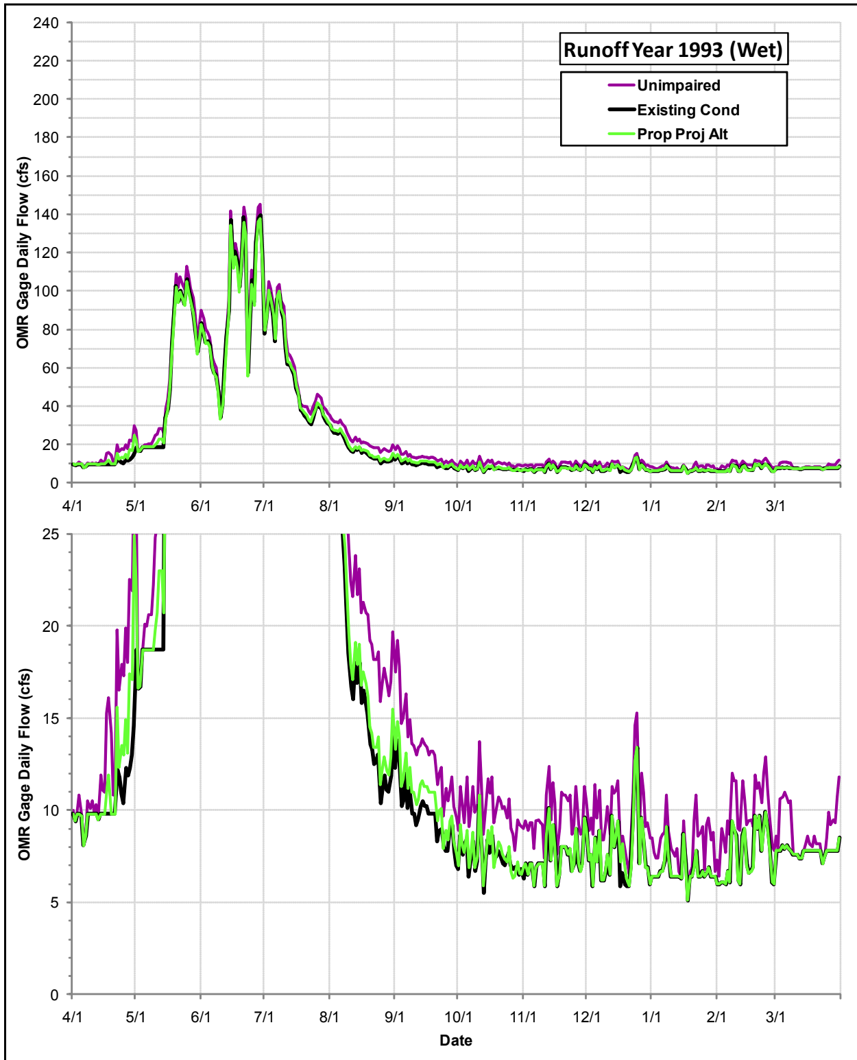
Daily Flows (cfs) at the OMR Gage under the Proposed Project Alternative, the Existing Condition and the Index of Unimpaired Conditions during Runoff Year 1993
