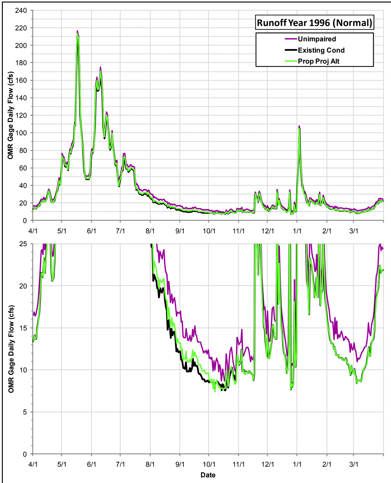
Daily Flows (cfs) at the OMR Gage under the Proposed Project Alternative, the Existing Condition and the Index of Unimpaired Conditions during Runoff Year 1996
