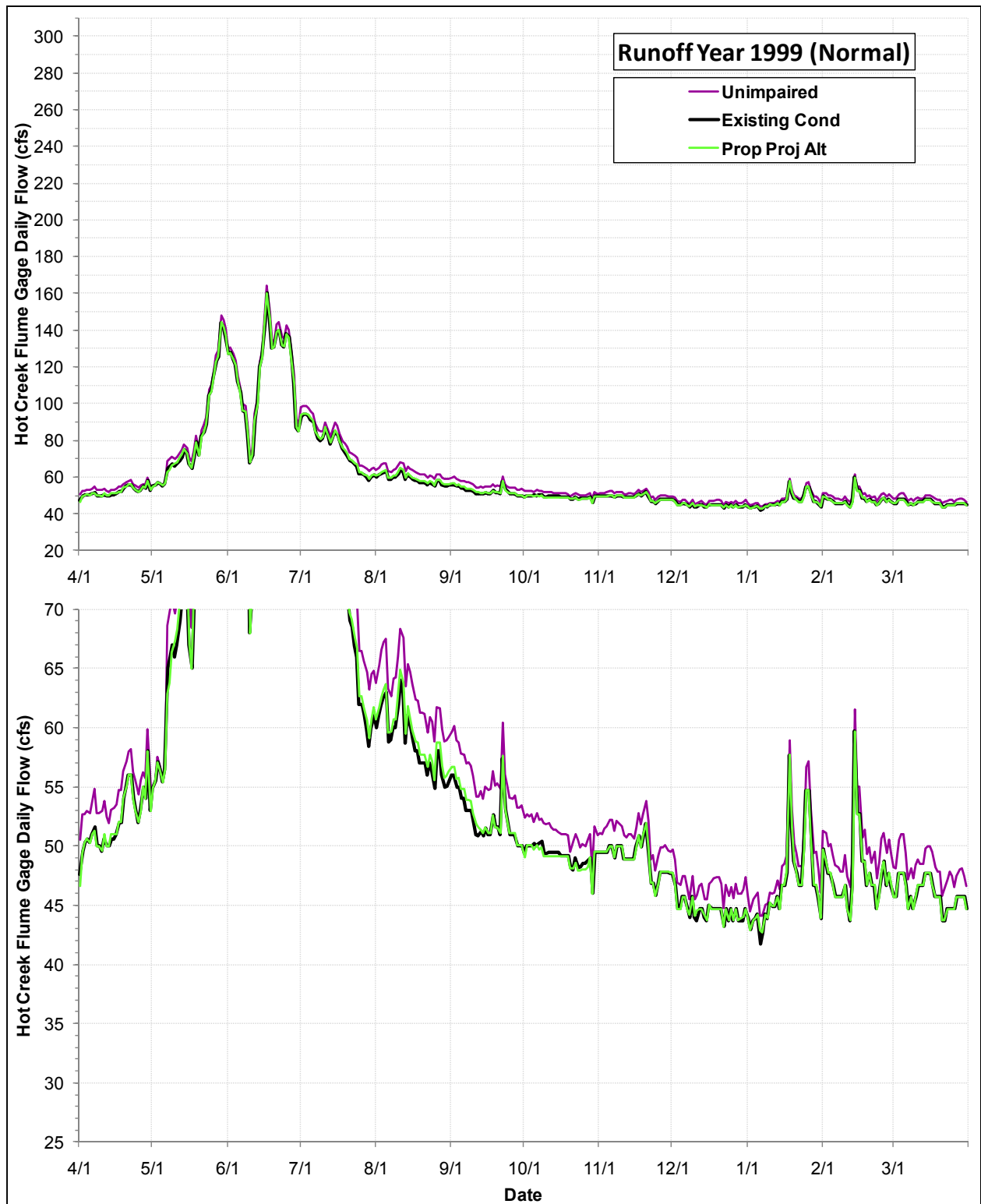
Daily Flows (cfs) at the USGS Hot Creek Flume Gage under the Proposed Project Alternative, the Existing Condition and the Index of Unimpaired Conditions during Runoff Year 1999
