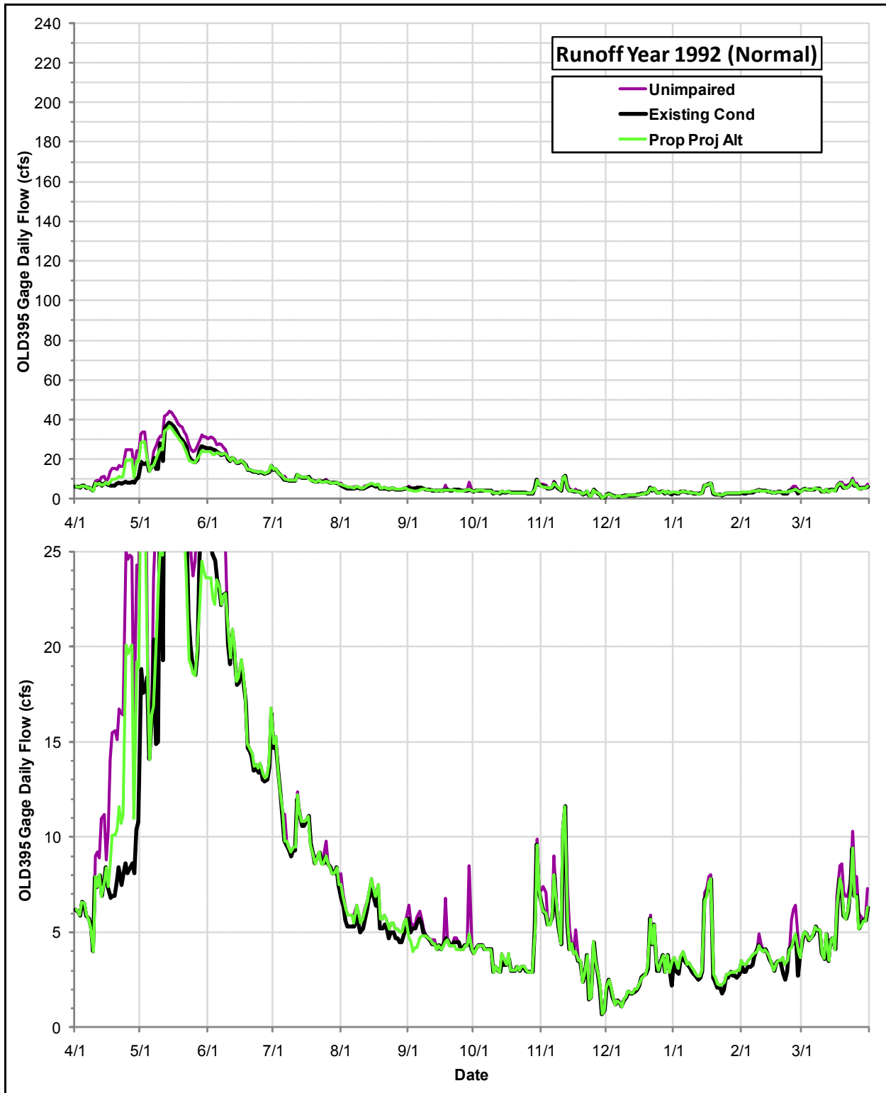
Daily Flows (cfs) at the OLD395 Gage under the Proposed Project Alternative, the Existing Condition and the Index Unimpaired Conditions during Runoff Year 1992
