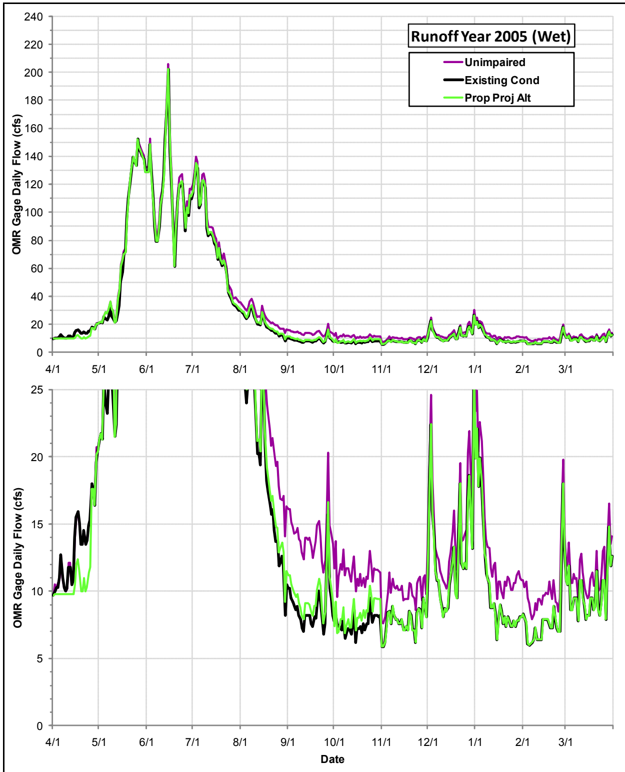
Daily Flows (cfs) at the OMR Gage under the Proposed Project Alternative, the Existing Condition and the Index of Unimpaired Conditions during Runoff Year 2005
