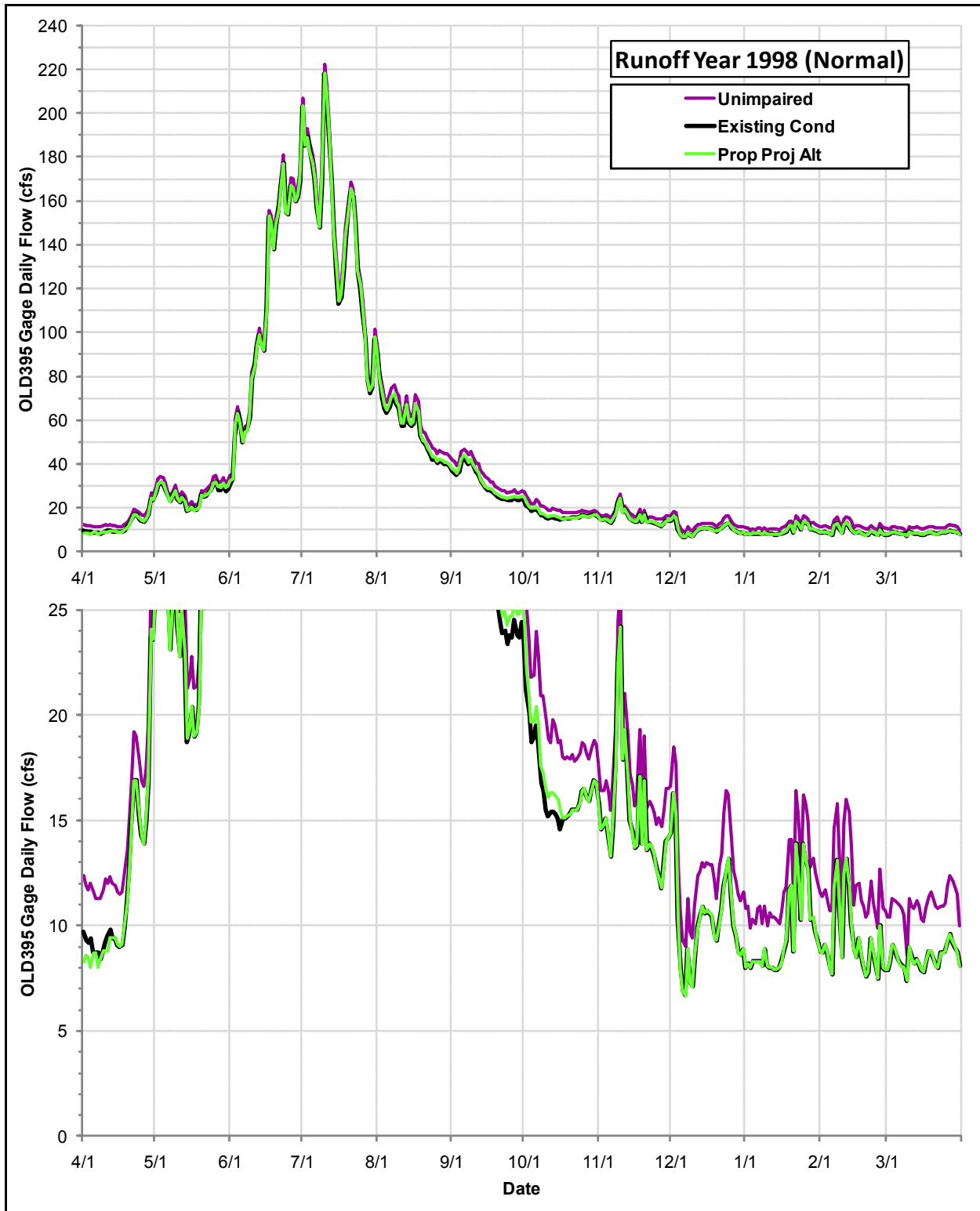
Daily Flows (cfs) at the OLD395 Gage under the Proposed Project Alternative, the Existing Condition and the Index of Unimpaired Conditions during Runoff Year 1998
