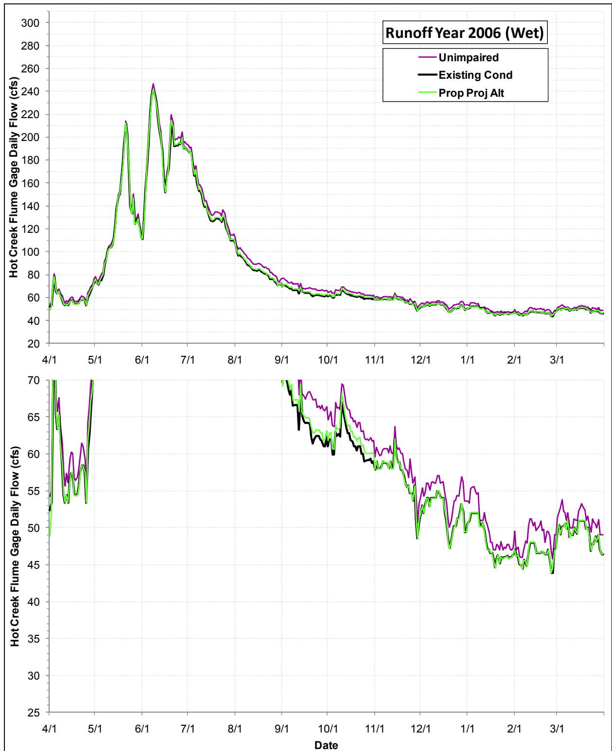
Daily Flows (cfs) at the USGS Hot Creek Flume Gage under the Proposed Project Alternative, the Existing Condition and the Index of Unimpaired Conditions during Runoff Year 2006
