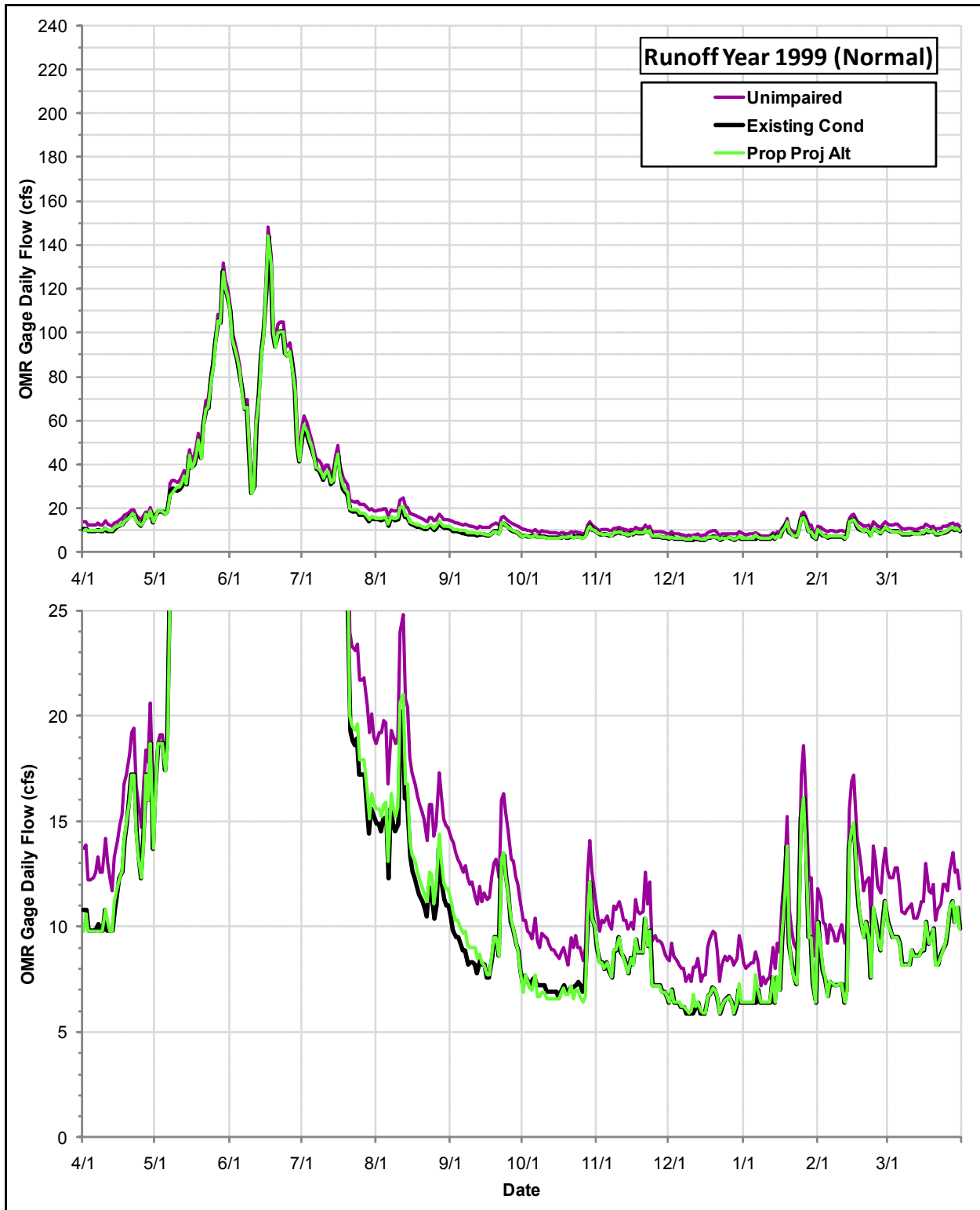
Daily Flows (cfs) at the OMR Gage under the Proposed Project Alternative, the Existing Condition and the Index of Unimpaired Conditions during Runoff Year 1999
