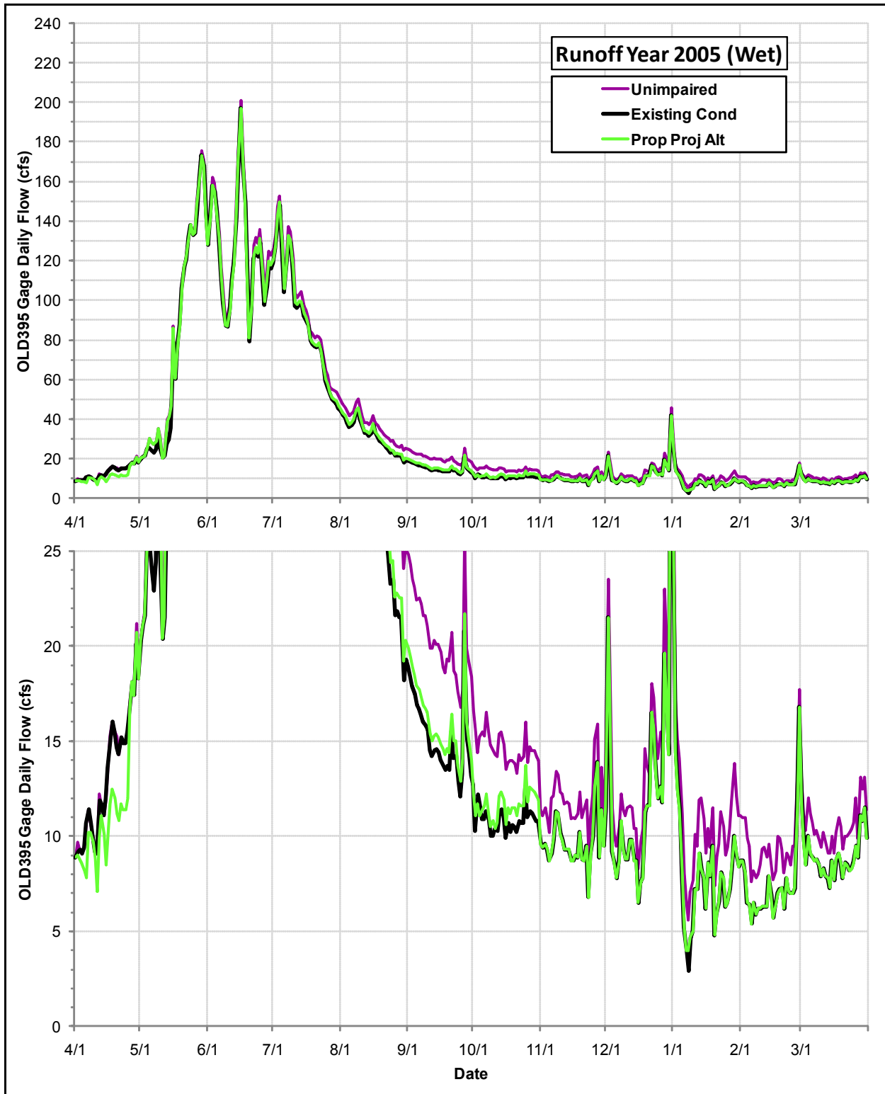
Daily Flows (cfs) at the OLD395 Gage under the Proposed Project Alternative, the Existing Condition and the Index of Unimpaired Conditions during Runoff Year 2005
