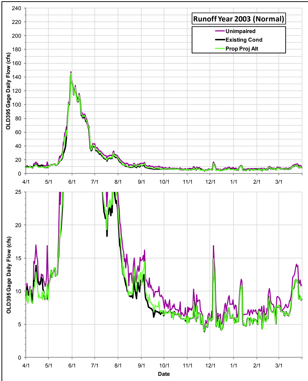
Daily Flows (cfs) at the OLD395 Gage under the Proposed Project Alternative, the Existing Condition and the Index of Unimpaired Conditions during Runoff Year 2003
