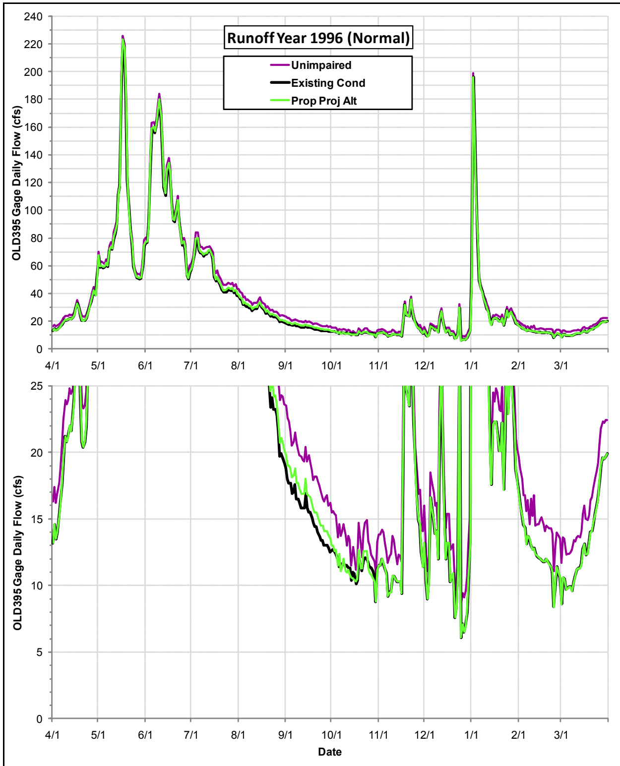
Daily Flows (cfs) at the OLD395 Gage under the Proposed Project Alternative, the Existing Condition and the Index of Unimpaired Conditions during Runoff Year 1996
