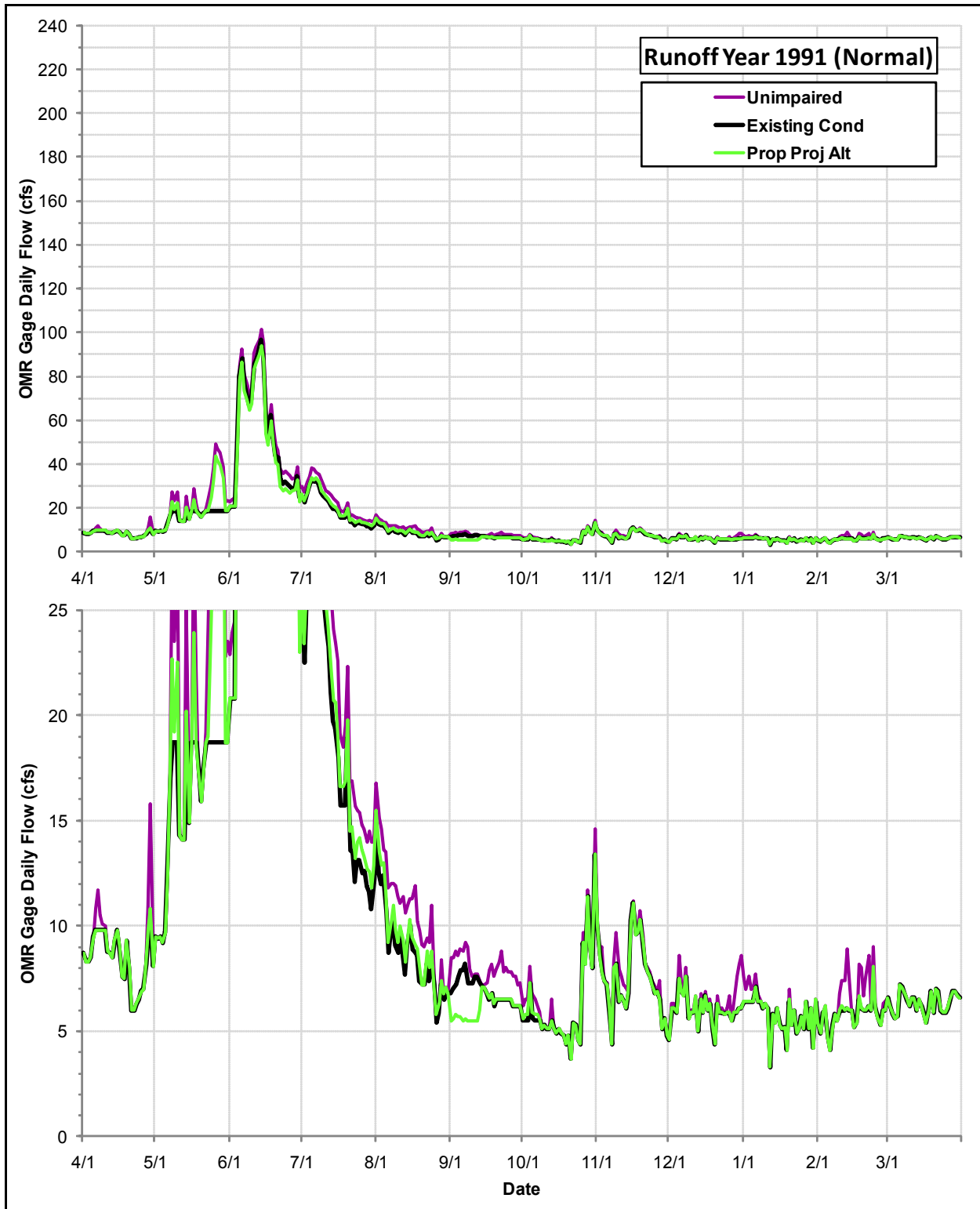
Daily Flows (cfs) at the OMR Gage under the Proposed Project Alternative, the Existing Condition and the Index of Unimpaired Conditions during Runoff Year 1991
