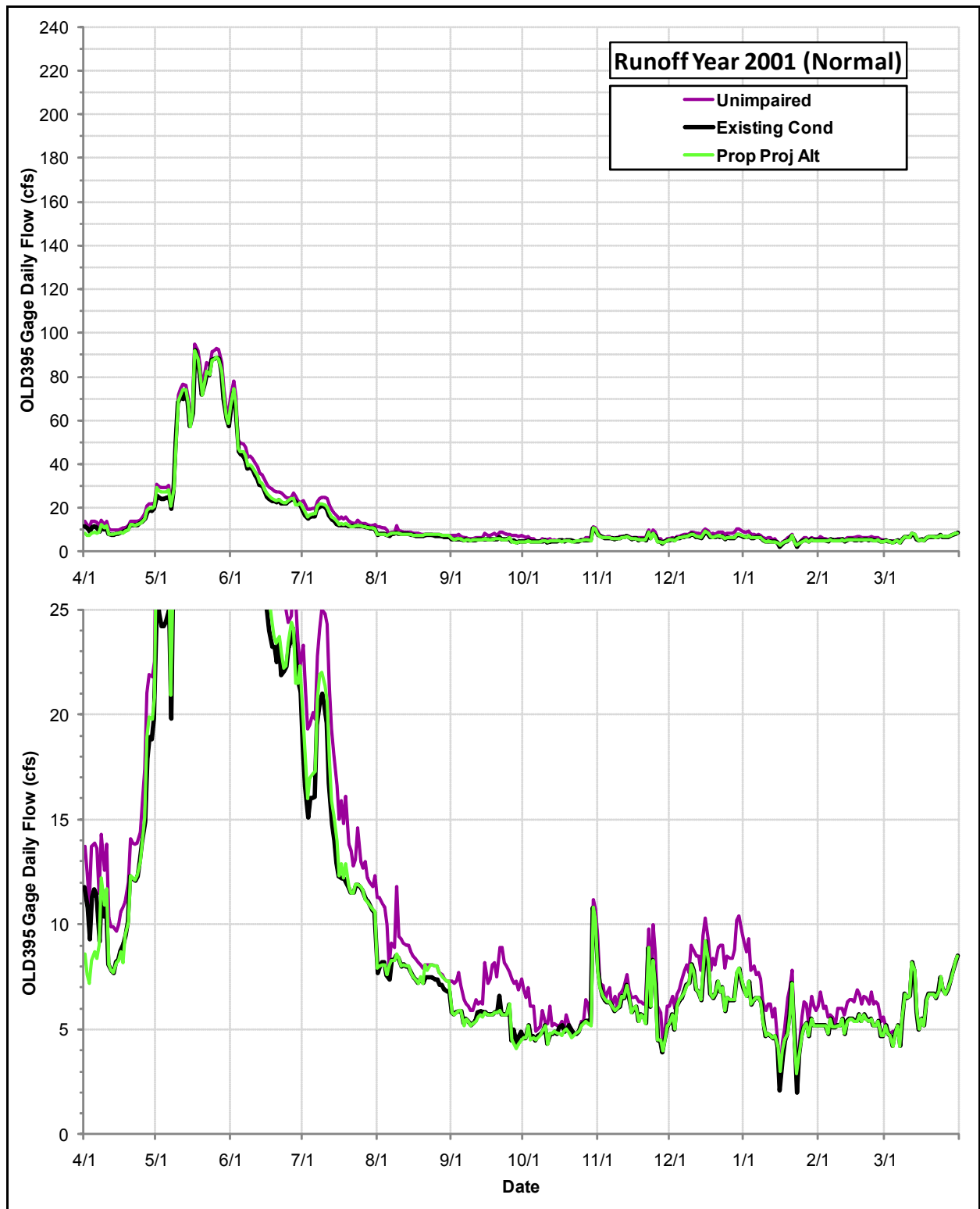
Daily Flows (cfs) at the OLD395 Gage under the Proposed Project Alternative, the Existing Condition and the Index of Unimpaired Conditions during Runoff Year 2001
