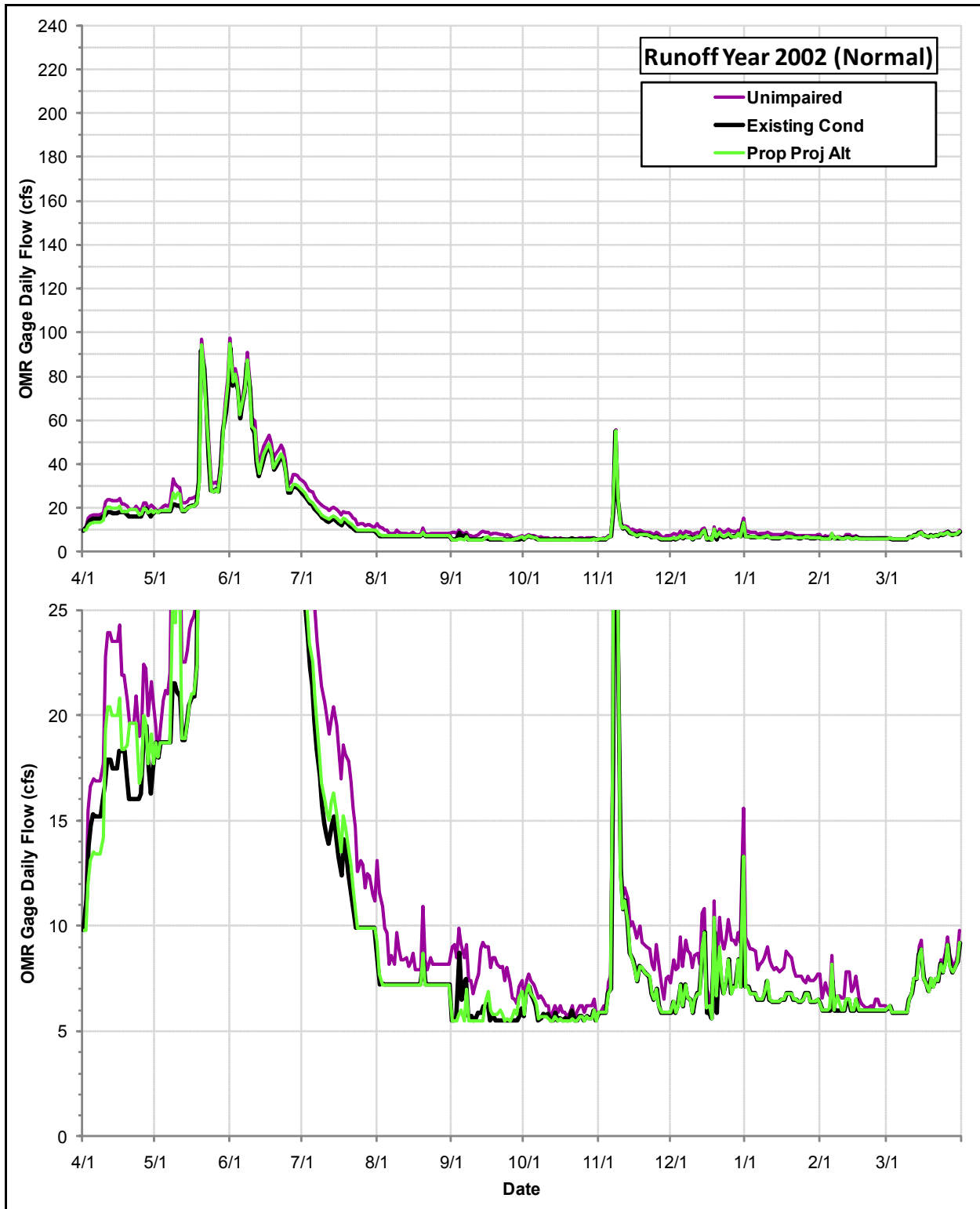
Daily Flows (cfs) at the OMR Gage under the Proposed Project Alternative, the Existing Condition and the Index of Unimpaired Conditions during Runoff Year 2002
