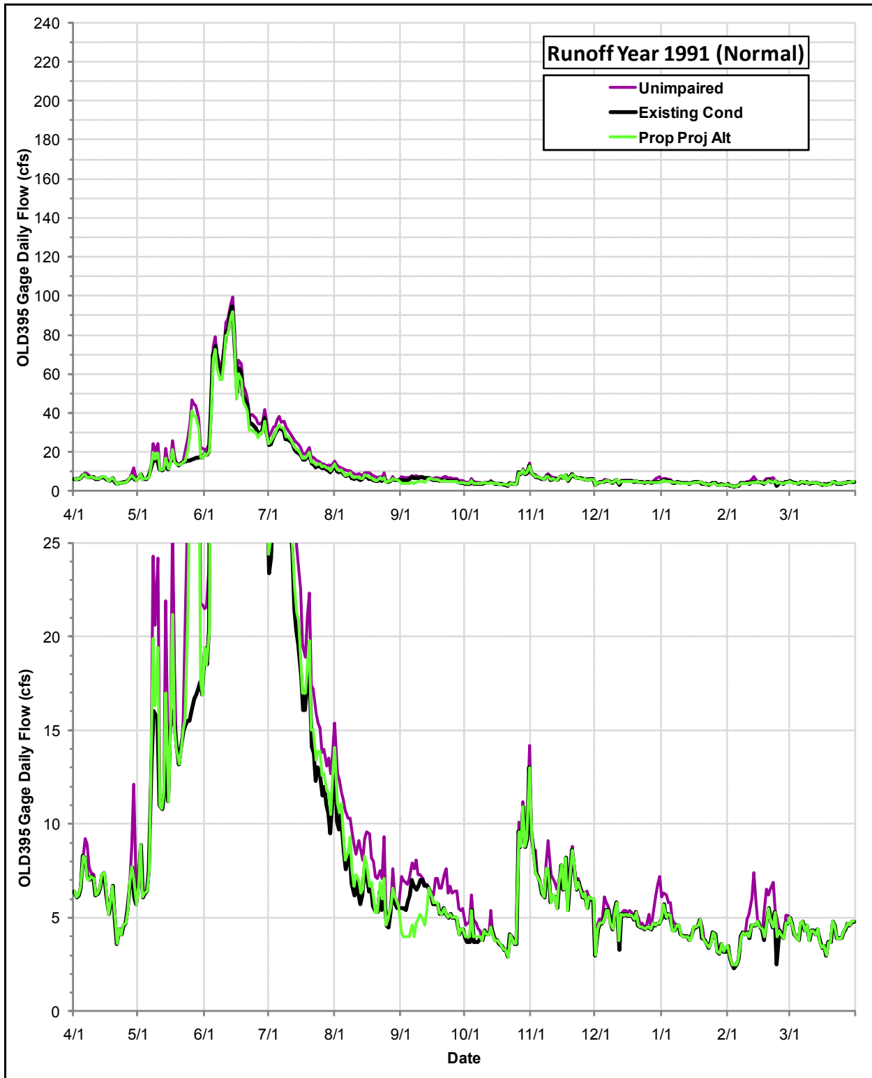
Daily Flows (cfs) at the OLD395 Gage under the Proposed Project Alternative, the Existing Condition and the Index of Unimpaired Conditions during Runoff Year 1991
