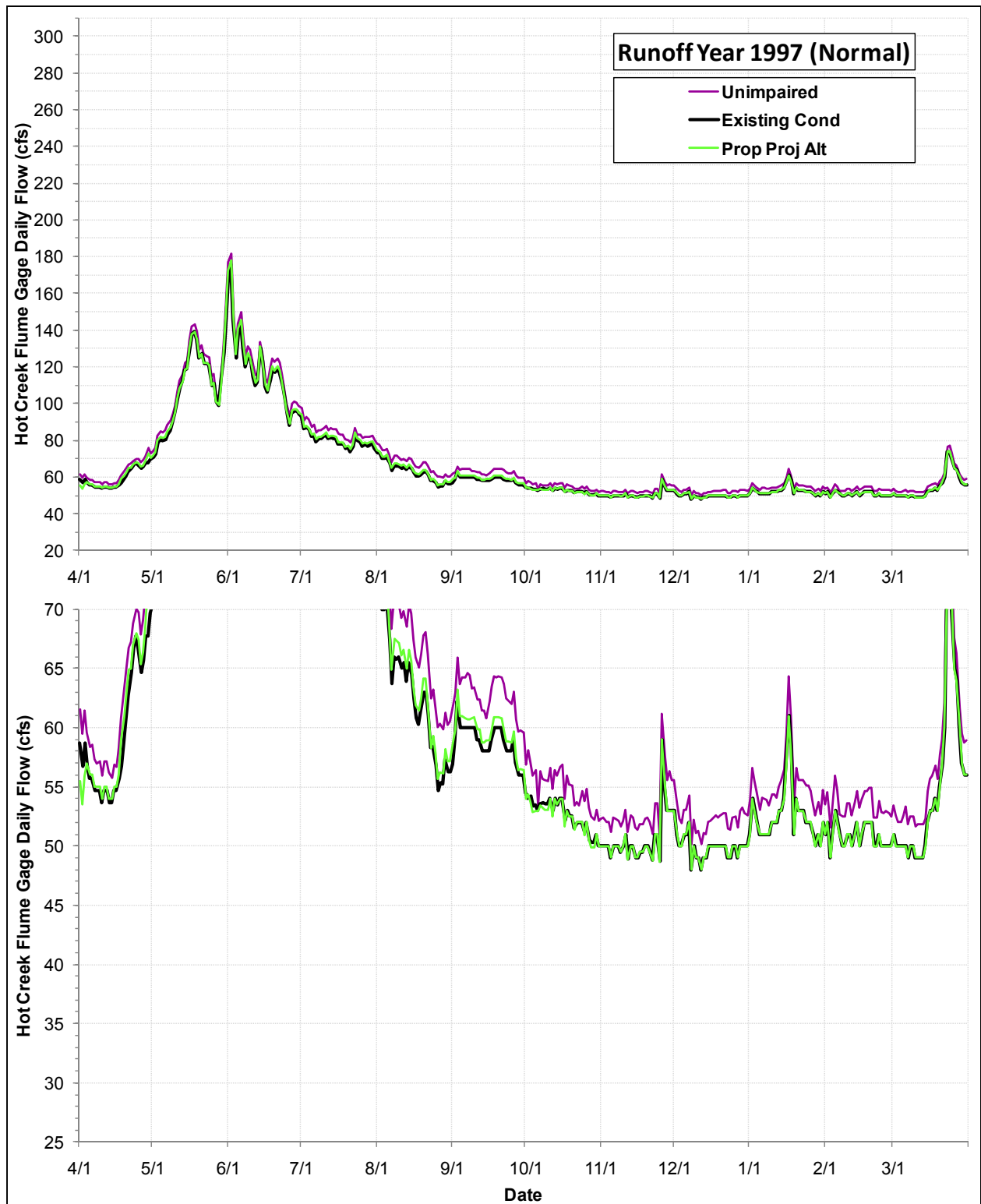
Daily Flows (cfs) at the USGS Hot Creek Flume Gage under the Proposed Project Alternative, the Existing Condition and the Index of Unimpaired Conditions during Runoff Year 1997
