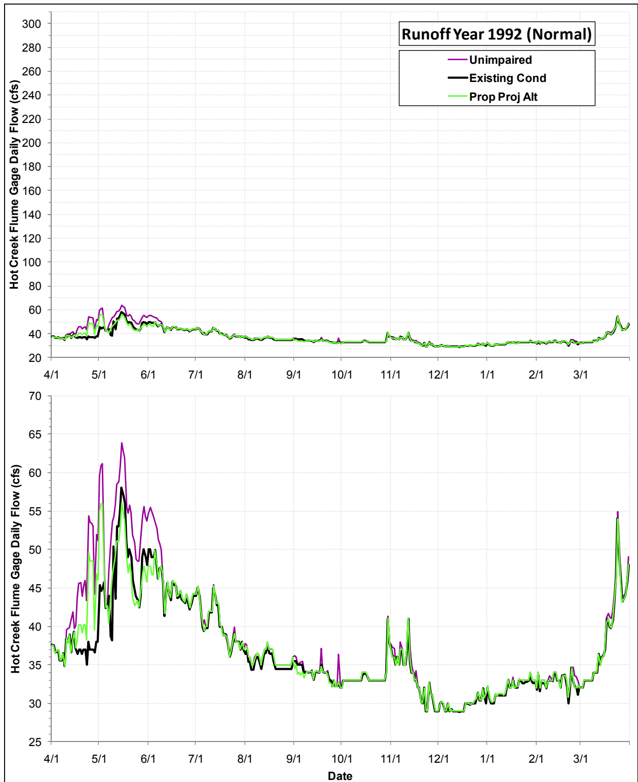
Daily Flows (cfs) at the USGS Hot Creek Flume Gage under the Proposed Project Alternative, the Existing Condition and the Index of Unimpaired Conditions during Runoff Year 1992
