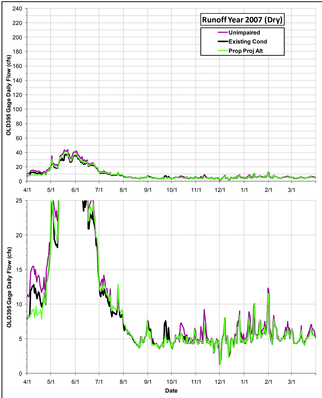
Daily Flows (cfs) at the OLD395 Gage under the Proposed Project Alternative, the Existing Condition and the Index of Unimpaired Conditions during Runoff Year 2007
