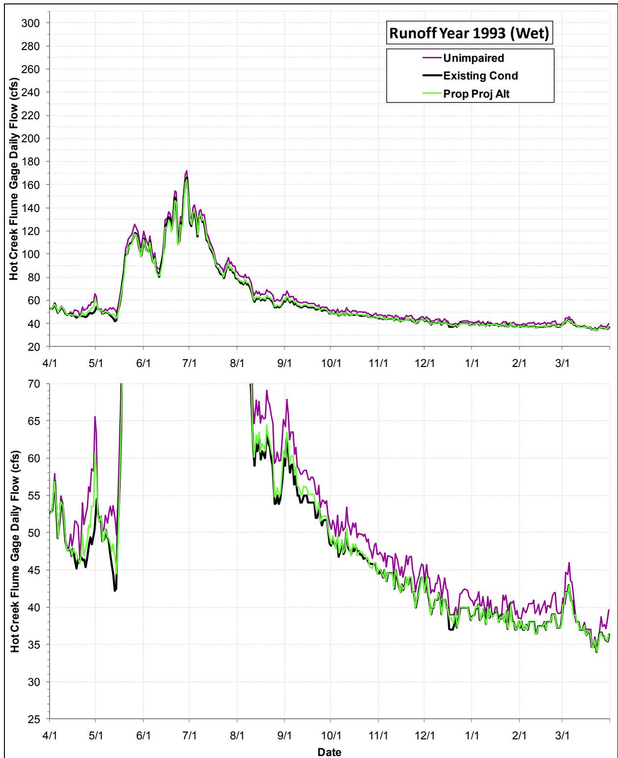
Daily Flows (cfs) at the USGS Hot Creek Flume Gage under the Proposed Project Alternative, the Existing Condition and the Index of Unimpaired Conditions during Runoff Year 1993
