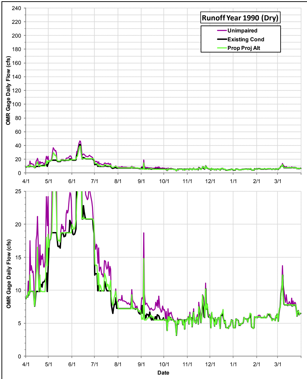
Daily Flows (cfs) at the OMR Gage under the Proposed Project Alternative, the Existing Condition and the Index of Unimpaired Conditions during Runoff Year 1990
