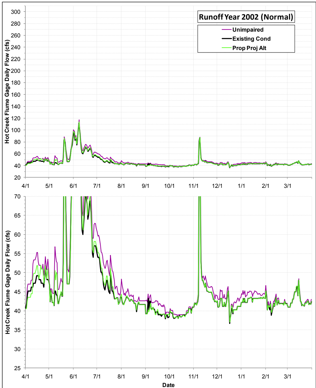
Daily Flows (cfs) at the USGS Hot Creek Flume Gage under the Proposed Project Alternative, the Existing Condition and the Index of Unimpaired Conditions during Runoff Year 2002
