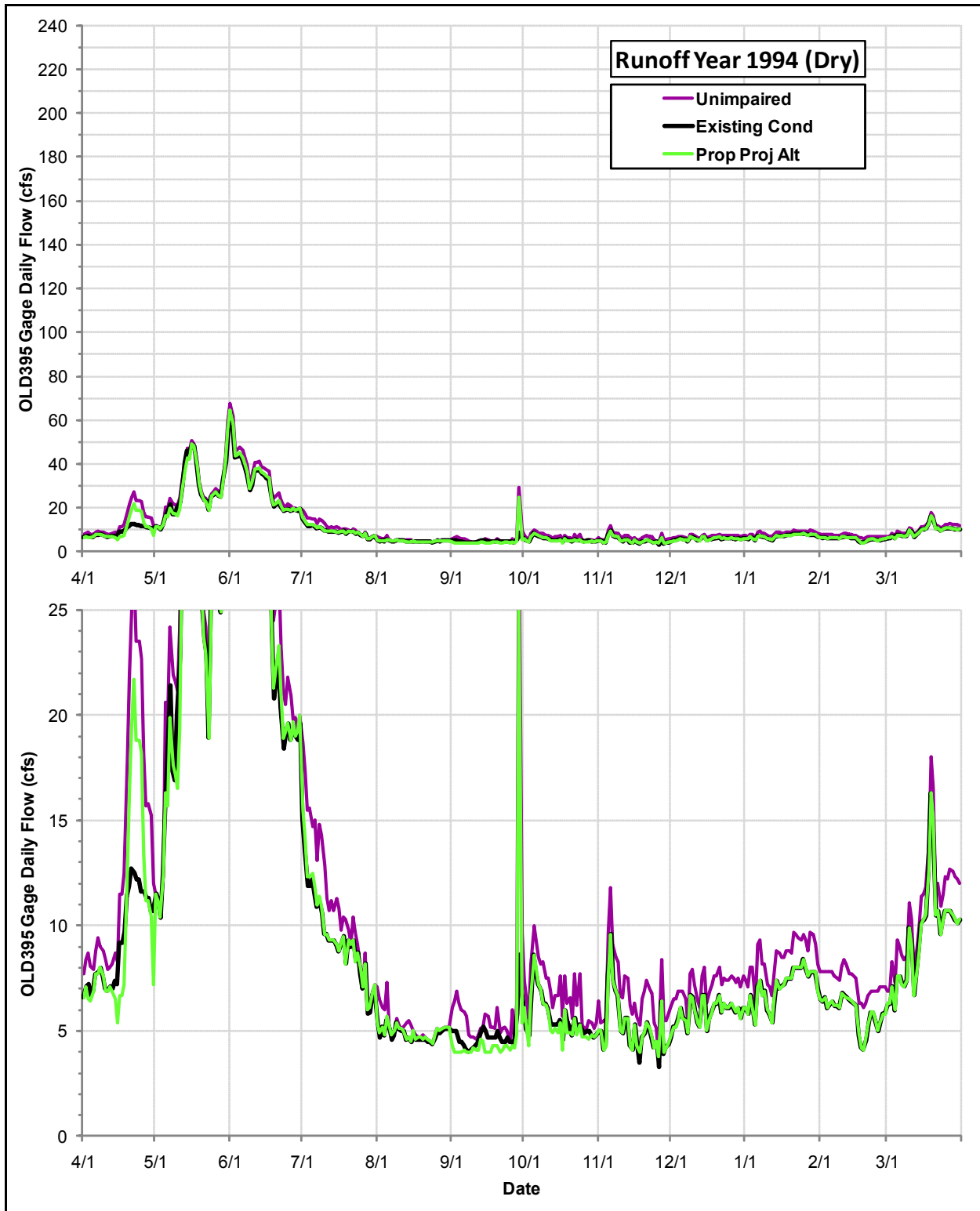
Daily Flows (cfs) at the OLD395 Gage under the Proposed Project Alternative, the Existing Condition and the Index of Unimpaired Conditions during Runoff Year 1994
