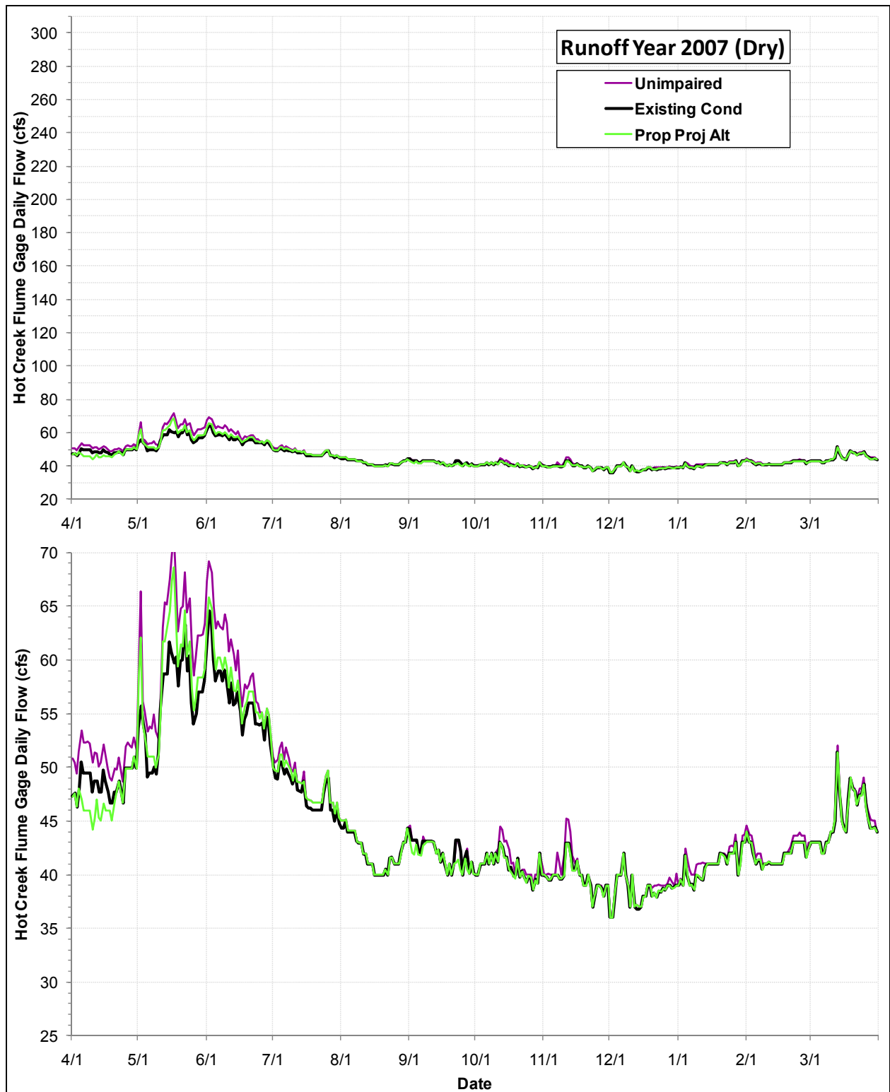
Daily Flows (cfs) at the USGS Hot Creek Flume Gage under the Proposed Project Alternative, the Existing Condition and the Index of Unimpaired Conditions during Runoff Year 2007
