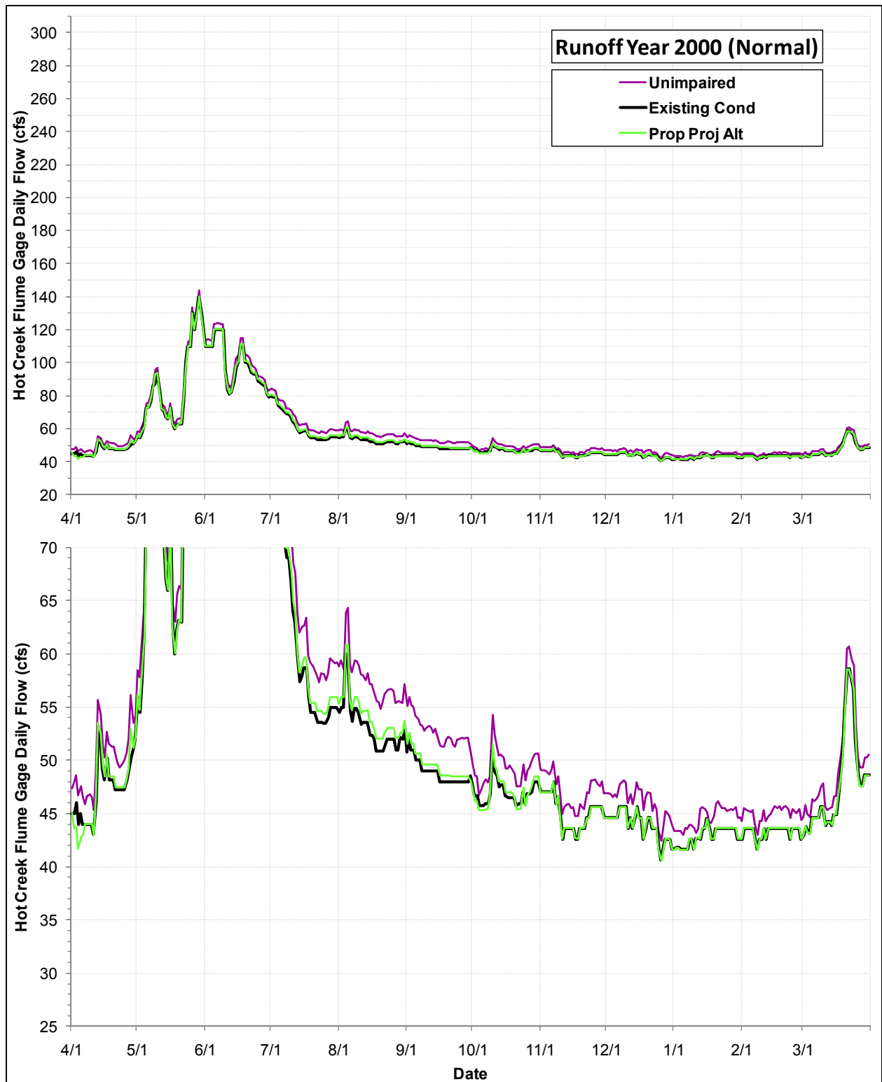
Daily Flows (cfs) at the USGS Hot Creek Flume Gage under the Proposed Project Alternative, the Existing Condition and the Index of Unimpaired Conditions during Runoff Year 2000
