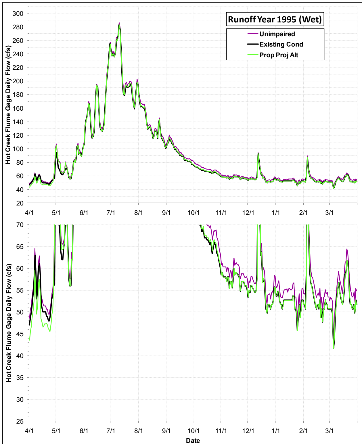
Daily Flows (cfs) at the USGS Hot Creek Flume Gage under the Proposed Project Alternative, the Existing Condition and the Index of Unimpaired Conditions during Runoff Year 1995
