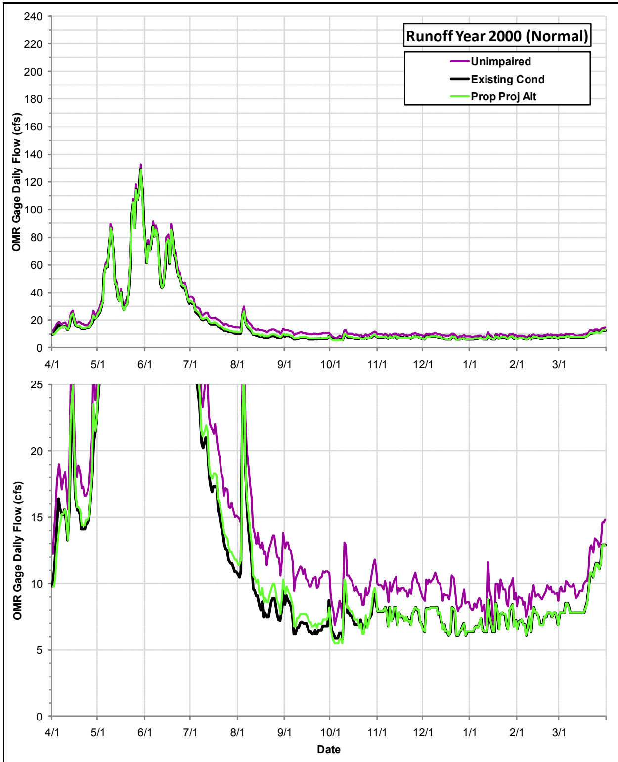
Daily Flows (cfs) at the OMR Gage under the Proposed Project Alternative, the Existing Condition and the Index of Unimpaired Conditions during Runoff Year 2000
