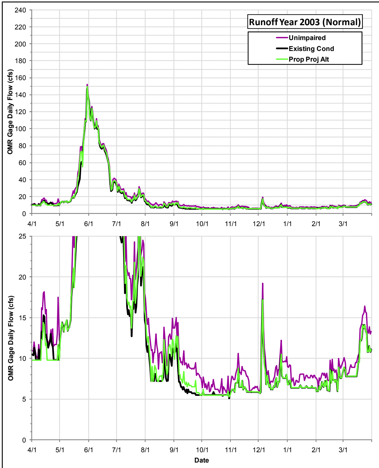
Daily Flows (cfs) at the OMR Gage under the Proposed Project Alternative, the Existing Condition and the Index of Unimpaired Conditions during Runoff Year 2003
