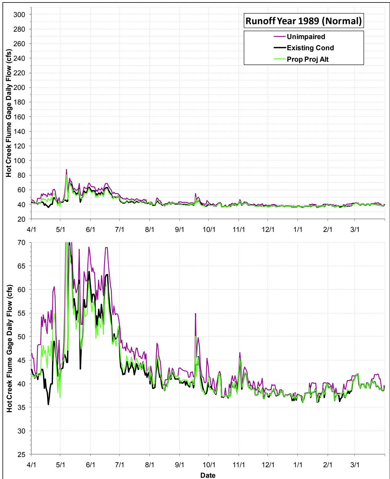
Daily Flows (cfs) at the USGS Hot Creek Flume Gage under the Proposed Project Alternative, the Existing Condition and the Index of Unimpaired Conditions during Runoff Year 1989
