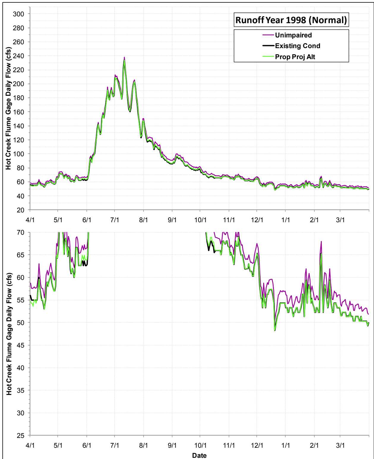
Daily Flows (cfs) at the USGS Hot Creek Flume Gage under the Proposed Project Alternative, the Existing Condition and the Index of Unimpaired Conditions during Runoff Year 1998
