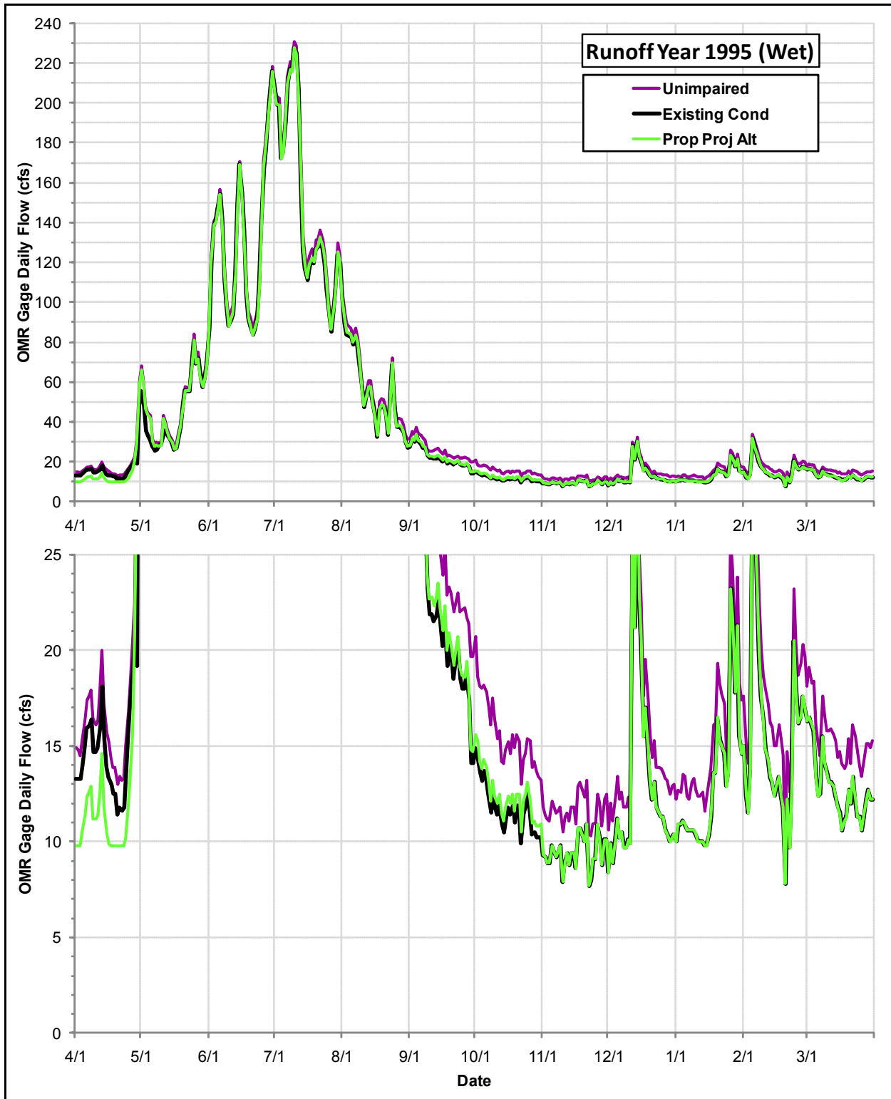
Daily Flows (cfs) at the OMR Gage under the Proposed Project Alternative, the Existing Condition and the Index of Unimpaired Conditions during Runoff Year 1995
