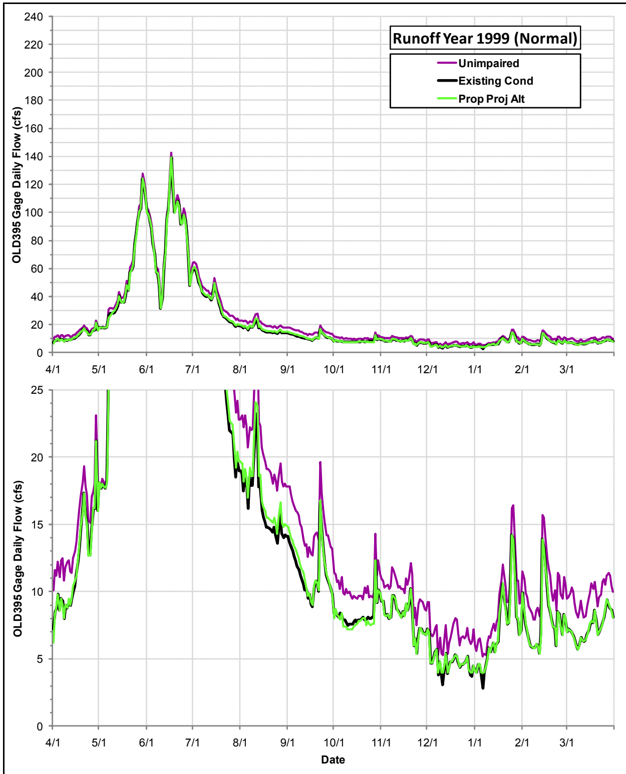
Daily Flows (cfs) at the OLD395 Gage under the Proposed Project Alternative, the Existing Condition and the Index of Unimpaired Conditions during Runoff Year 1999
