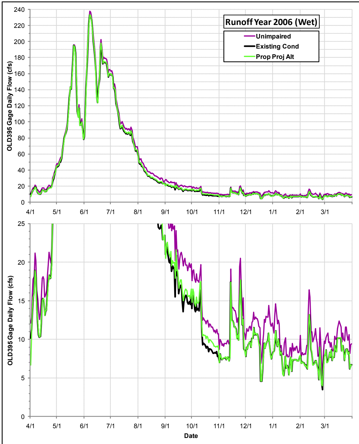
Daily Flows (cfs) at the OLD395 Gage under the Proposed Project Alternative, the Existing Condition and the Index of Unimpaired Conditions during Runoff Year 2006
